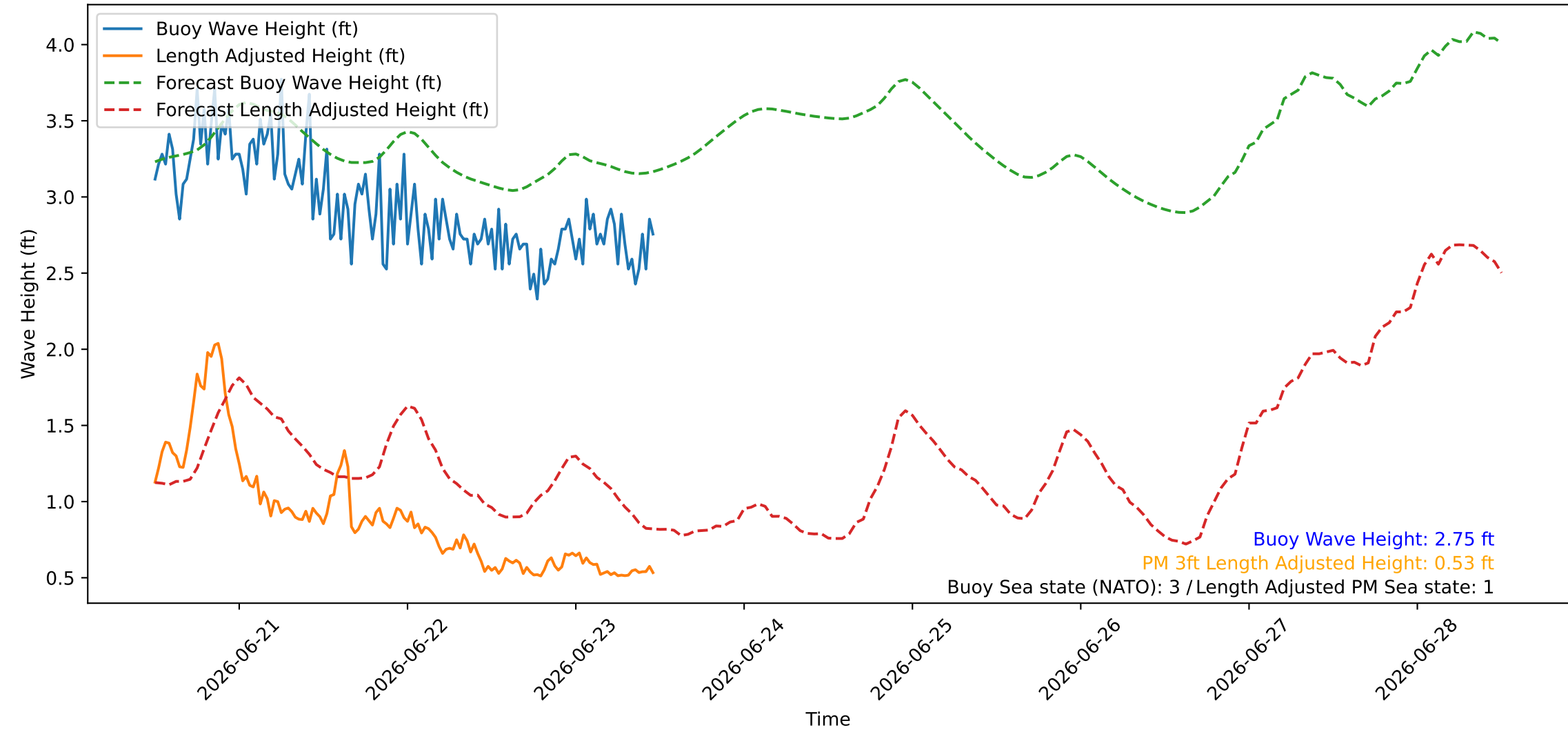
Wave Heights over Time for Red Beach at 2026-06-23 11:50:47
