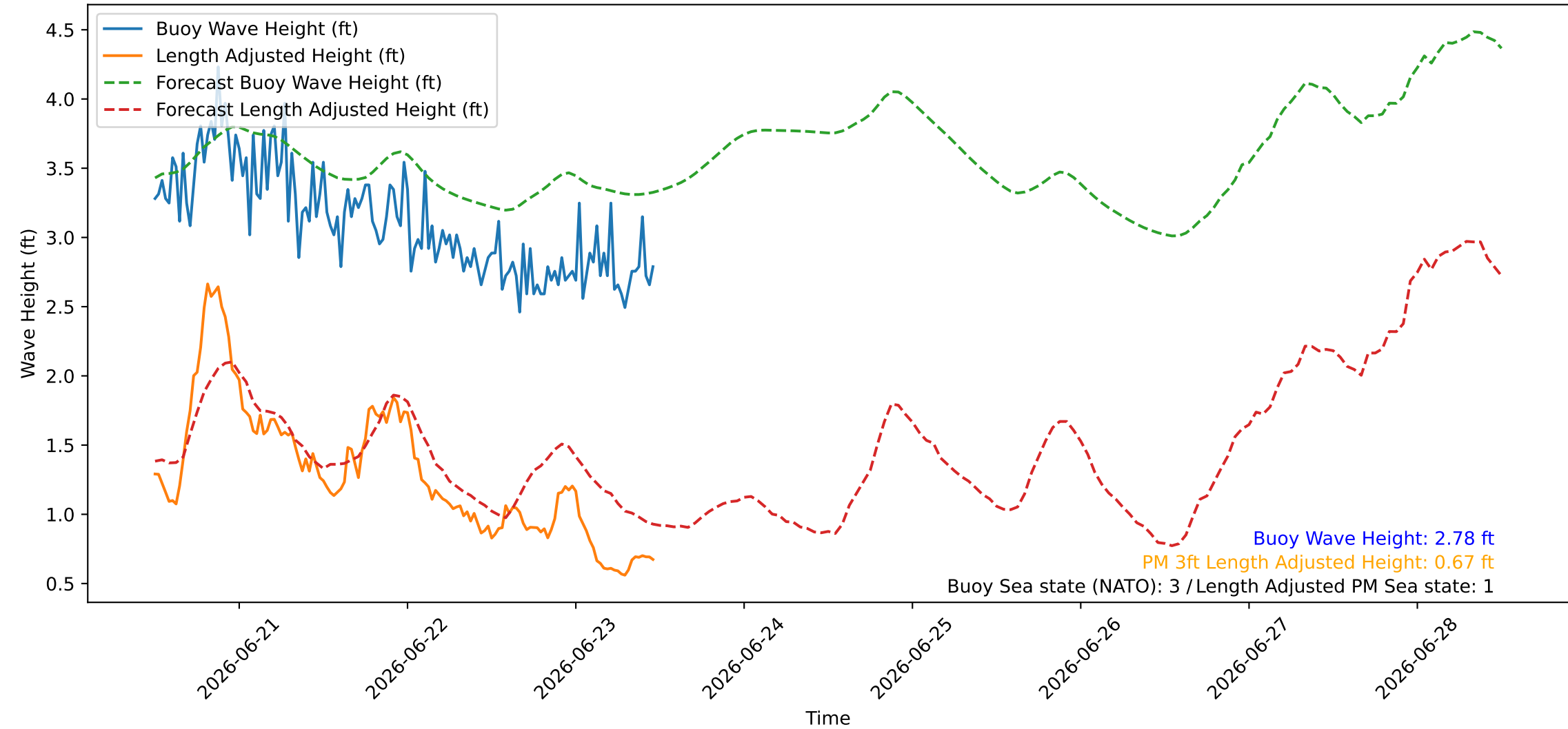
Wave Heights over Time for Green Beach at 2026-06-23 11:51:09
