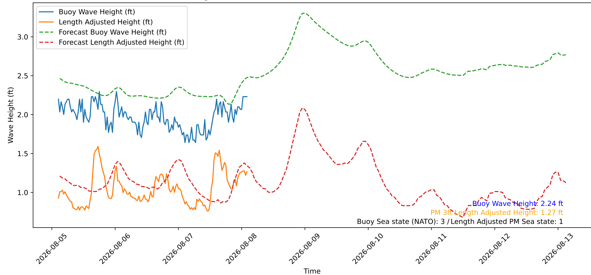
Wave Heights over Time for Oceanside Harbor at 2026-08-08 02:30:26
