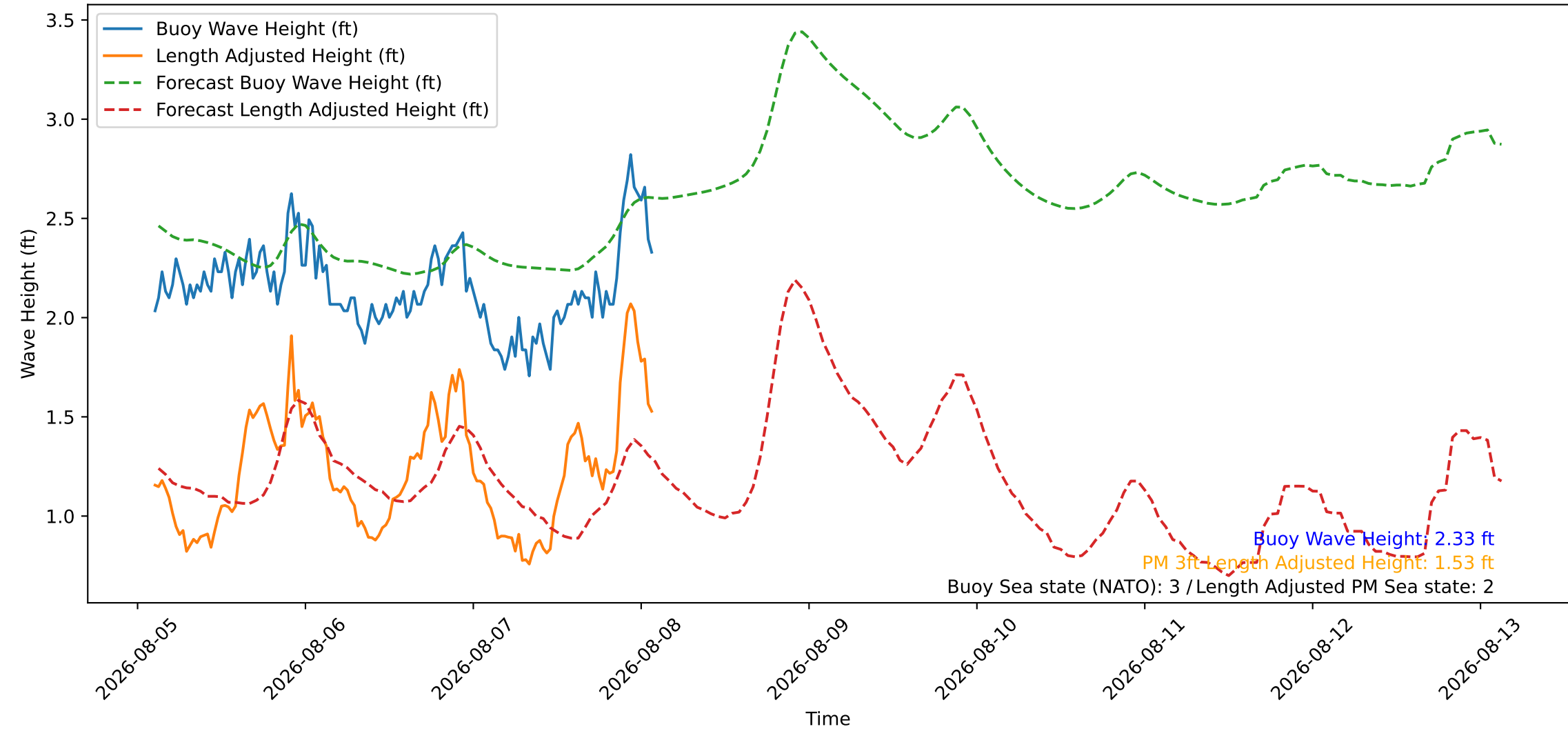
Wave Heights over Time for Green Beach at 2026-08-08 02:31:07
