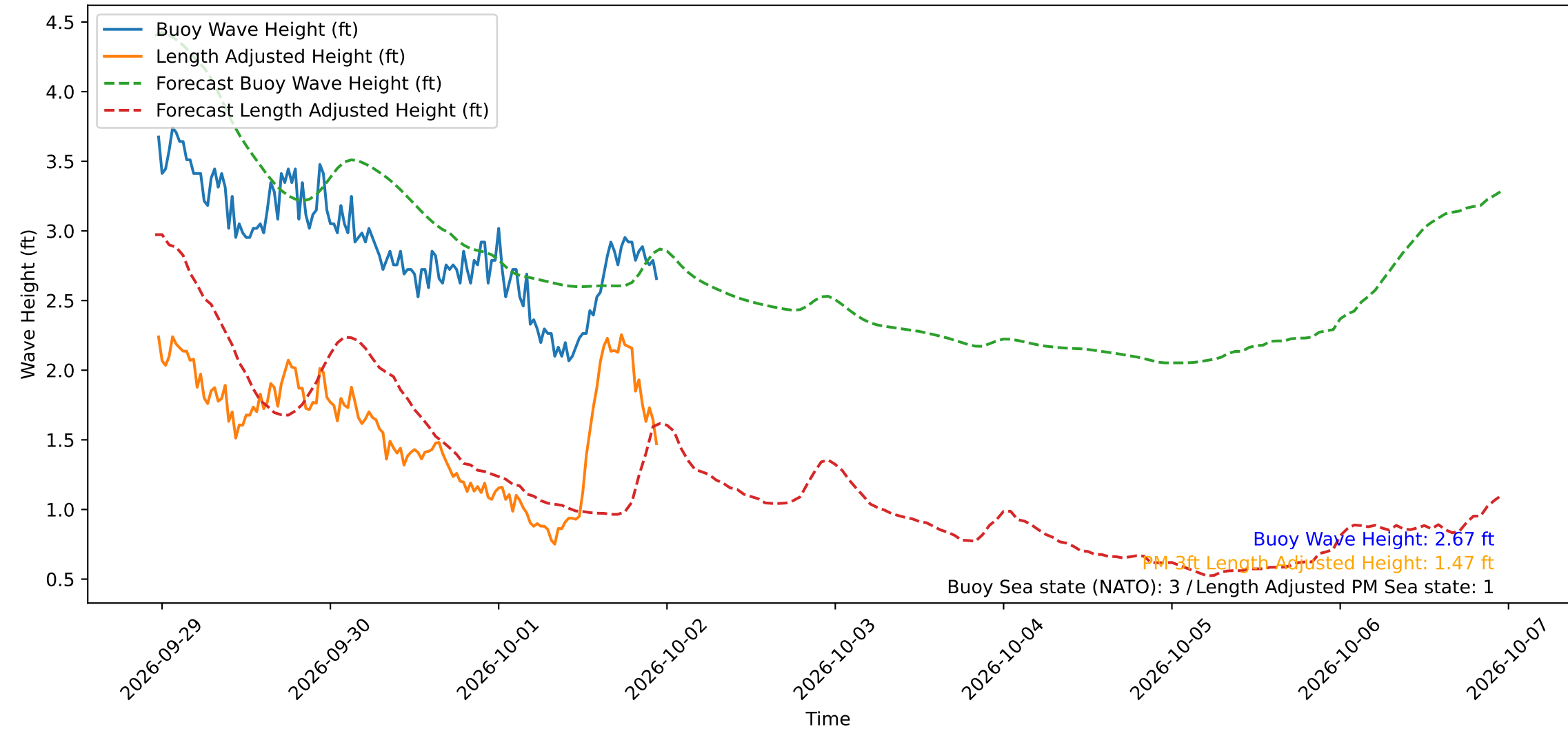
Wave Heights over Time for Red Beach at 2026-10-01 23:20:50
