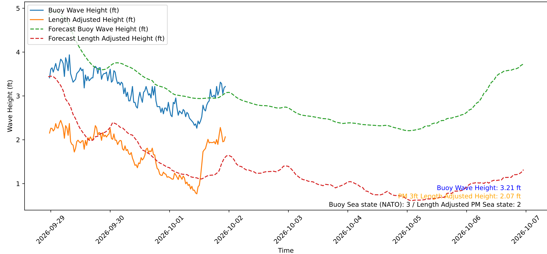
Wave Heights over Time for Oceanside Harbor at 2026-10-01 23:20:29
