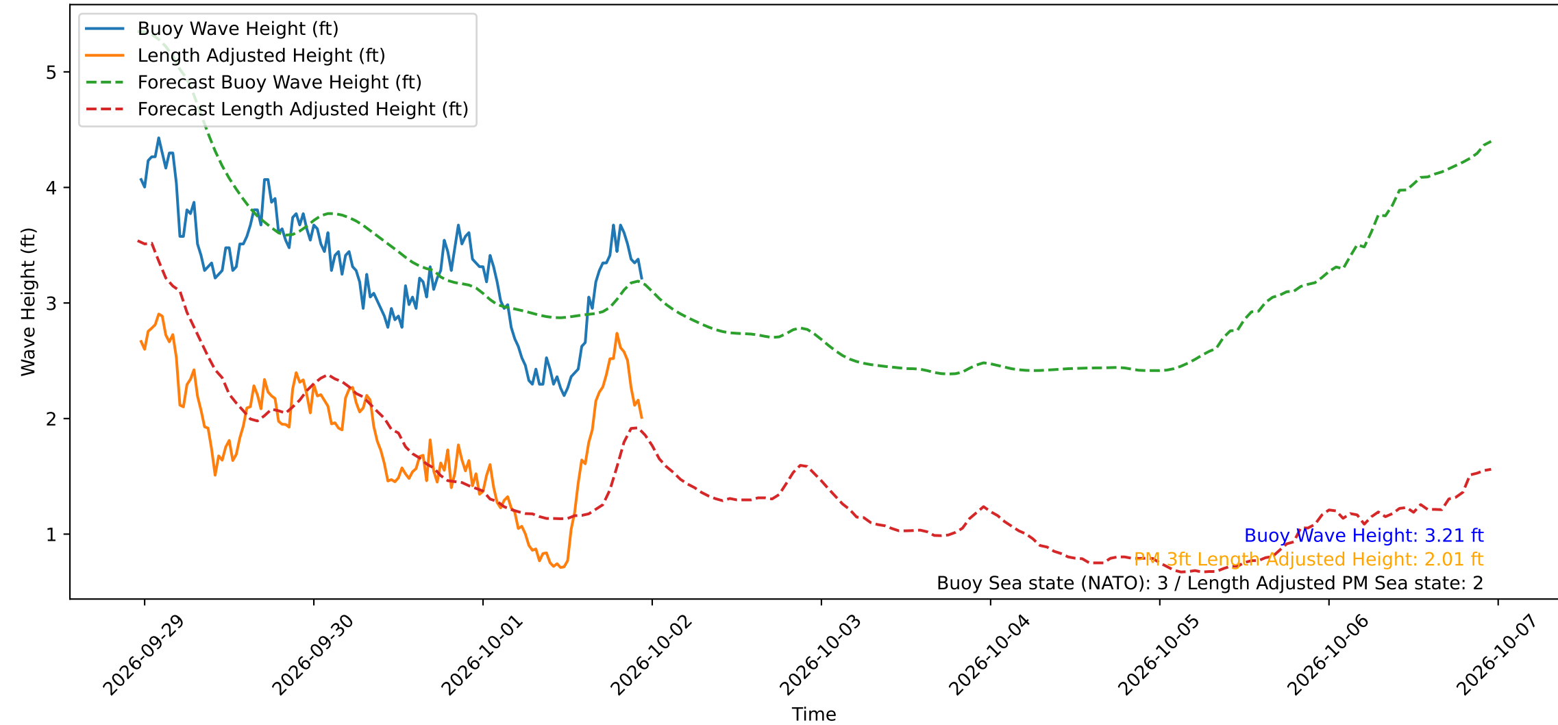
Wave Heights over Time for Green Beach at 2026-10-01 23:21:14
