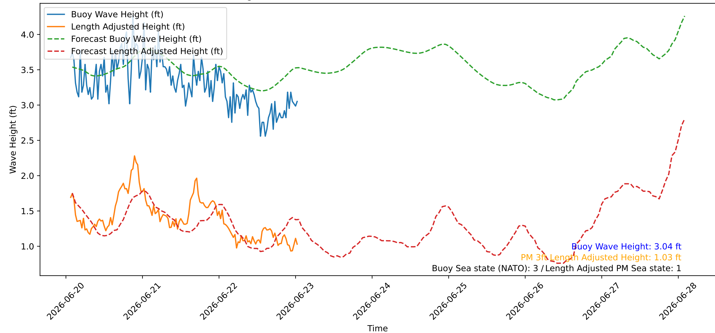
Wave Heights over Time for Oceanside Harbor at 2026-06-23 01:30:26
