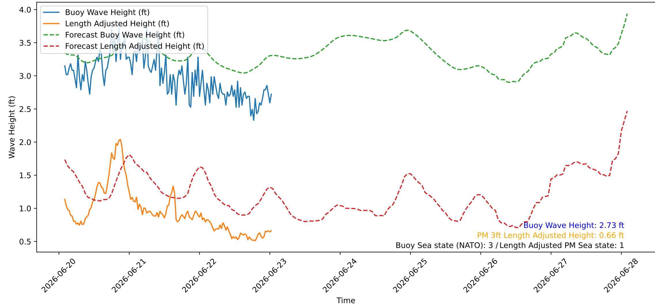
Wave Heights over Time for Red Beach at 2026-06-23 01:30:44
