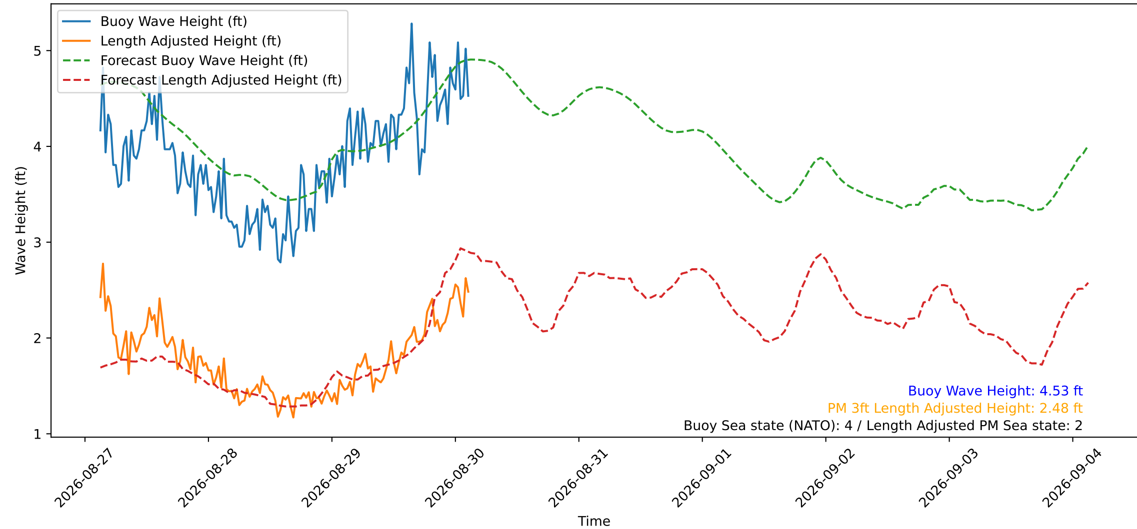
Wave Heights over Time for Oceanside Harbor at 2026-08-30 03:10:29
