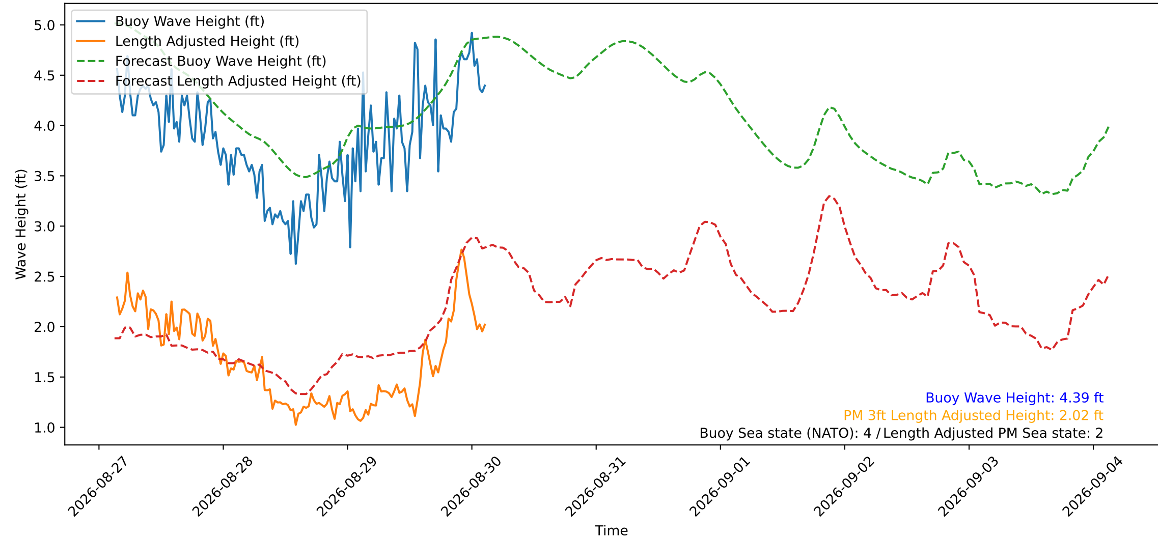
Wave Heights over Time for Green Beach at 2026-08-30 03:11:11
