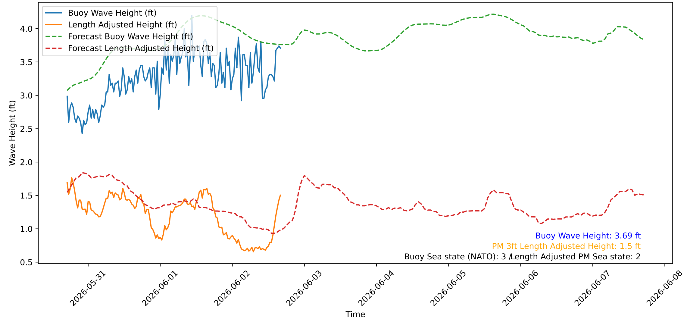
Wave Heights over Time for Red Beach at 2026-06-02 16:50:47
