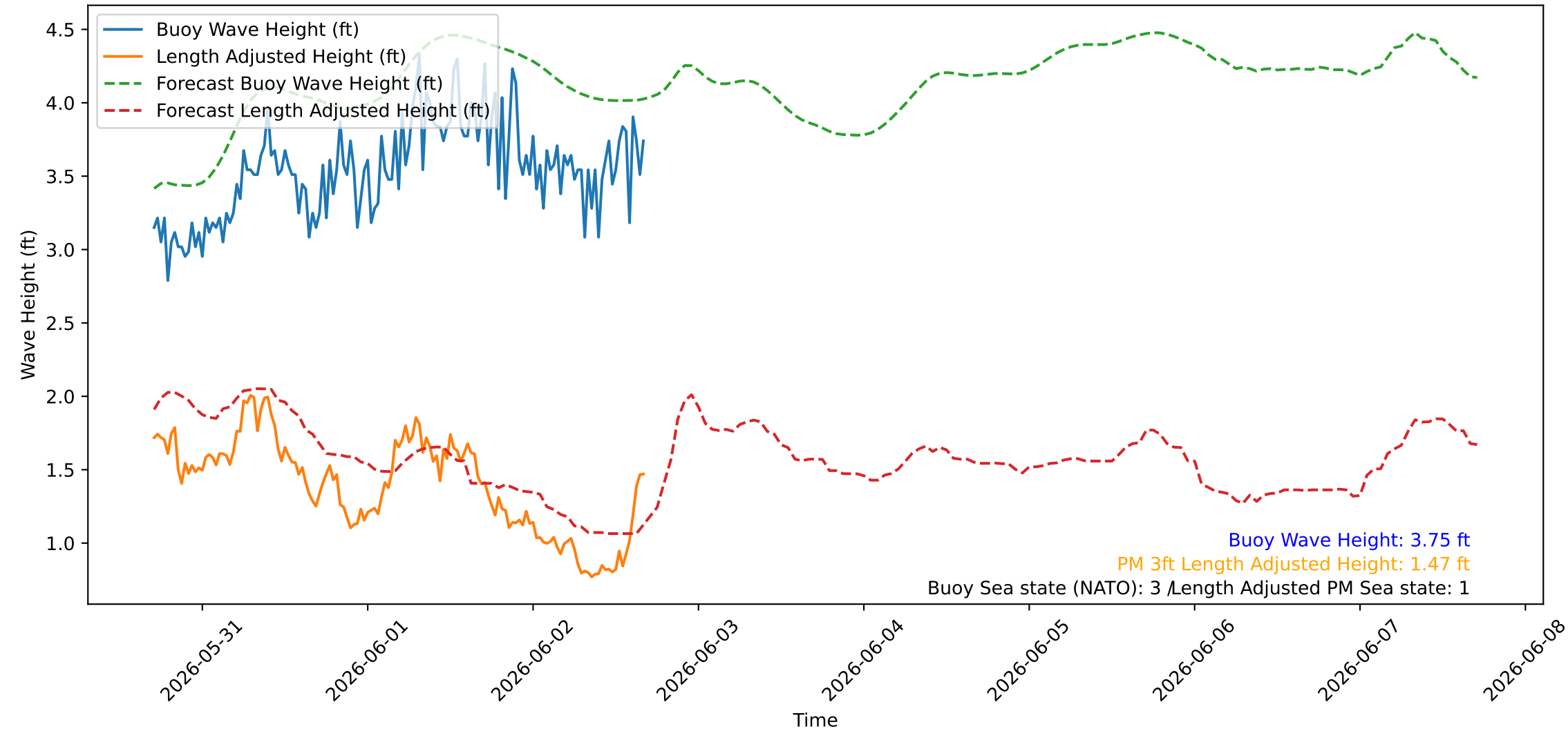
Wave Heights over Time for Green Beach at 2026-06-02 16:51:09
