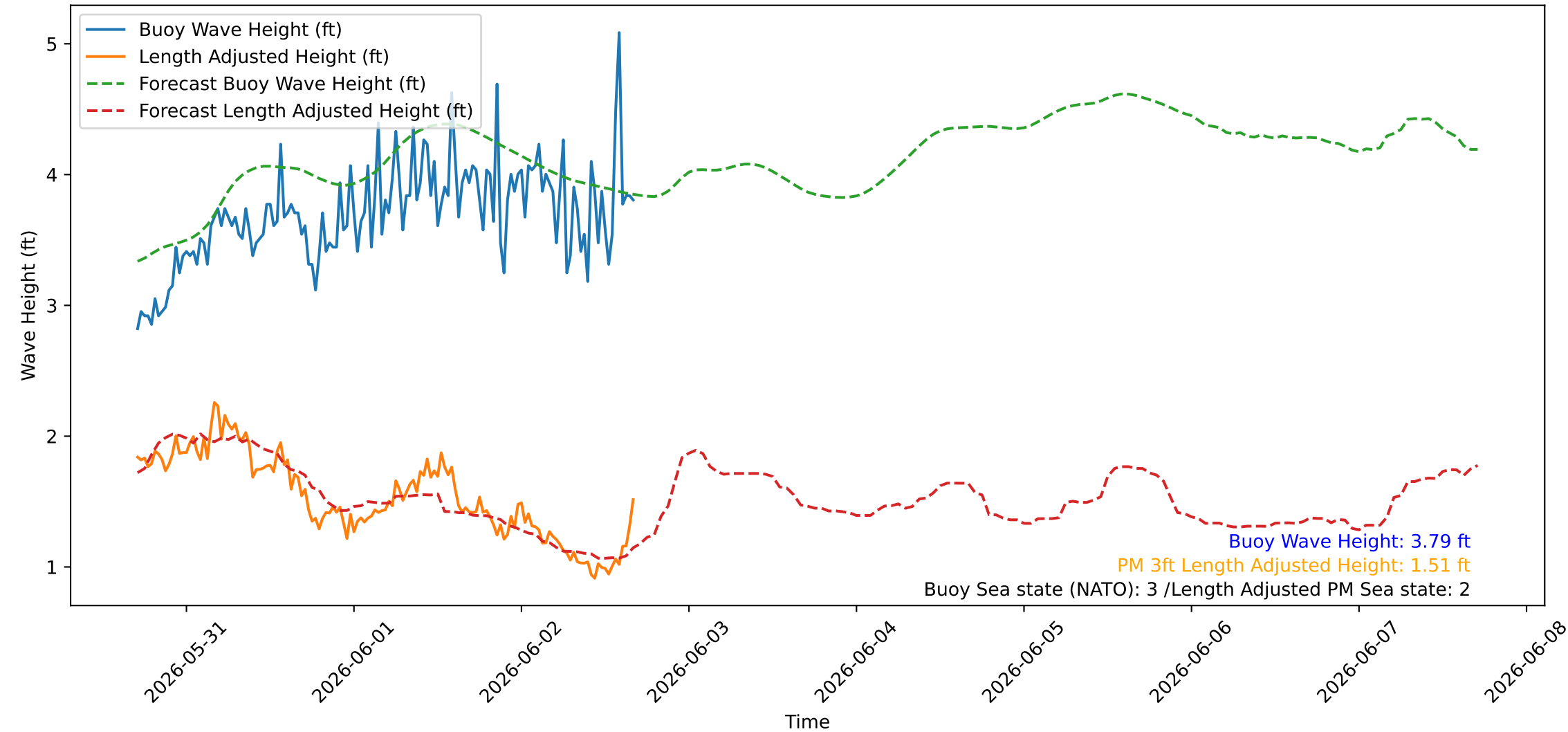
Wave Heights over Time for Oceanside Harbor at 2026-06-02 16:50:26
