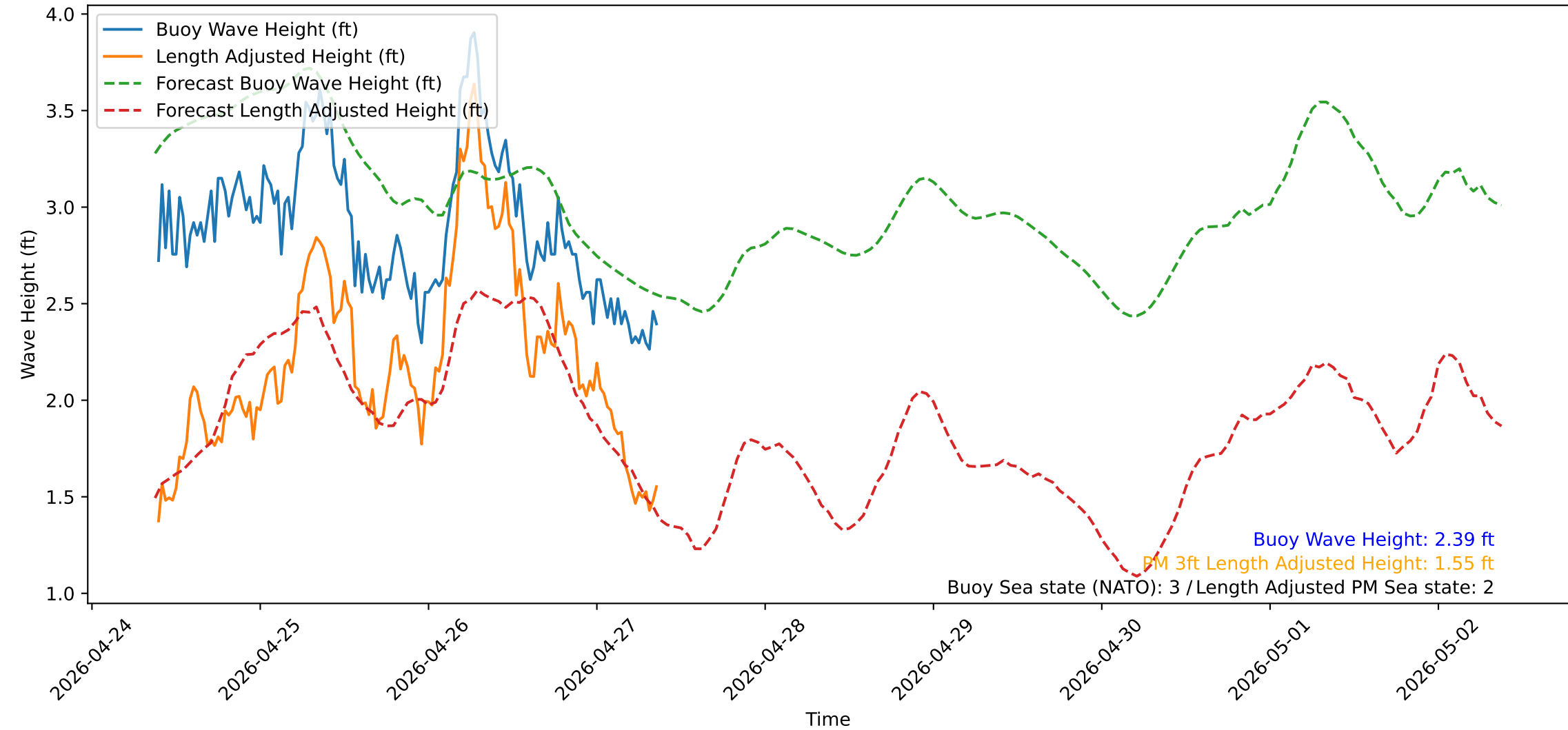
Wave Heights over Time for Oceanside Harbor at 2026-04-27 09:20:31
