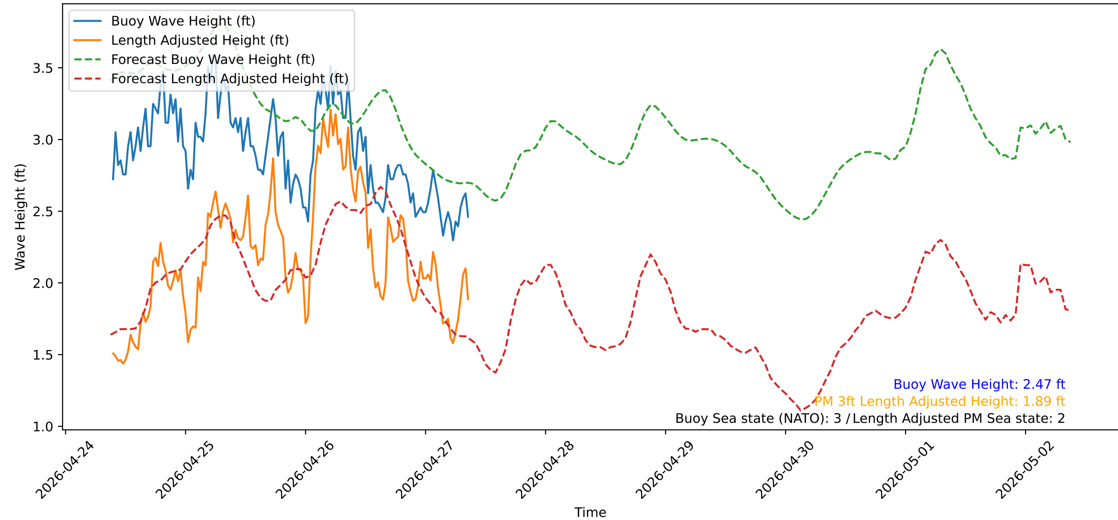
Wave Heights over Time for Green Beach at 2026-04-27 09:21:13
