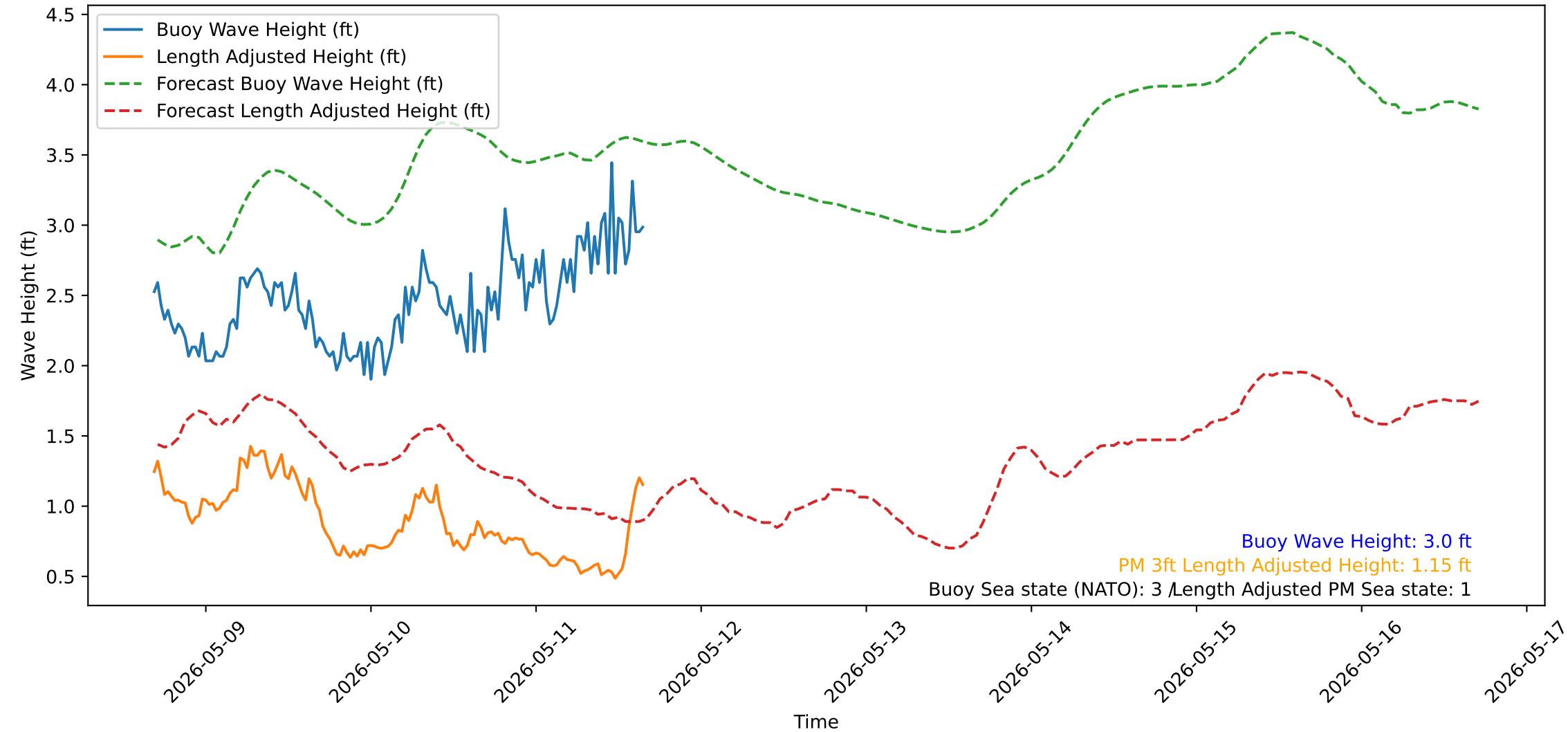
Wave Heights over Time for Green Beach at 2026-05-11 16:31:12
