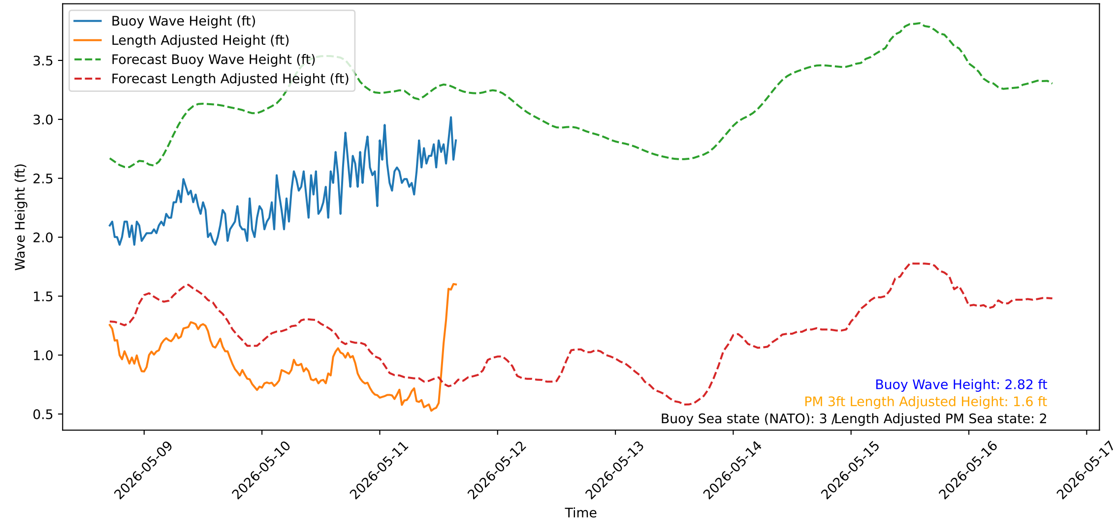
Wave Heights over Time for Red Beach at 2026-05-11 16:30:50
