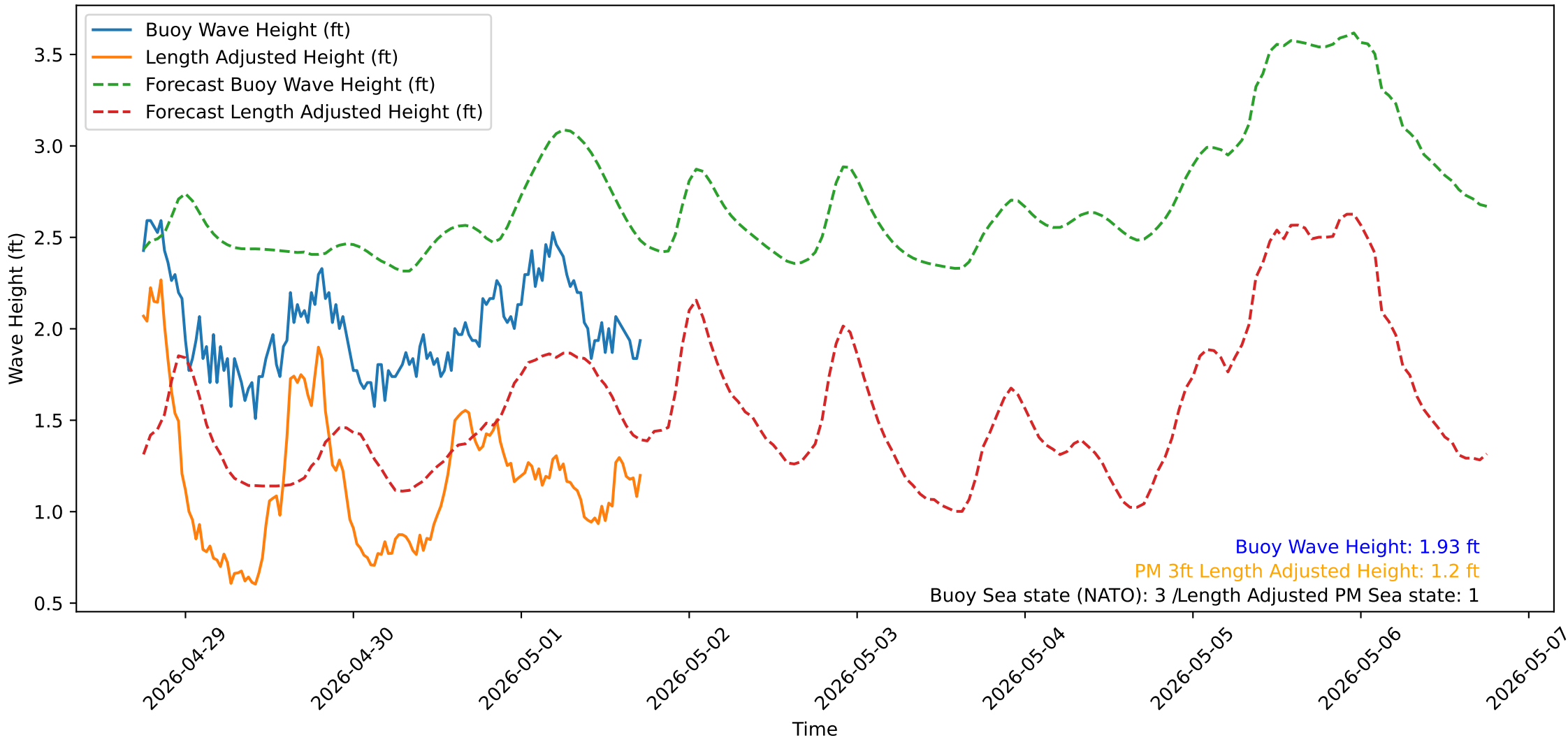
Wave Heights over Time for Red Beach at 2026-05-01 17:50:52
