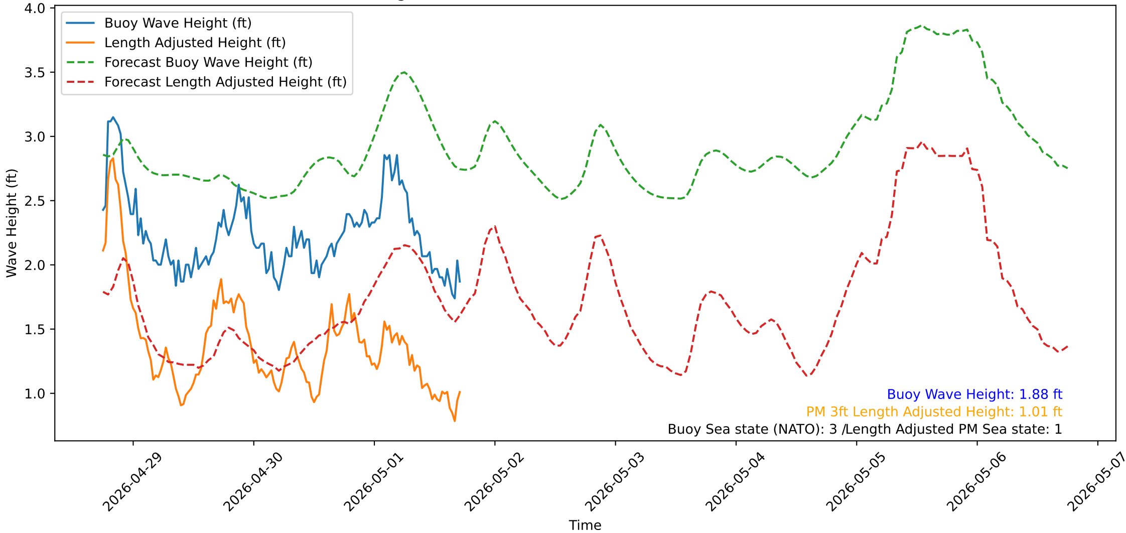
Wave Heights over Time for Green Beach at 2026-05-01 17:51:14
