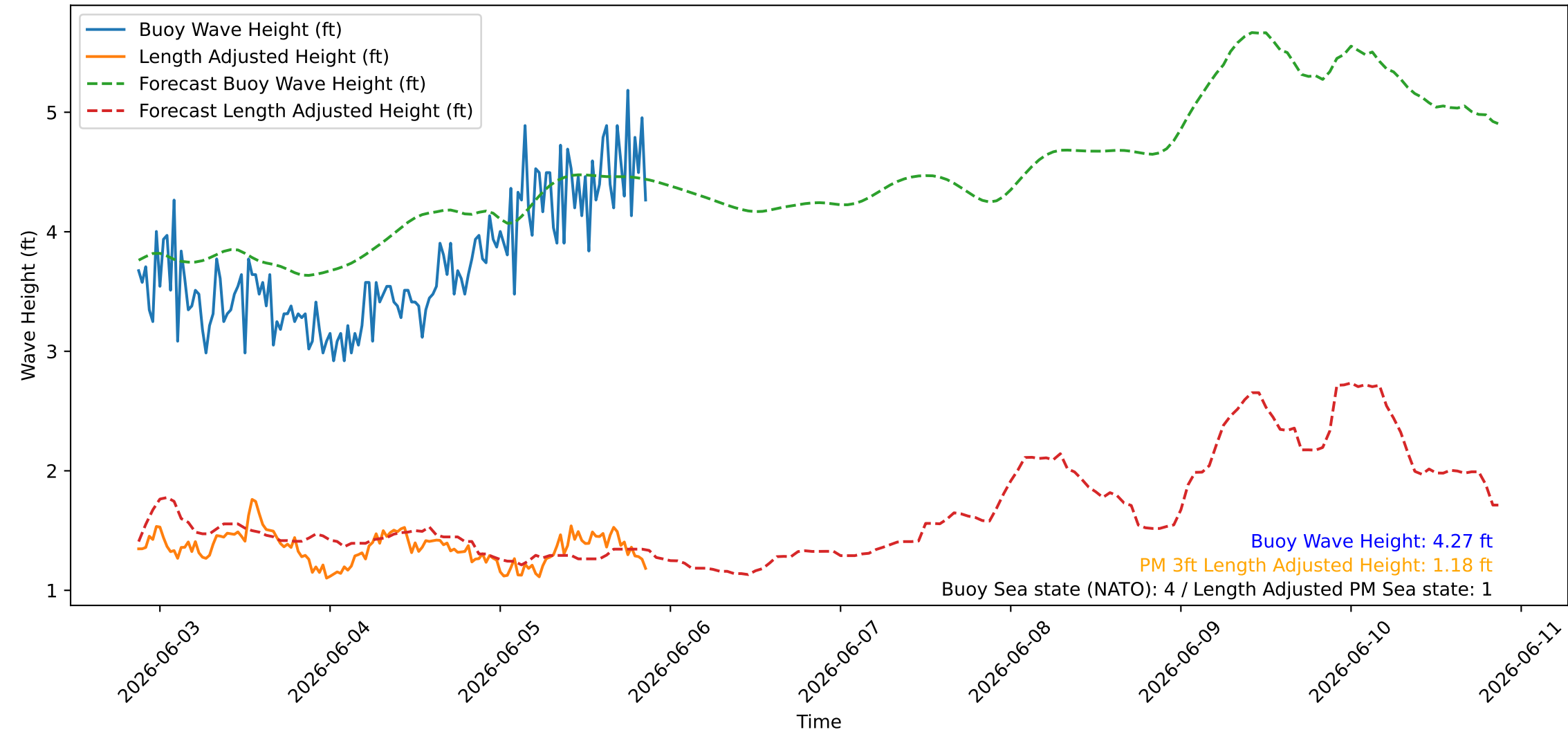
Wave Heights over Time for Oceanside Harbor at 2026-06-05 21:10:26
