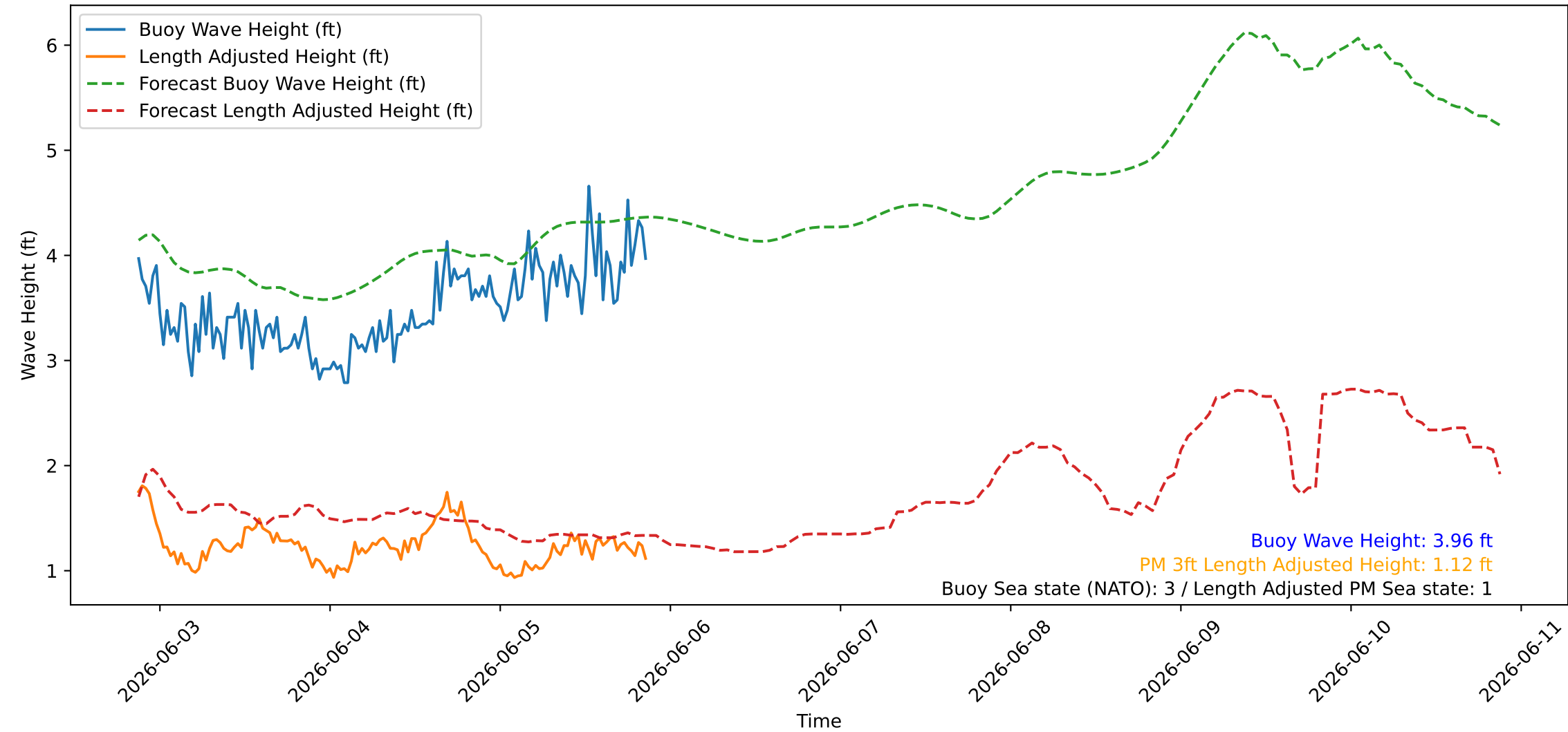
Wave Heights over Time for Green Beach at 2026-06-05 21:11:08
