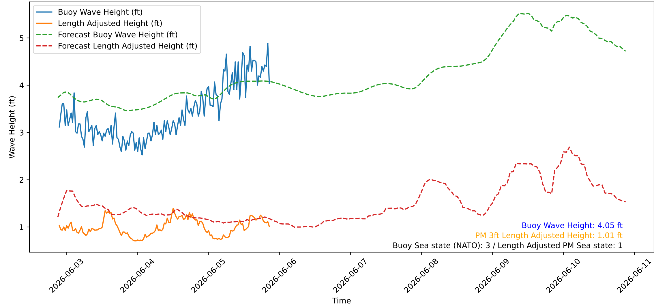
Wave Heights over Time for Red Beach at 2026-06-05 21:10:46
