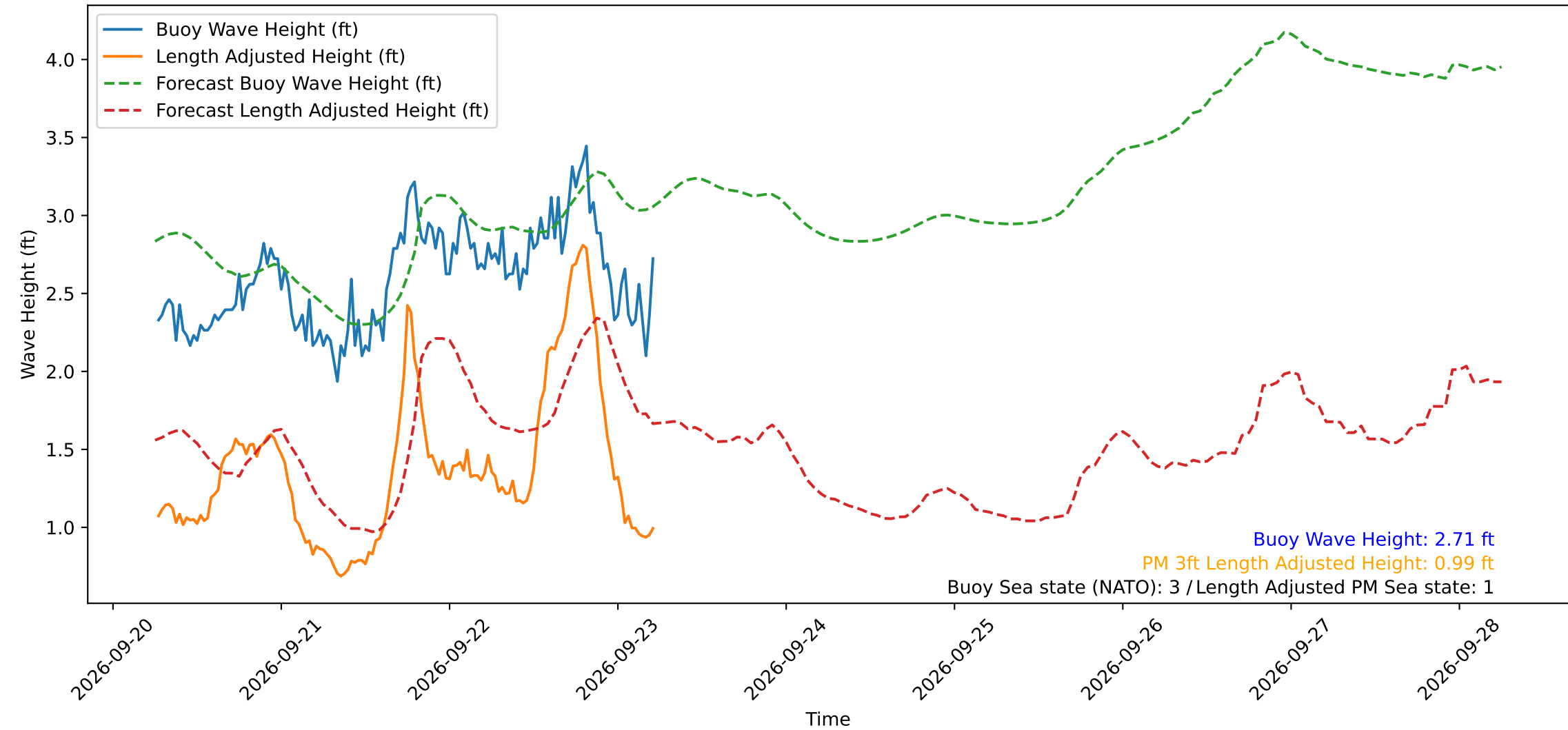
Wave Heights over Time for Green Beach at 2026-09-23 06:01:11
