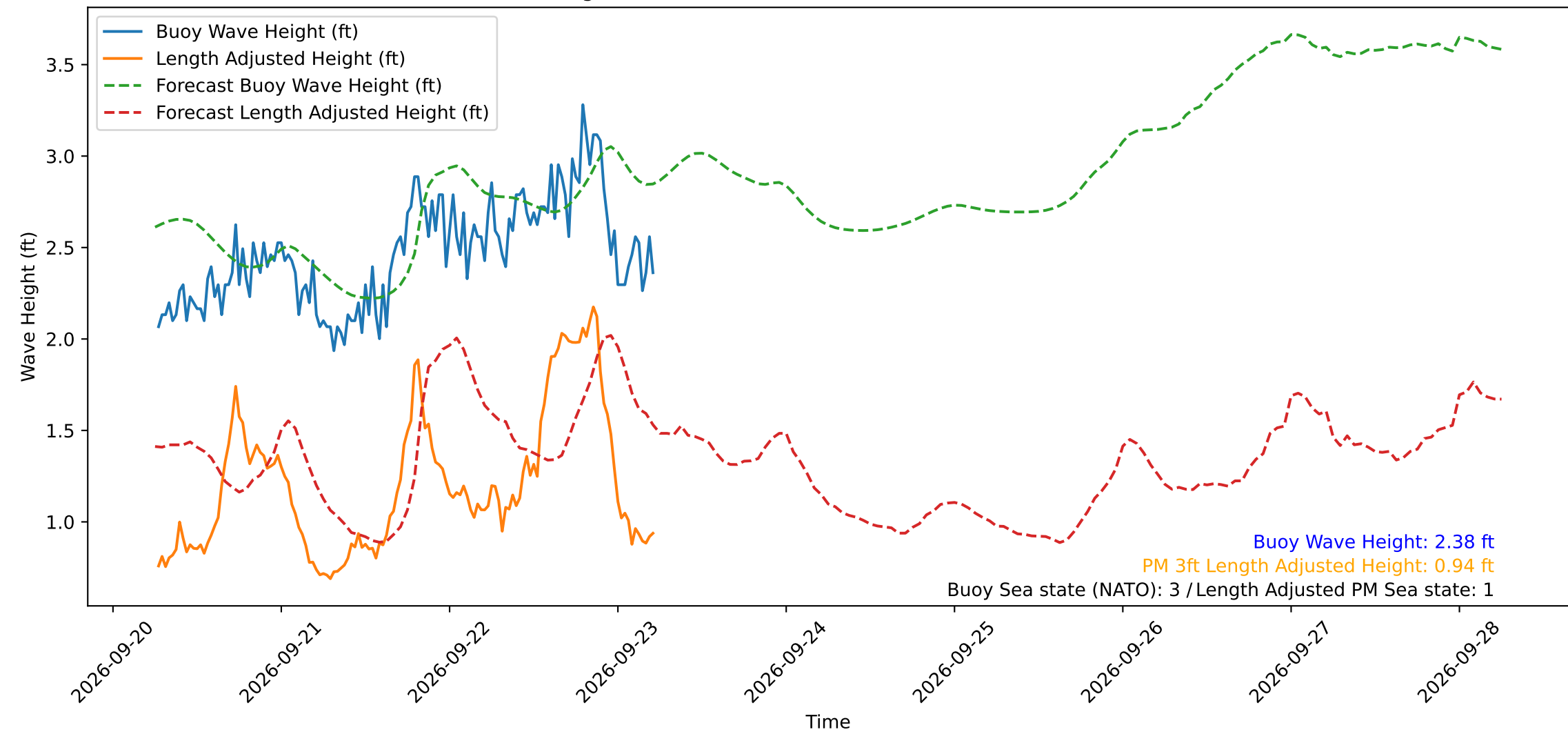
Wave Heights over Time for Red Beach at 2026-09-23 06:00:49
