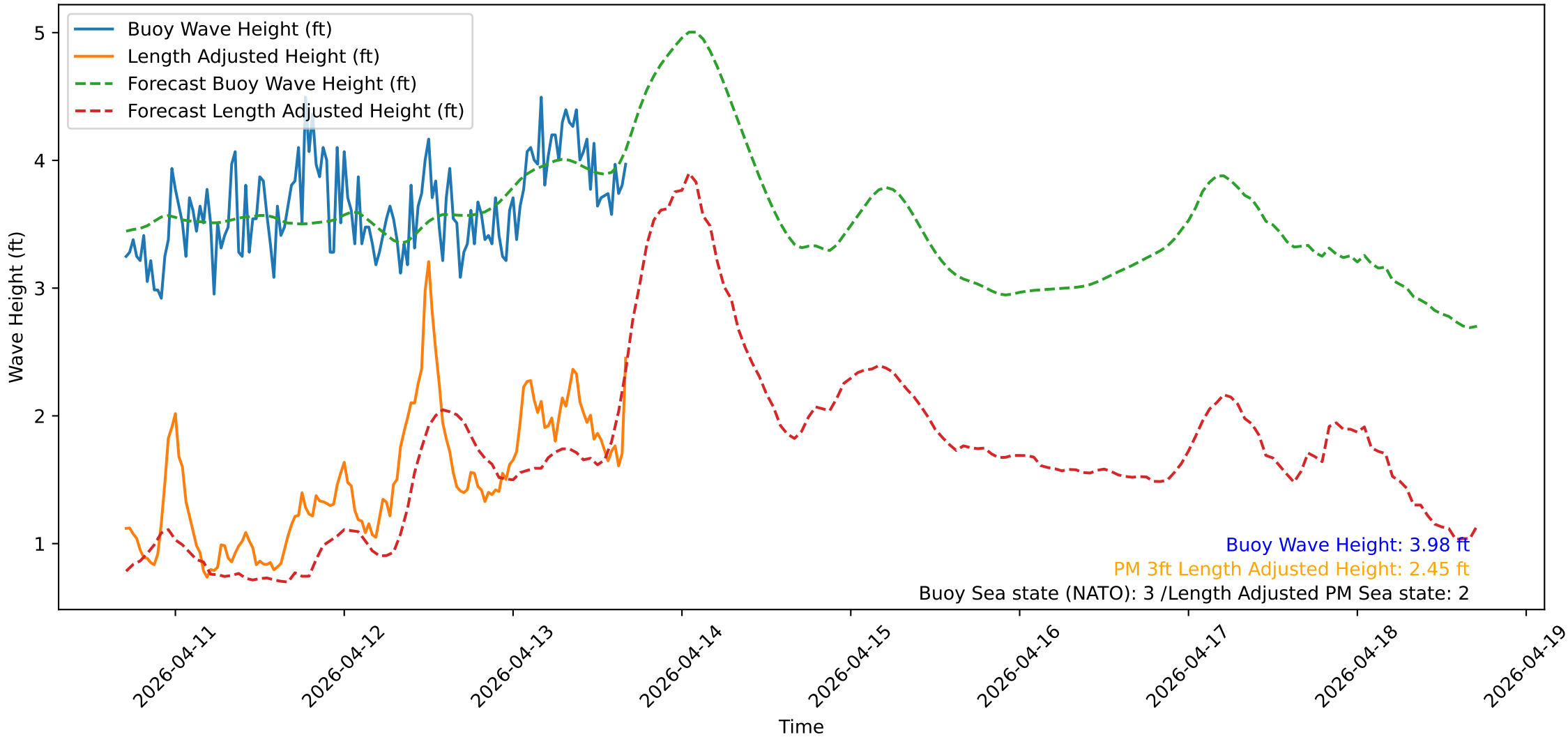
Wave Heights over Time for Green Beach at 2026-04-13 17:01:12
