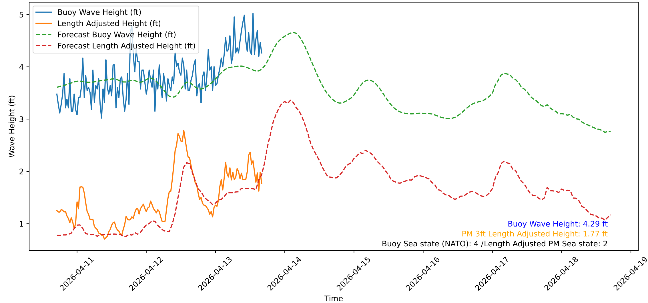
Wave Heights over Time for Oceanside Harbor at 2026-04-13 17:00:31
