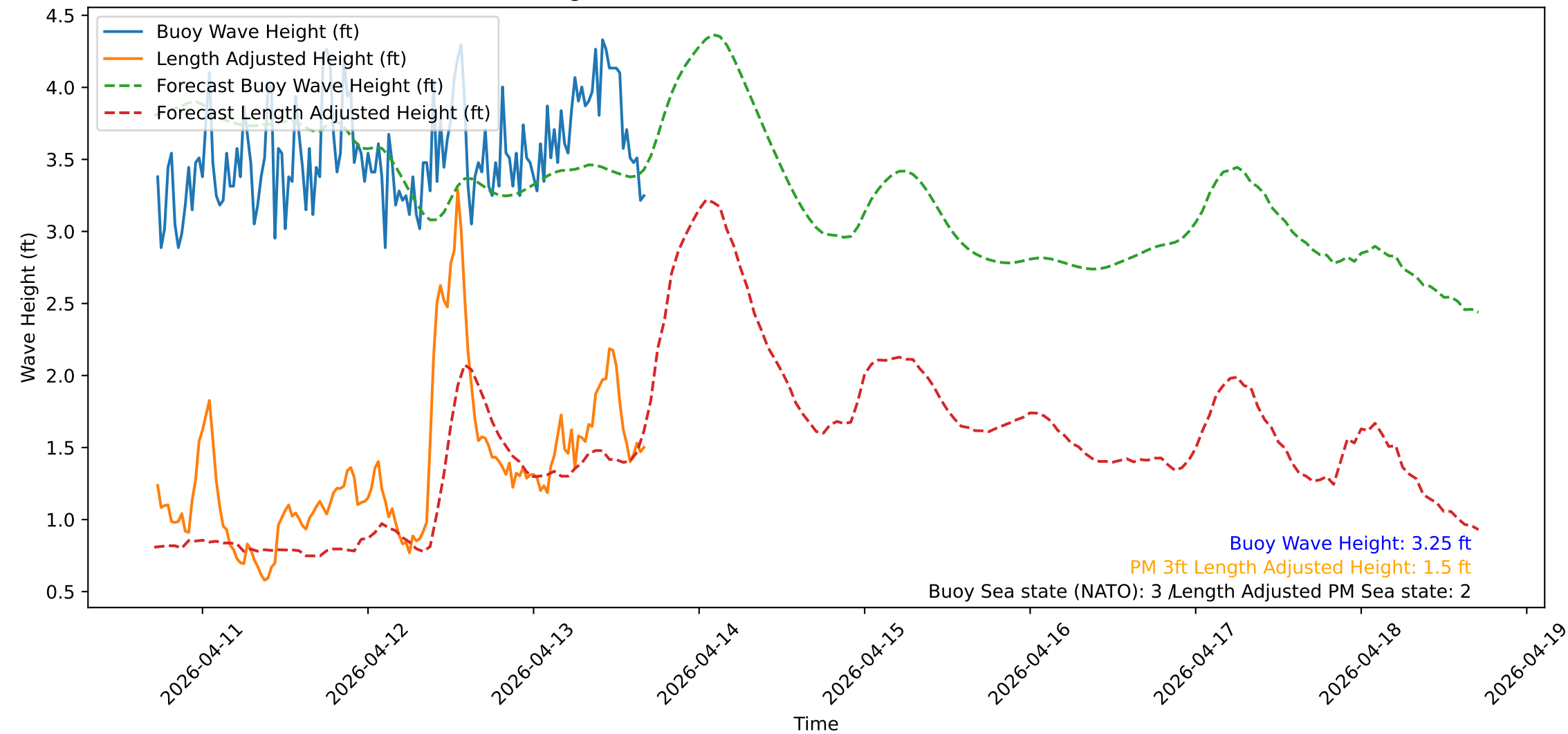
Wave Heights over Time for Red Beach at 2026-04-13 17:00:50
