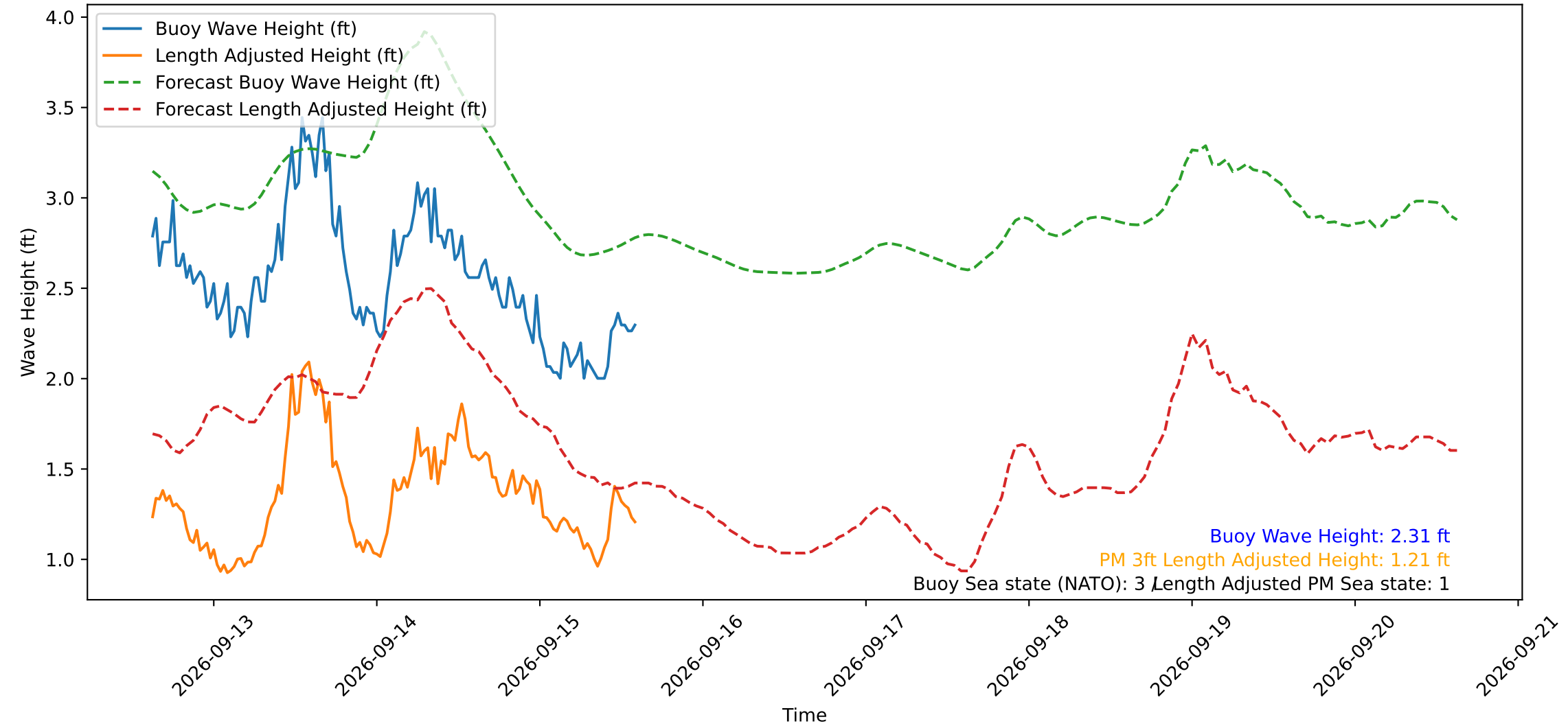
Wave Heights over Time for Red Beach at 2026-09-15 14:50:50
