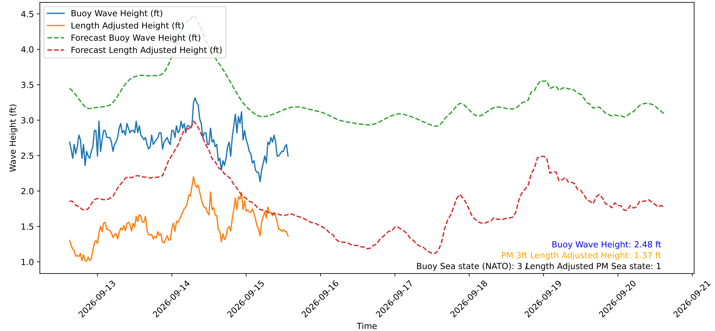
Wave Heights over Time for Green Beach at 2026-09-15 14:51:13
