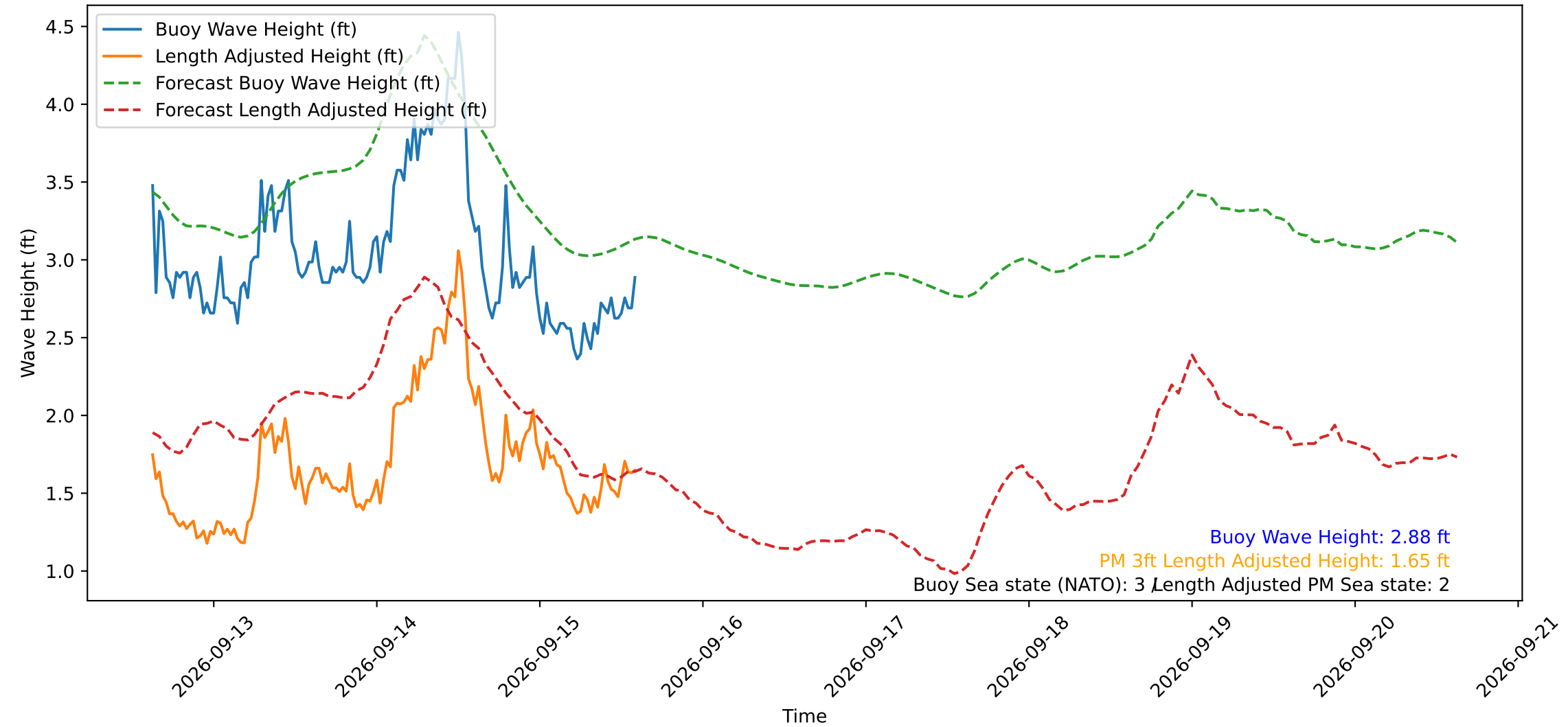
Wave Heights over Time for Oceanside Harbor at 2026-09-15 14:50:29
