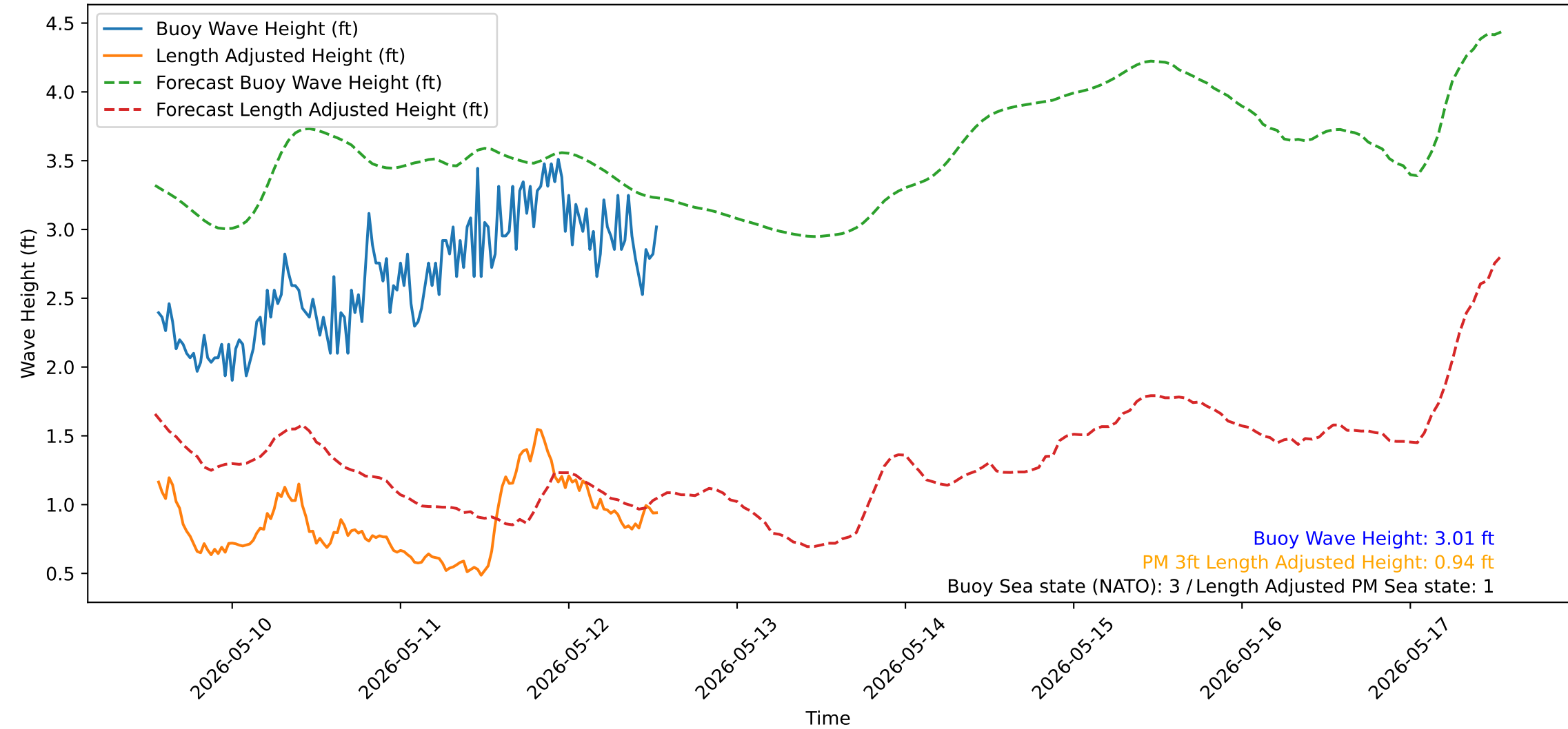
Wave Heights over Time for Green Beach at 2026-05-12 13:21:14
