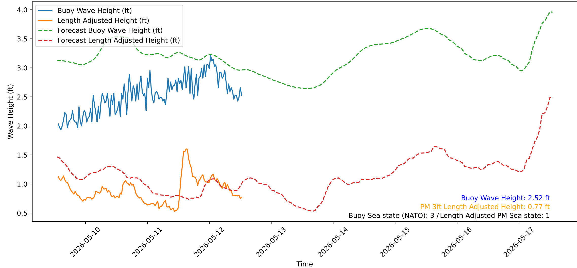
Wave Heights over Time for Red Beach at 2026-05-12 13:20:51
