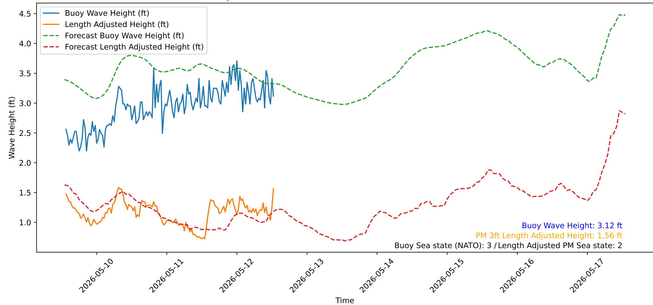
Wave Heights over Time for Oceanside Harbor at 2026-05-12 13:20:31
