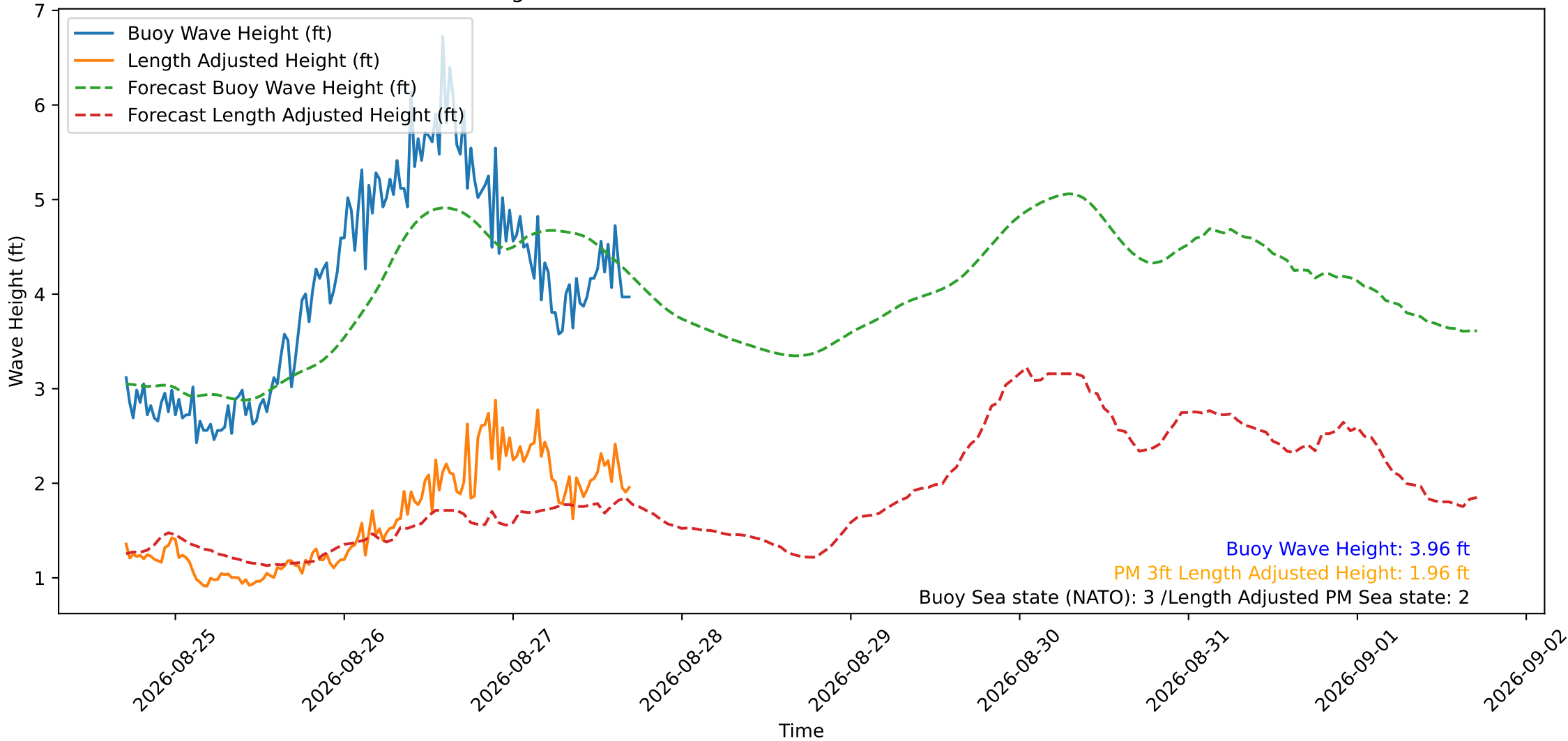
Wave Heights over Time for Oceanside Harbor at 2026-08-27 17:10:29
