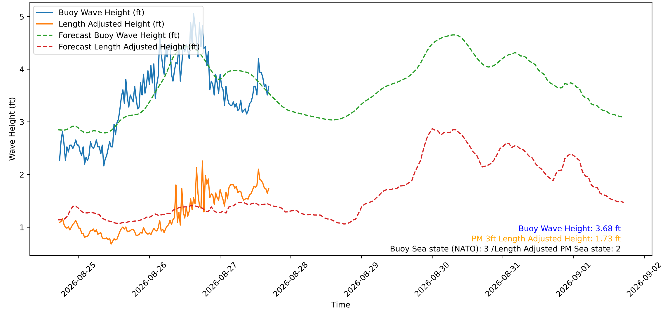
Wave Heights over Time for Red Beach at 2026-08-27 17:10:49
