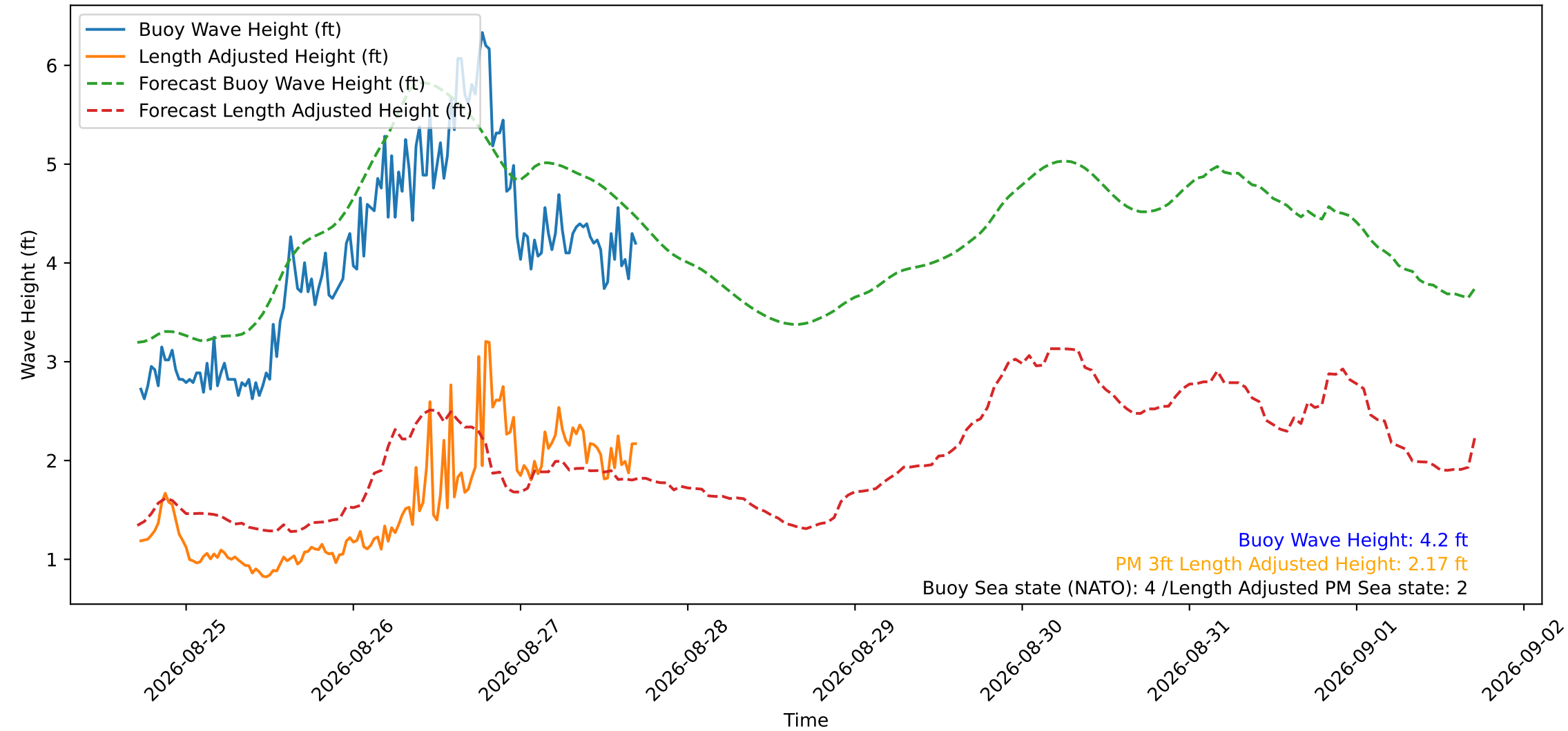
Wave Heights over Time for Green Beach at 2026-08-27 17:11:12
