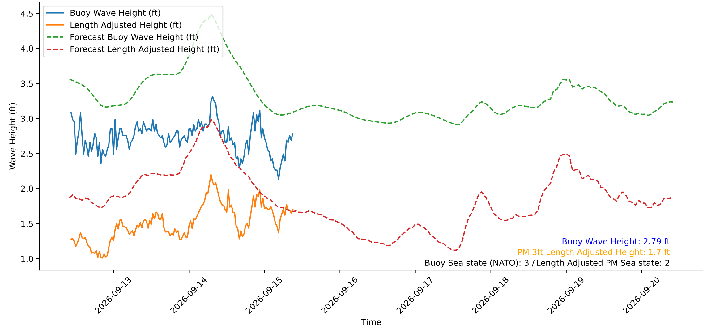
Wave Heights over Time for Green Beach at 2026-09-15 10:01:11
