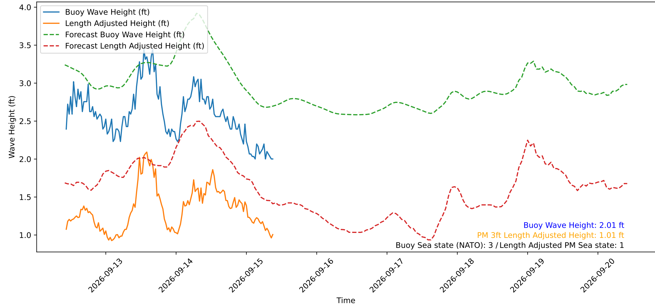
Wave Heights over Time for Red Beach at 2026-09-15 10:00:49
