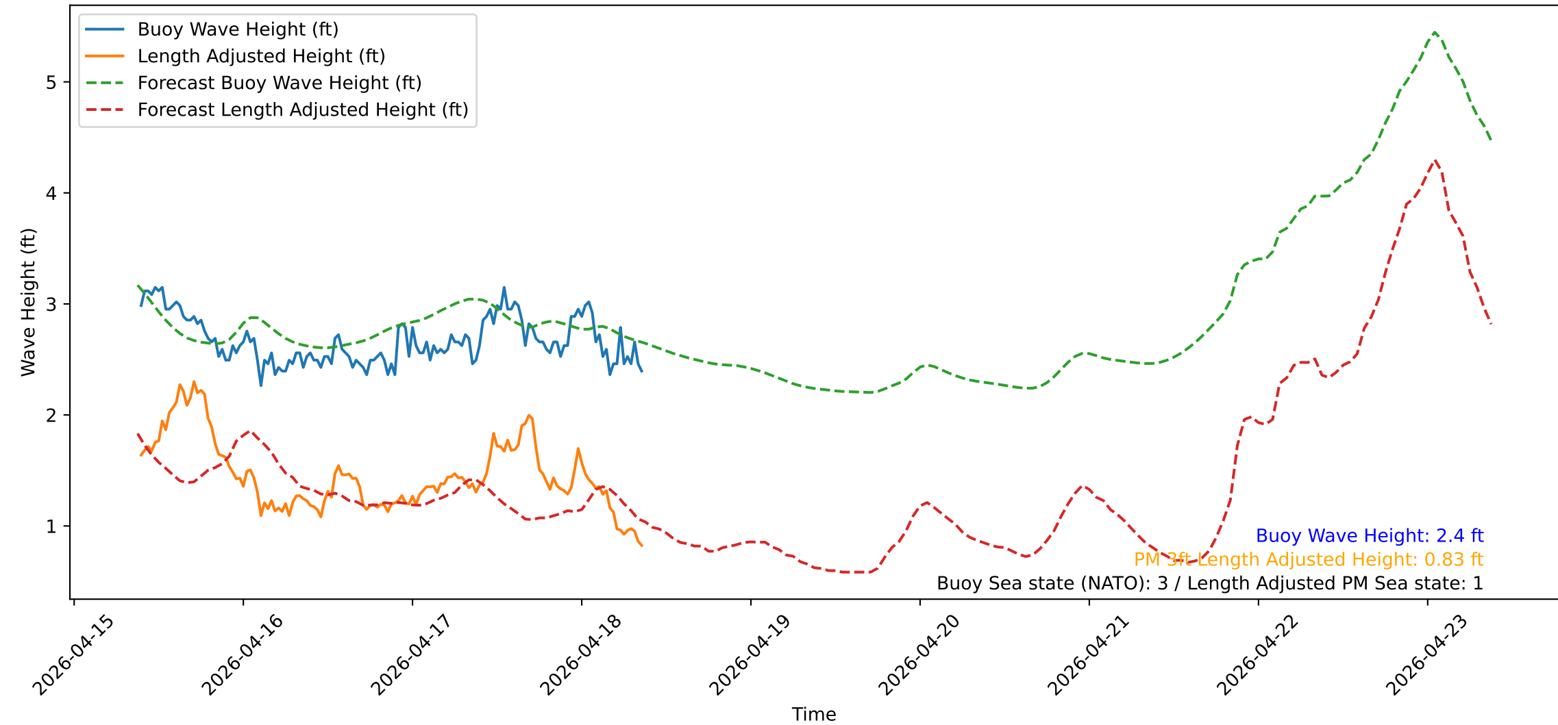
Wave Heights over Time for Red Beach at 2026-04-18 09:20:51
