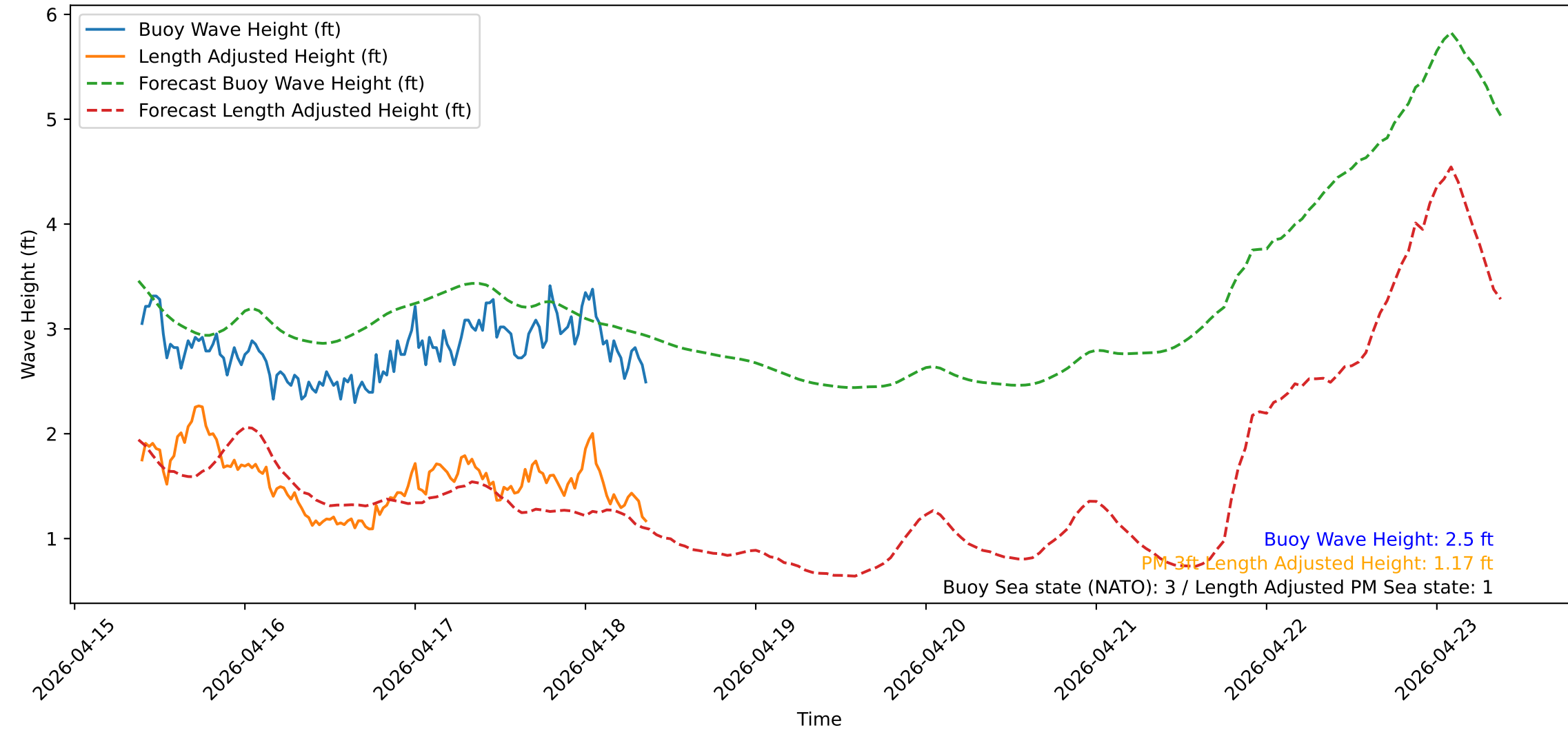
Wave Heights over Time for Oceanside Harbor at 2026-04-18 09:20:31
