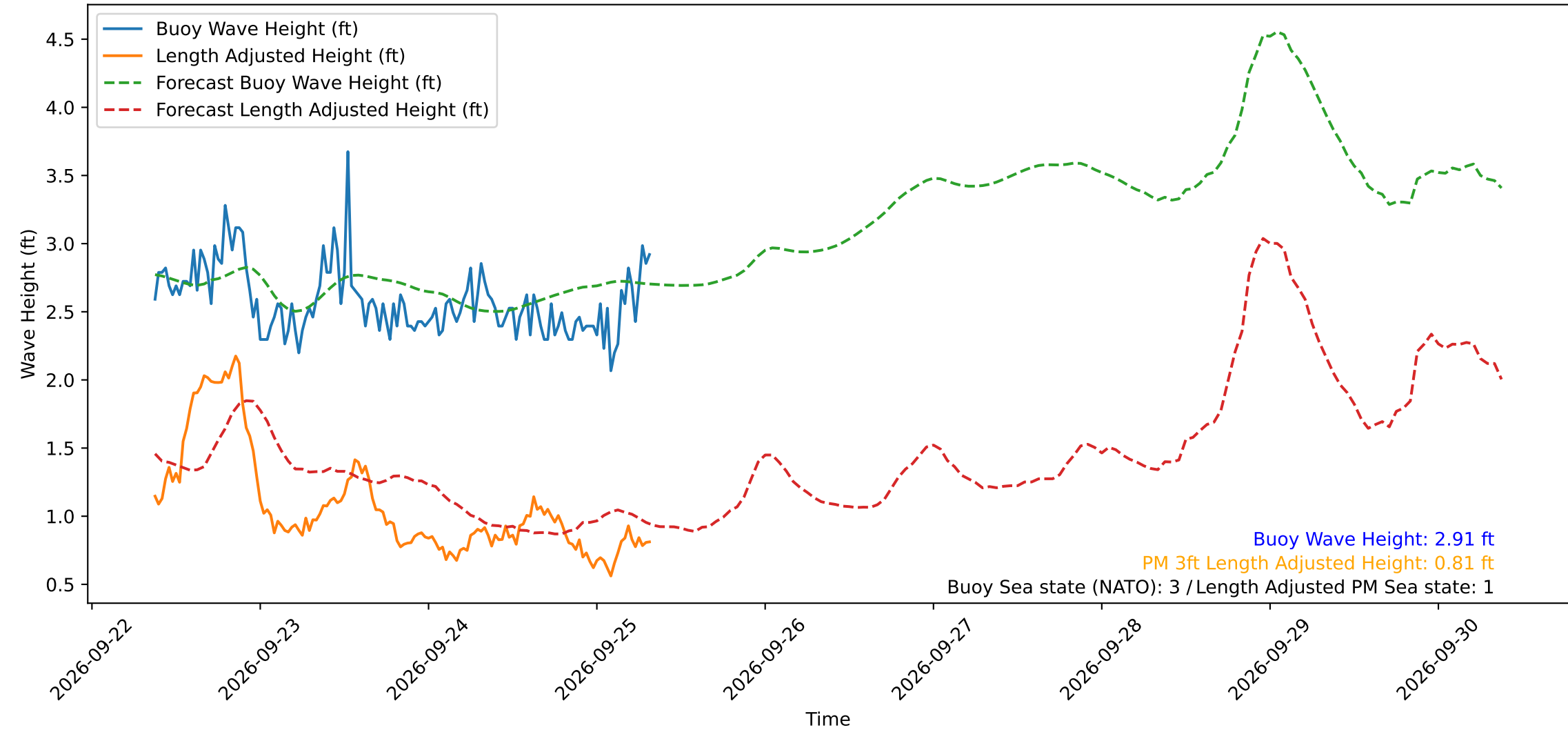
Wave Heights over Time for Red Beach at 2026-09-25 08:30:48
