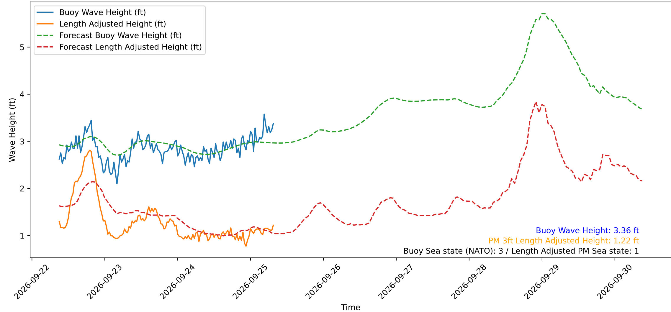
Wave Heights over Time for Green Beach at 2026-09-25 08:31:10
