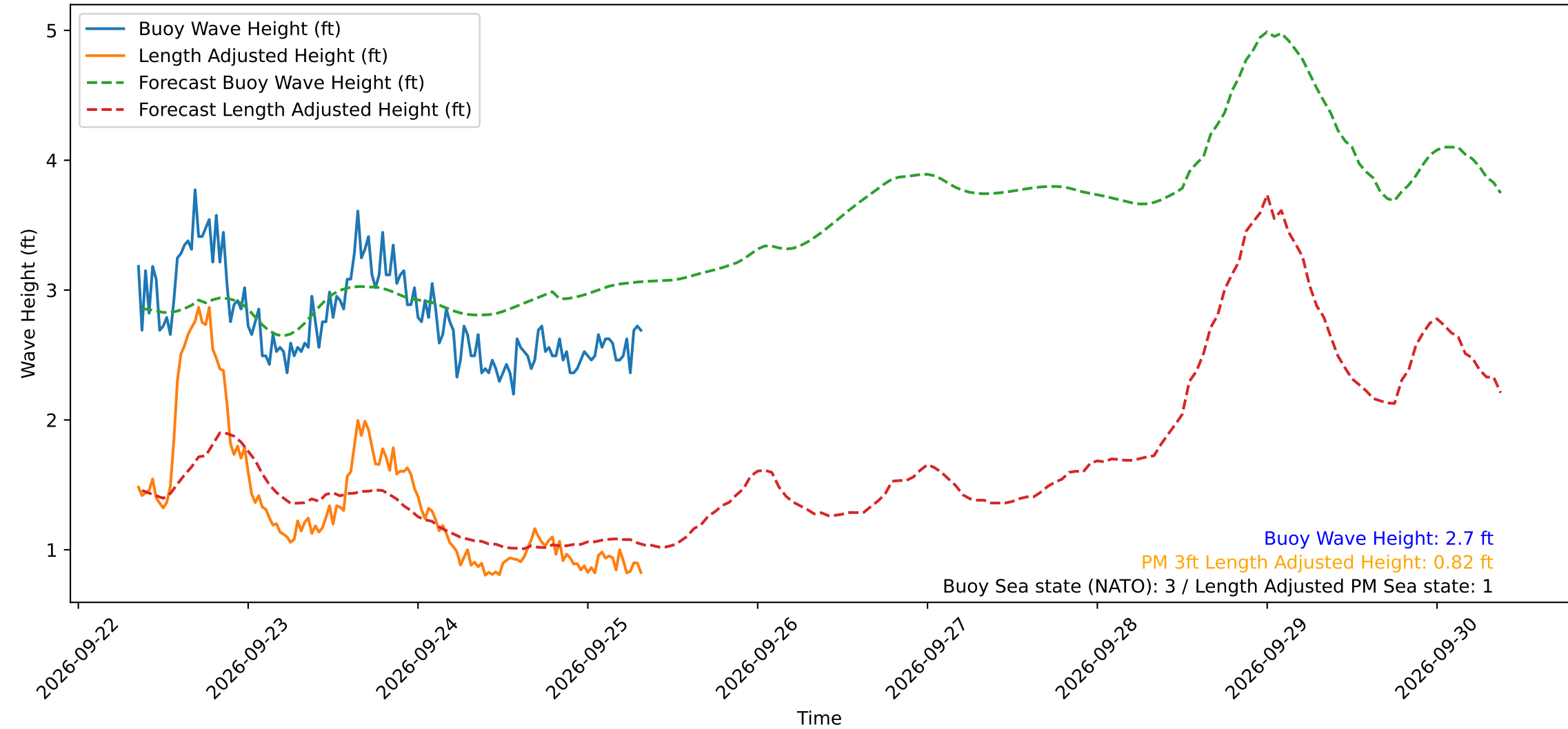
Wave Heights over Time for Oceanside Harbor at 2026-09-25 08:30:29
