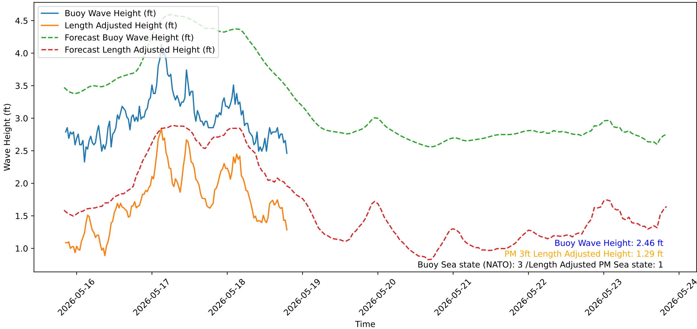
Wave Heights over Time for Red Beach at 2026-05-18 20:00:52
