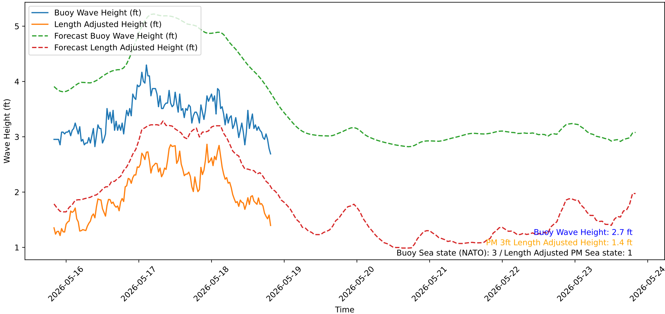
Wave Heights over Time for Oceanside Harbor at 2026-05-18 20:00:32
