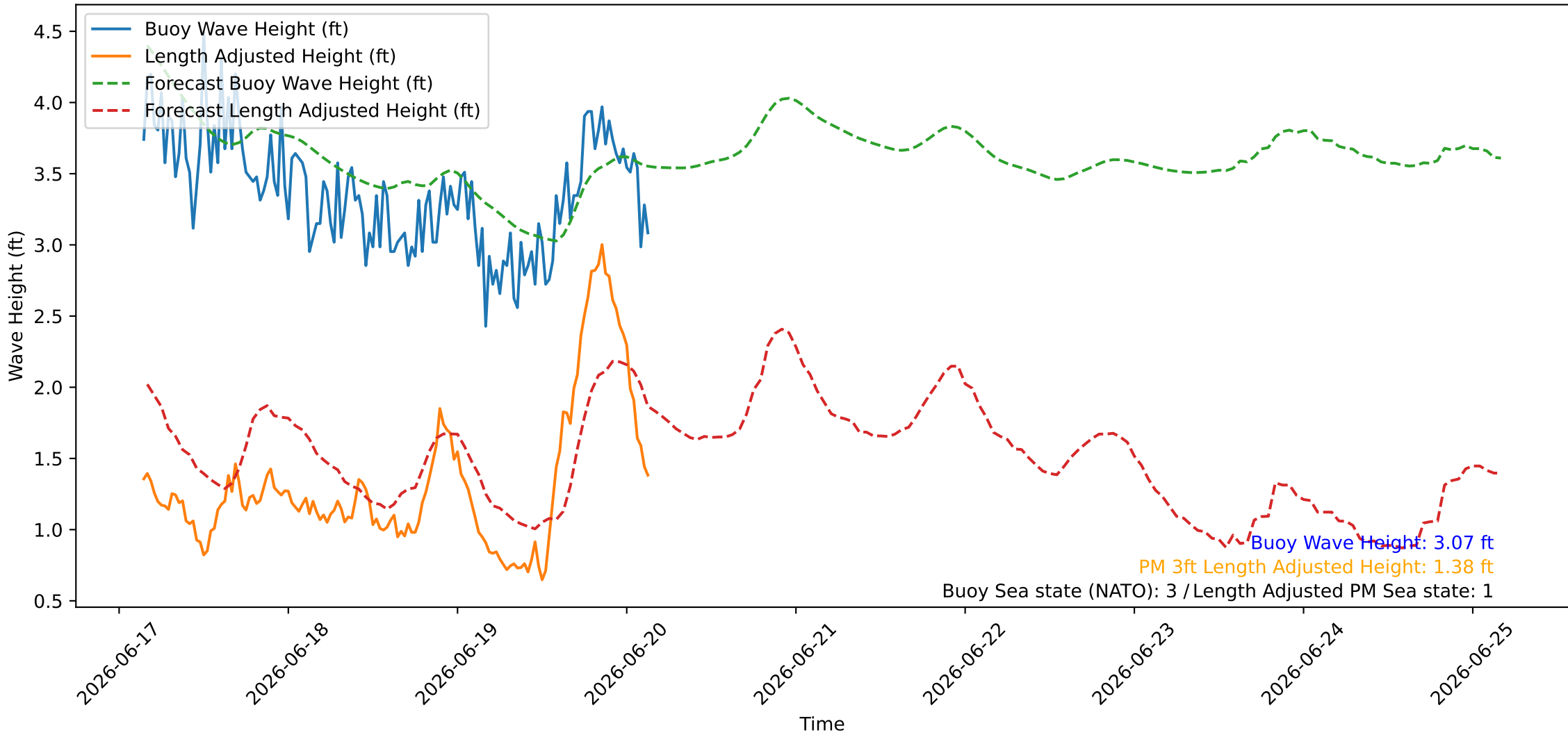
Wave Heights over Time for Green Beach at 2026-06-20 03:41:08
