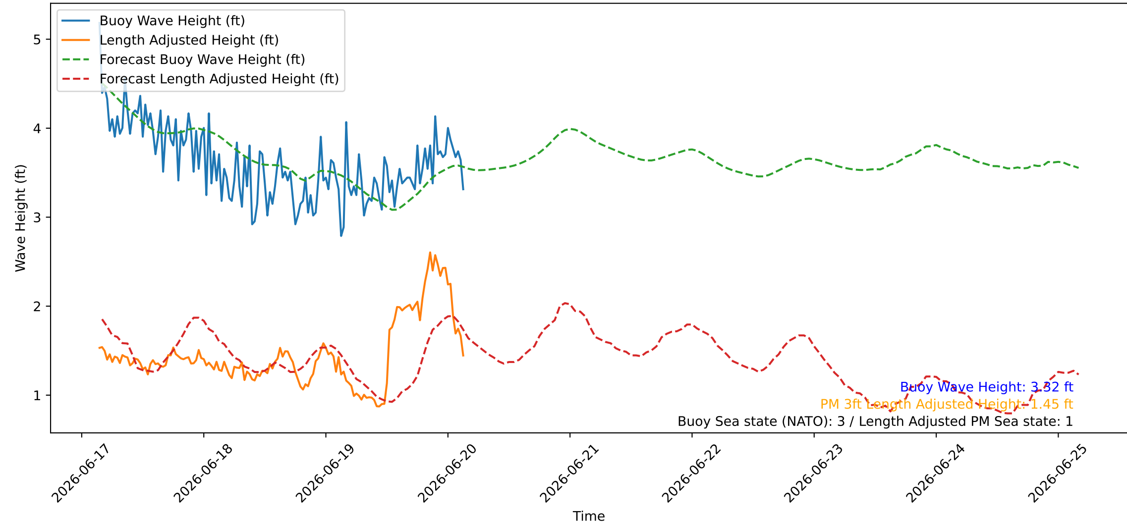
Wave Heights over Time for Oceanside Harbor at 2026-06-20 03:40:26
