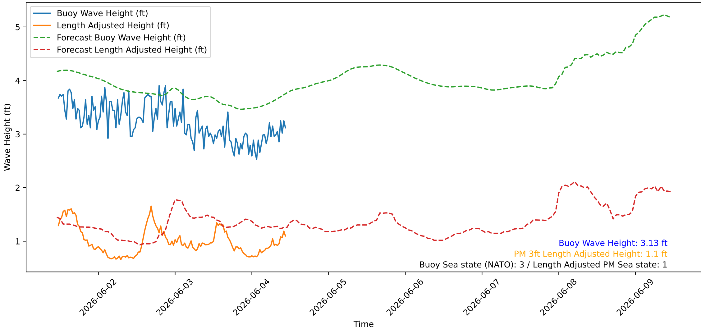
Wave Heights over Time for Red Beach at 2026-06-04 11:20:46
