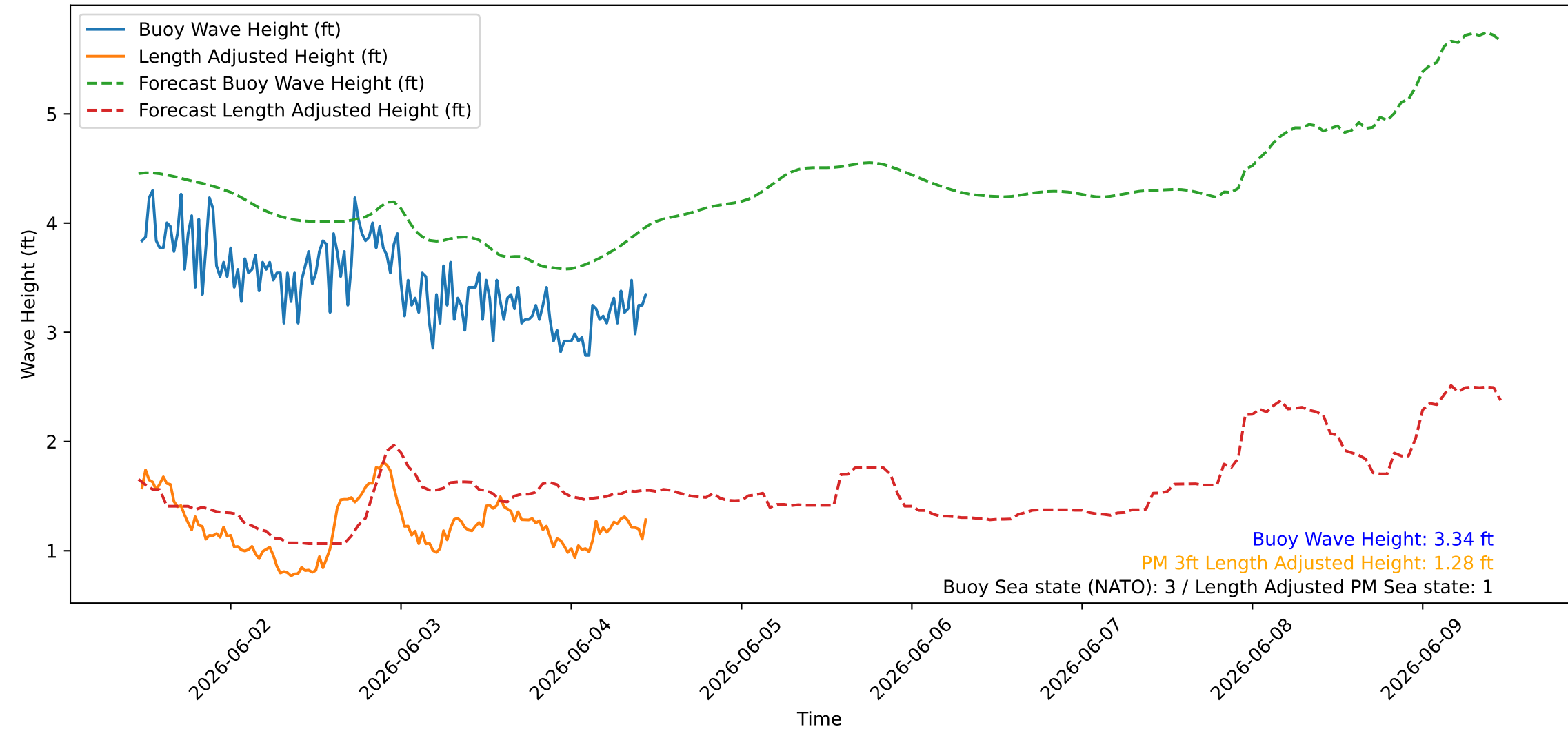
Wave Heights over Time for Green Beach at 2026-06-04 11:21:09
