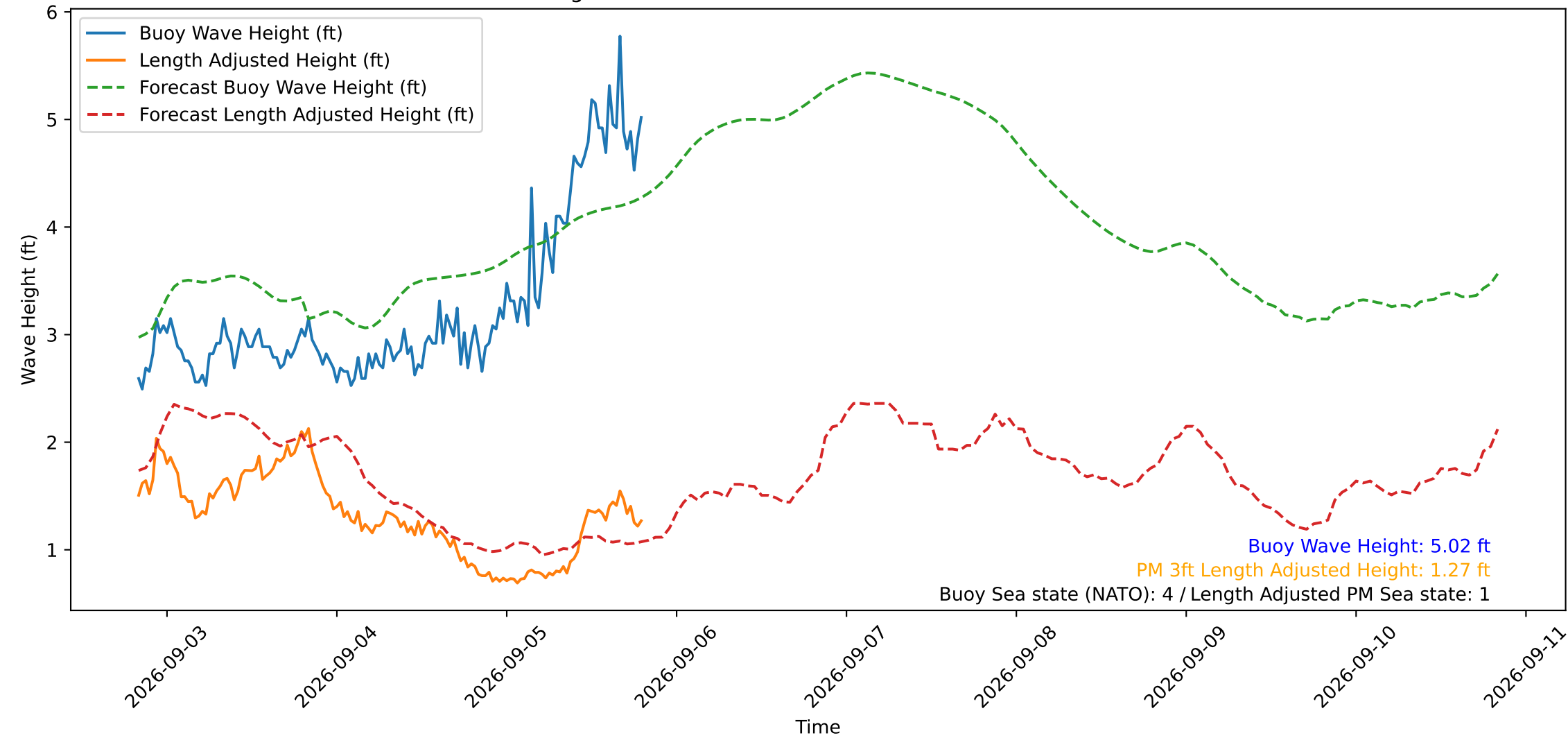
Wave Heights over Time for Red Beach at 2026-09-05 19:40:49
