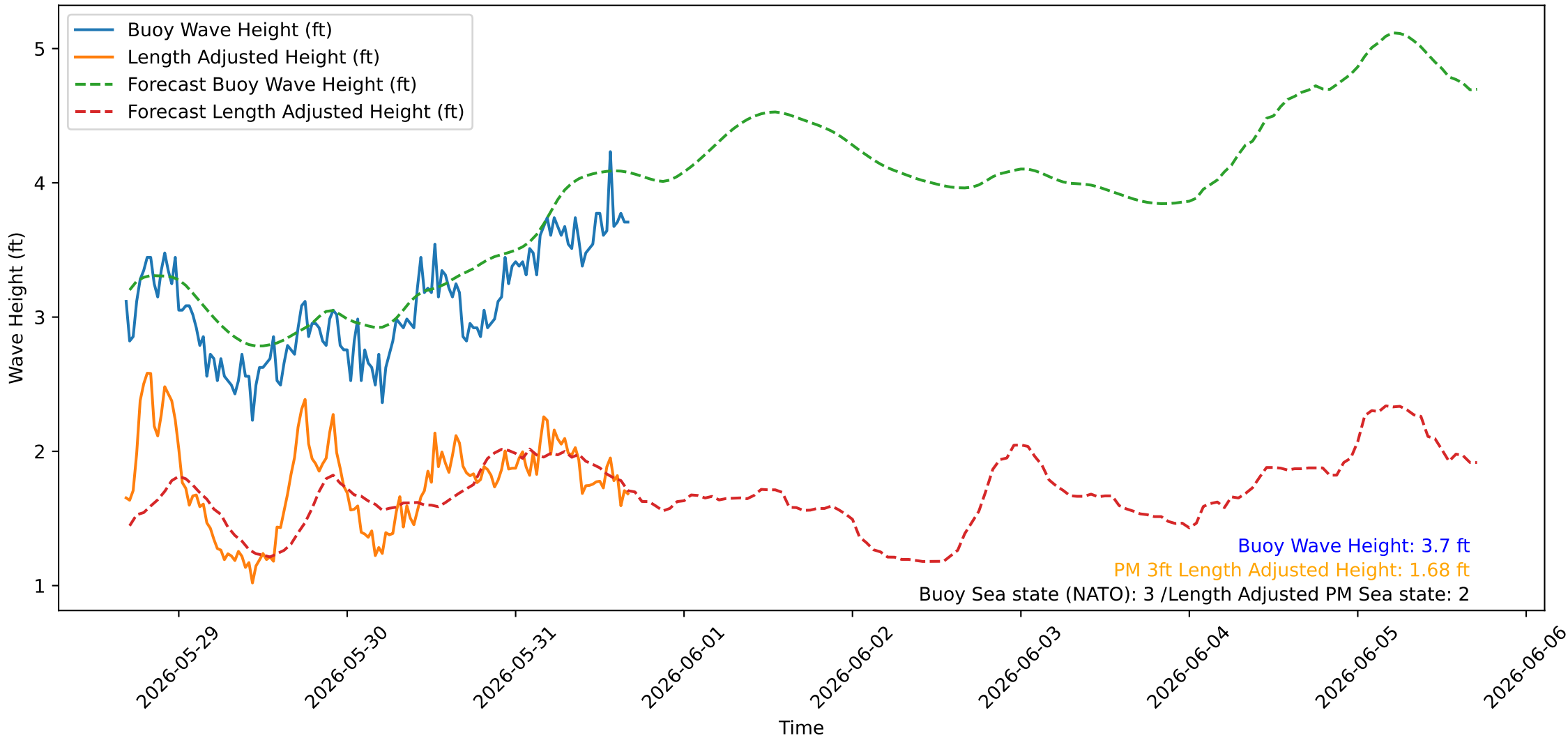
Wave Heights over Time for Oceanside Harbor at 2026-05-31 16:30:26
