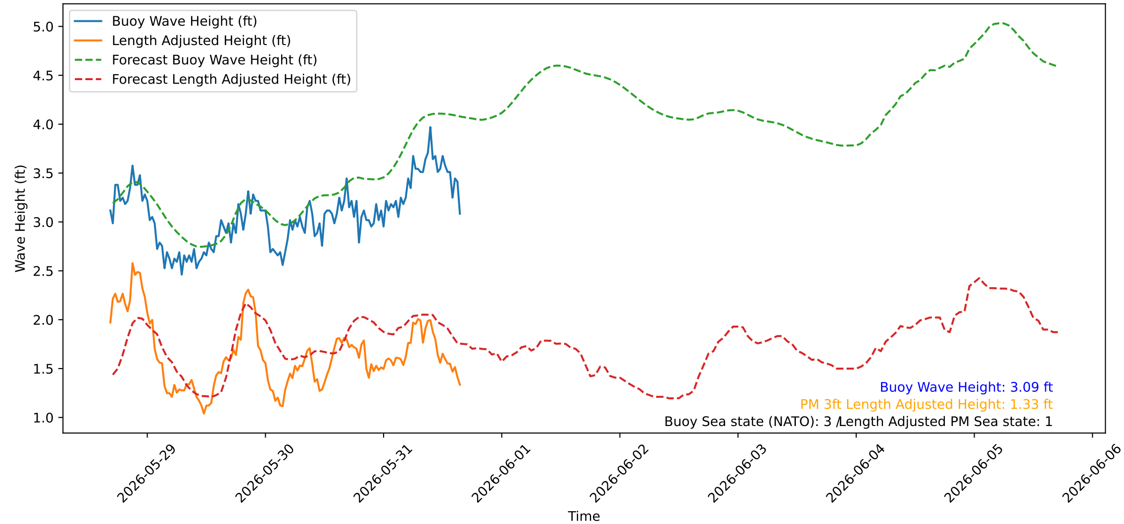
Wave Heights over Time for Green Beach at 2026-05-31 16:31:08
