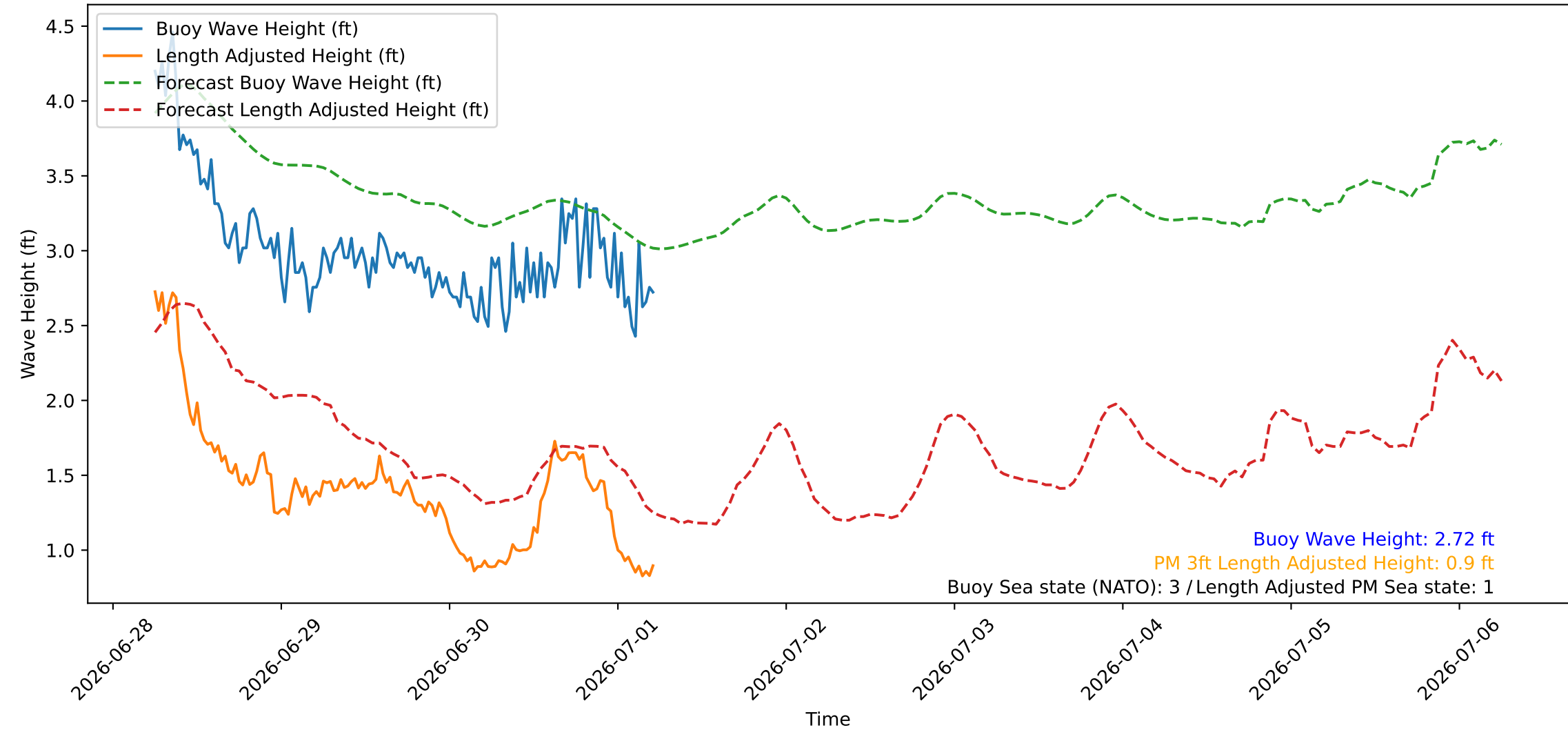
Wave Heights over Time for Red Beach at 2026-07-01 05:40:46
