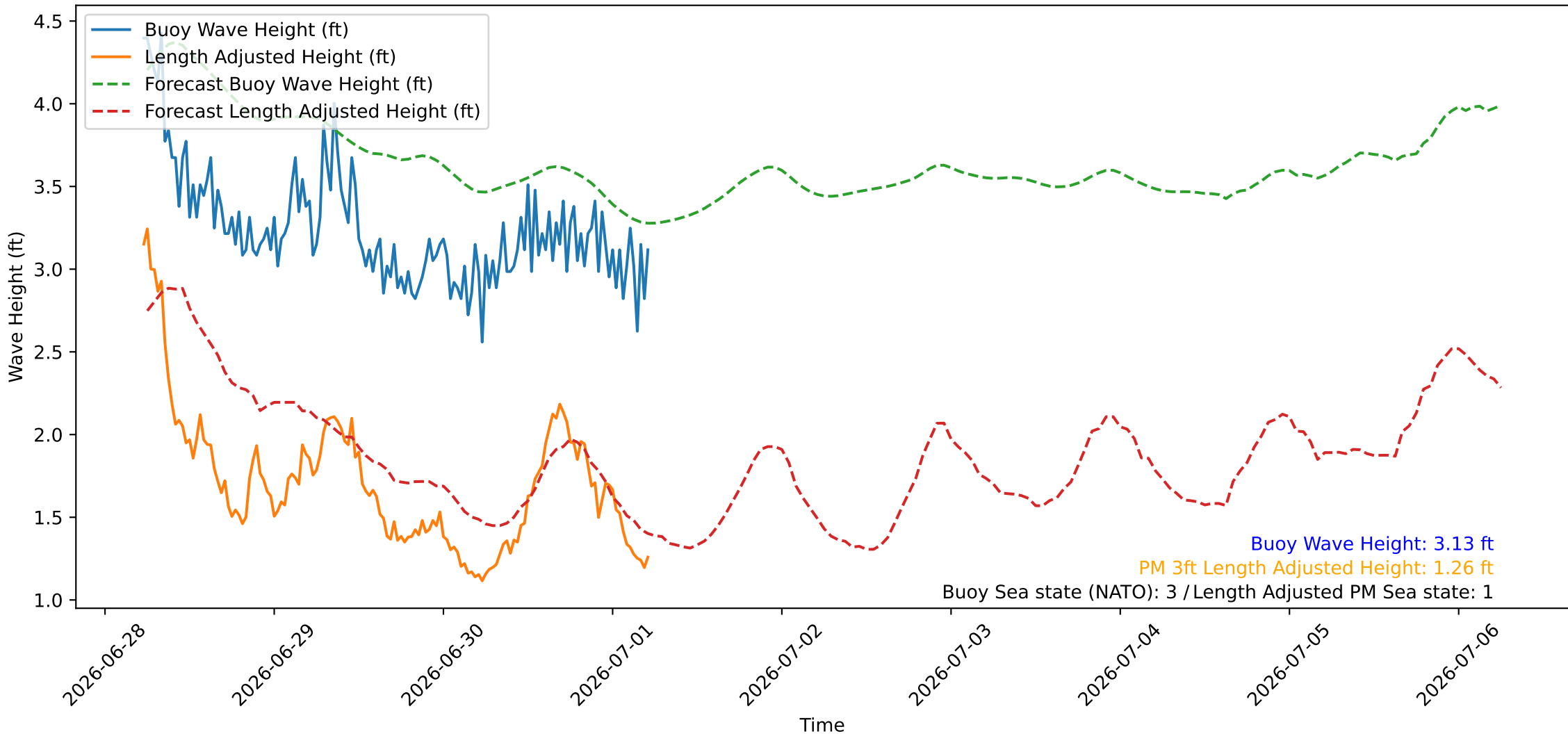
Wave Heights over Time for Oceanside Harbor at 2026-07-01 05:40:26
