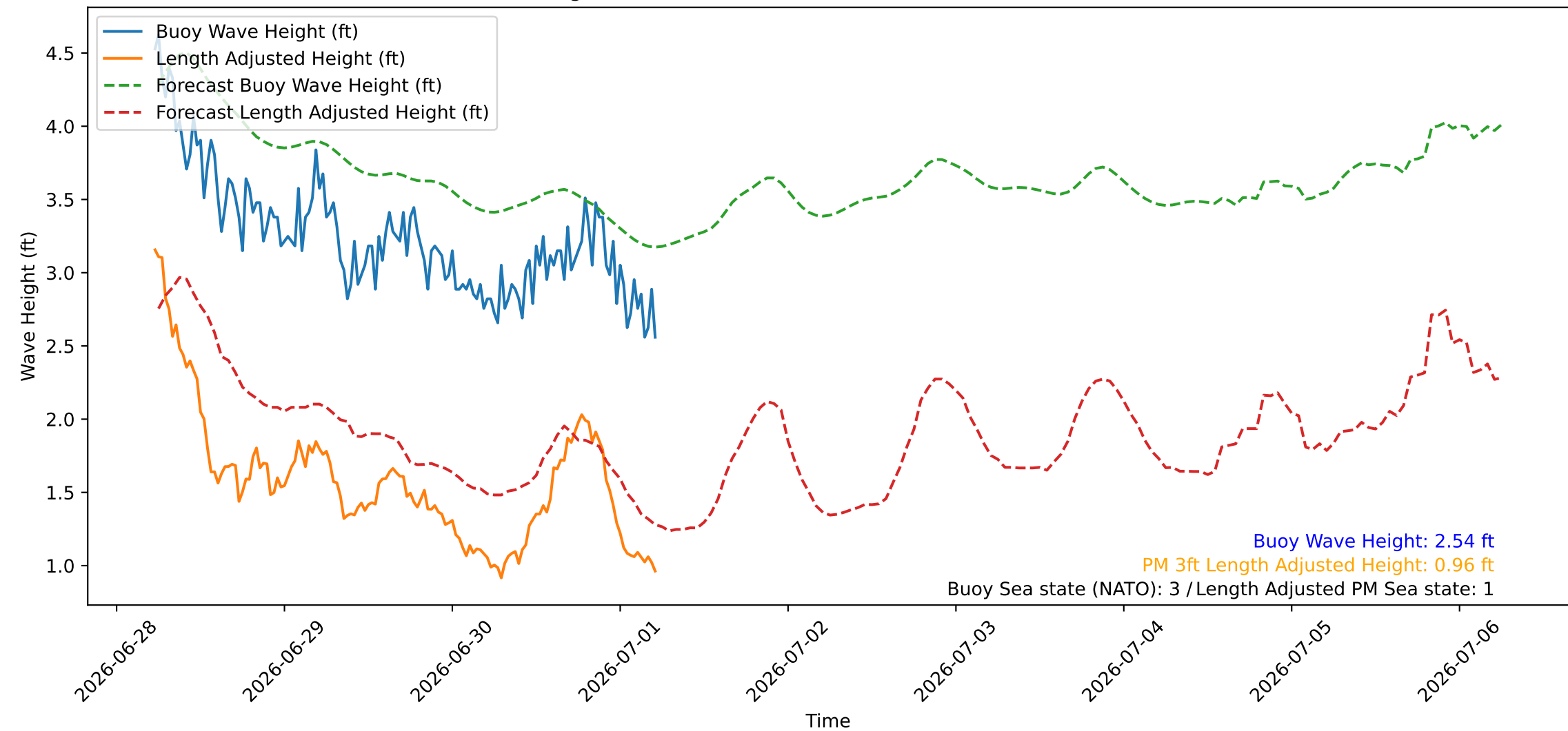
Wave Heights over Time for Green Beach at 2026-07-01 05:41:09
