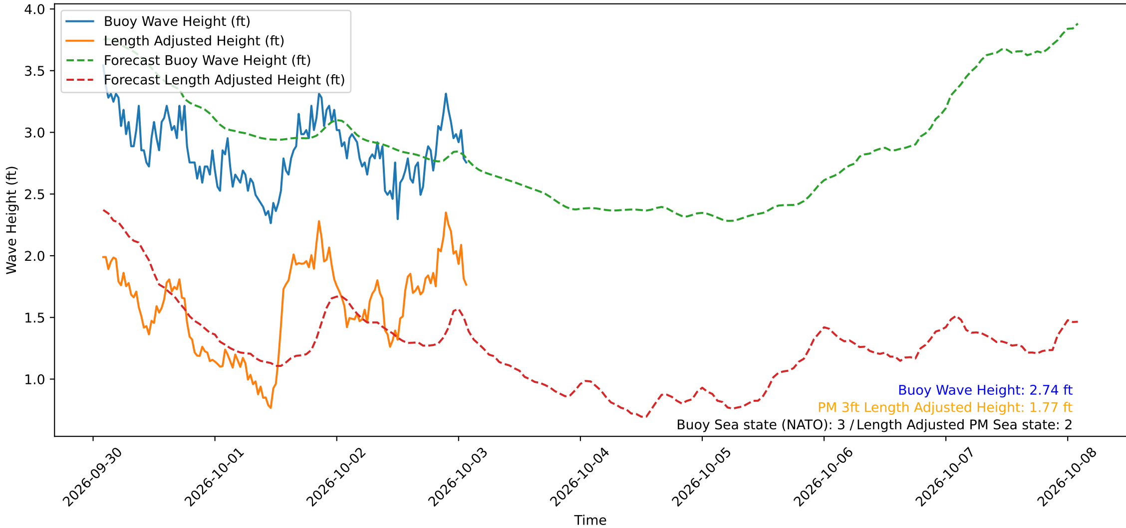
Wave Heights over Time for Oceanside Harbor at 2026-10-03 02:10:50
