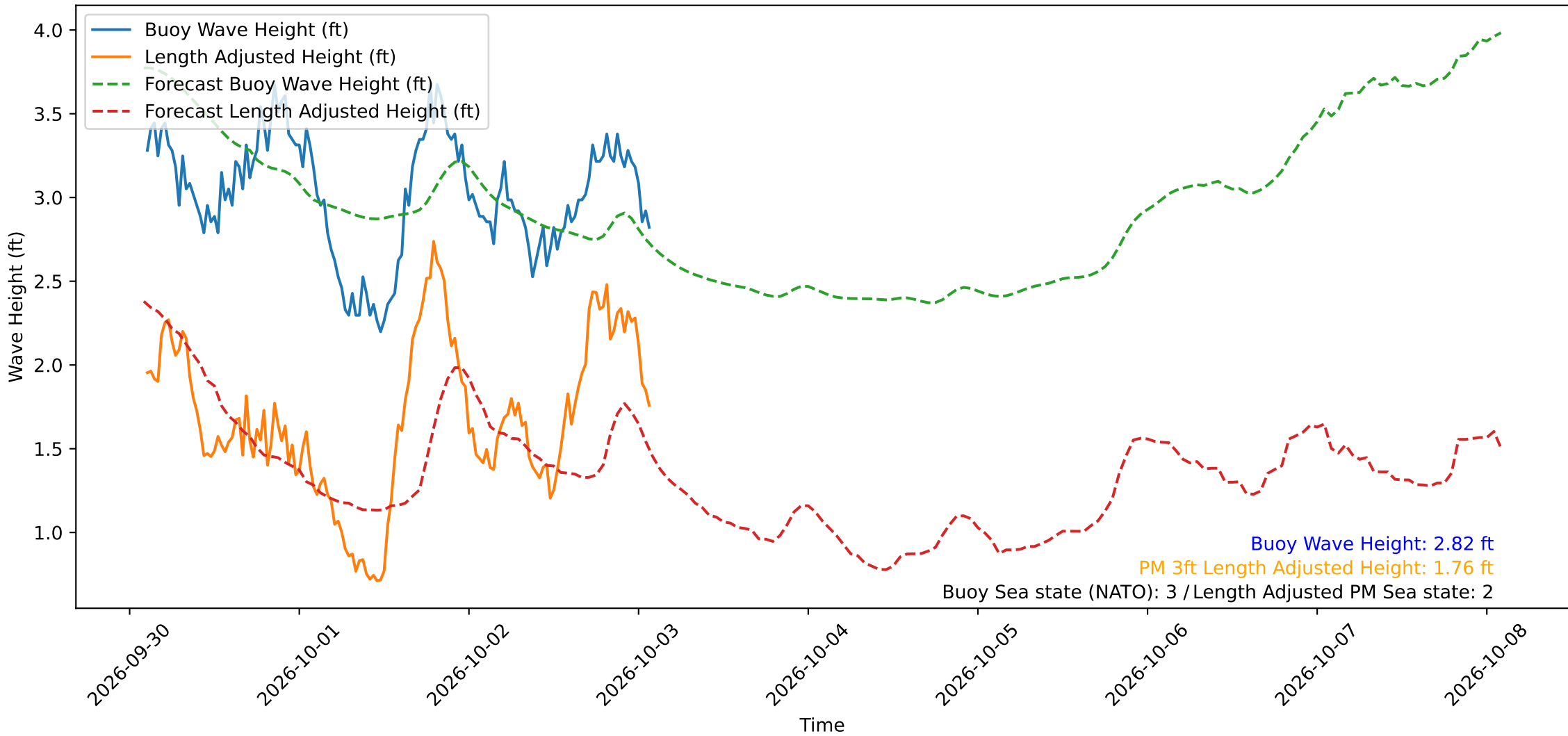
Wave Heights over Time for Green Beach at 2026-10-03 02:11:33
