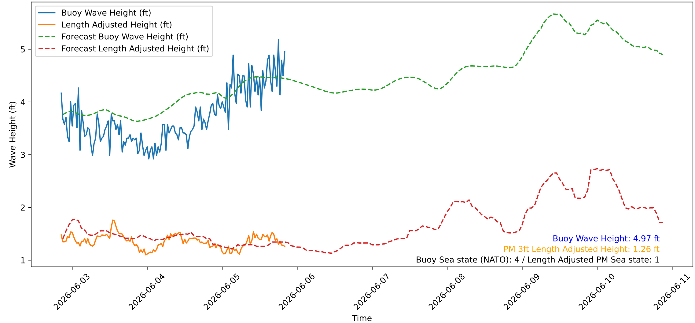
Wave Heights over Time for Oceanside Harbor at 2026-06-05 20:40:26
