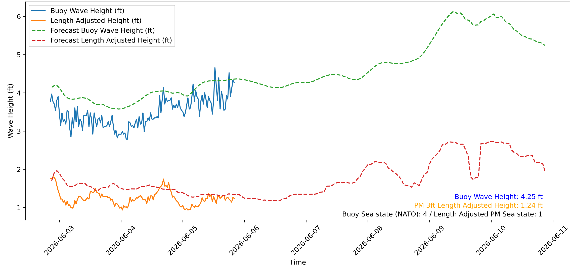
Wave Heights over Time for Green Beach at 2026-06-05 20:41:08
