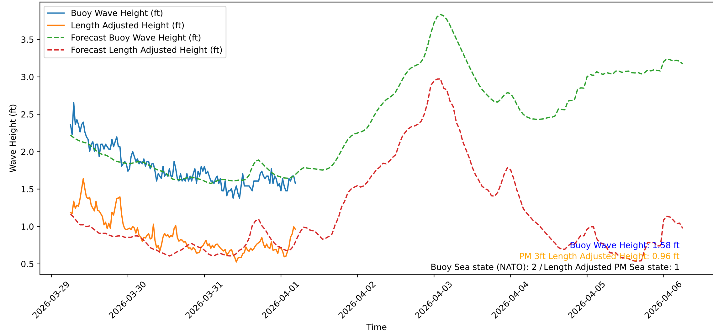
Wave Heights over Time for Red Beach at 2026-04-01 05:30:48
