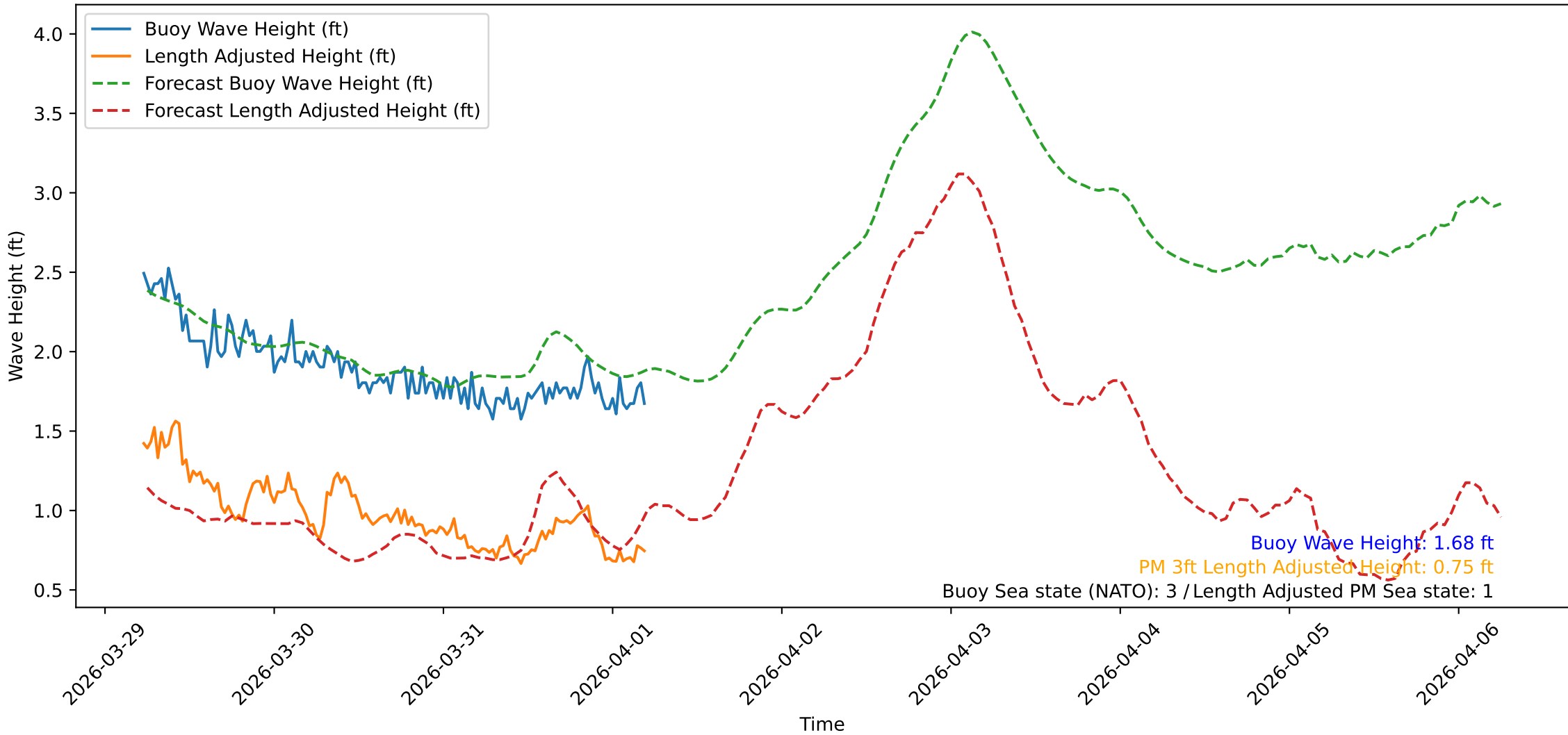
Wave Heights over Time for Oceanside Harbor at 2026-04-01 05:30:32
