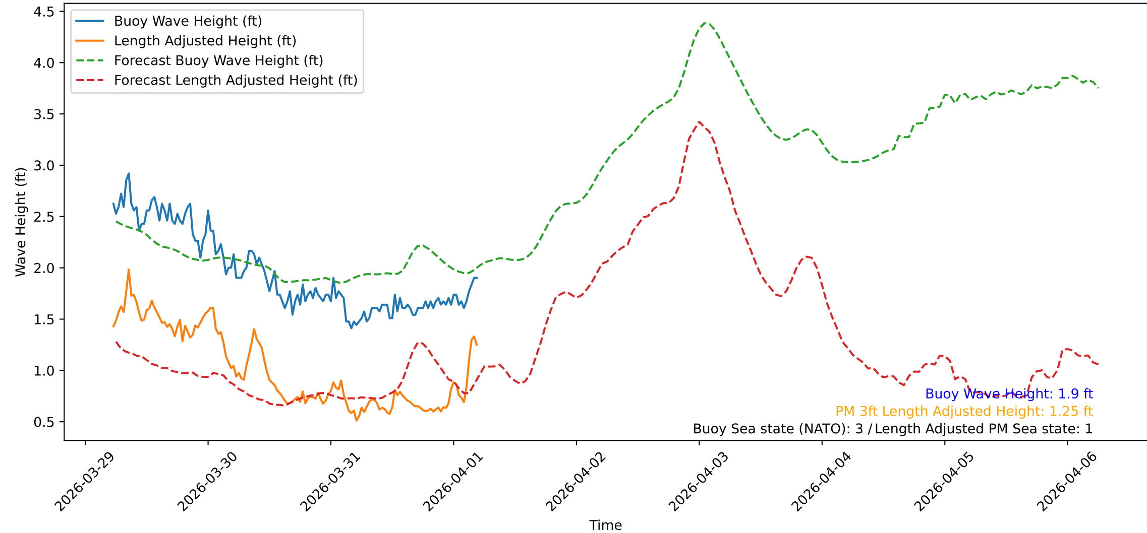
Wave Heights over Time for Green Beach at 2026-04-01 05:31:11
