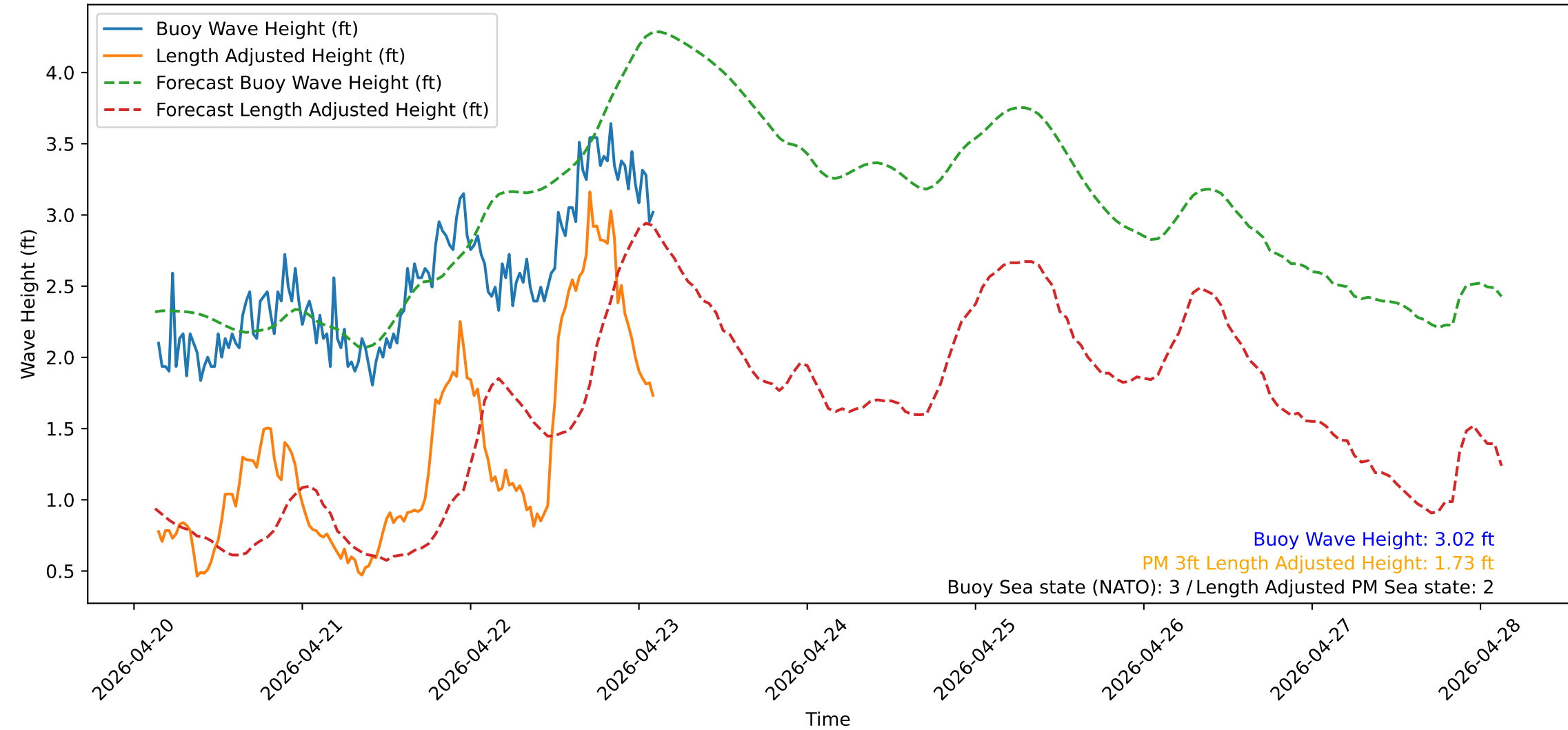
Wave Heights over Time for Red Beach at 2026-04-23 03:10:50
