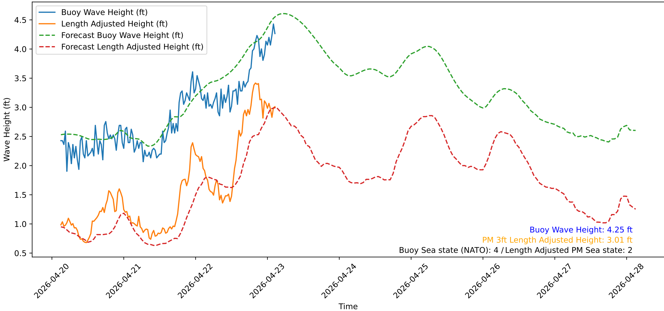
Wave Heights over Time for Oceanside Harbor at 2026-04-23 03:10:31
