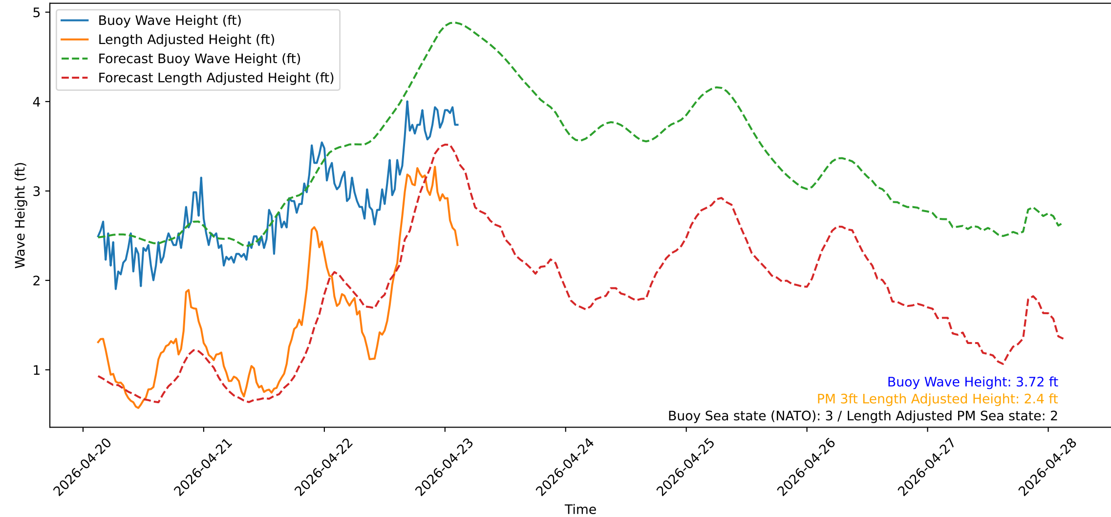
Wave Heights over Time for Green Beach at 2026-04-23 03:11:12
