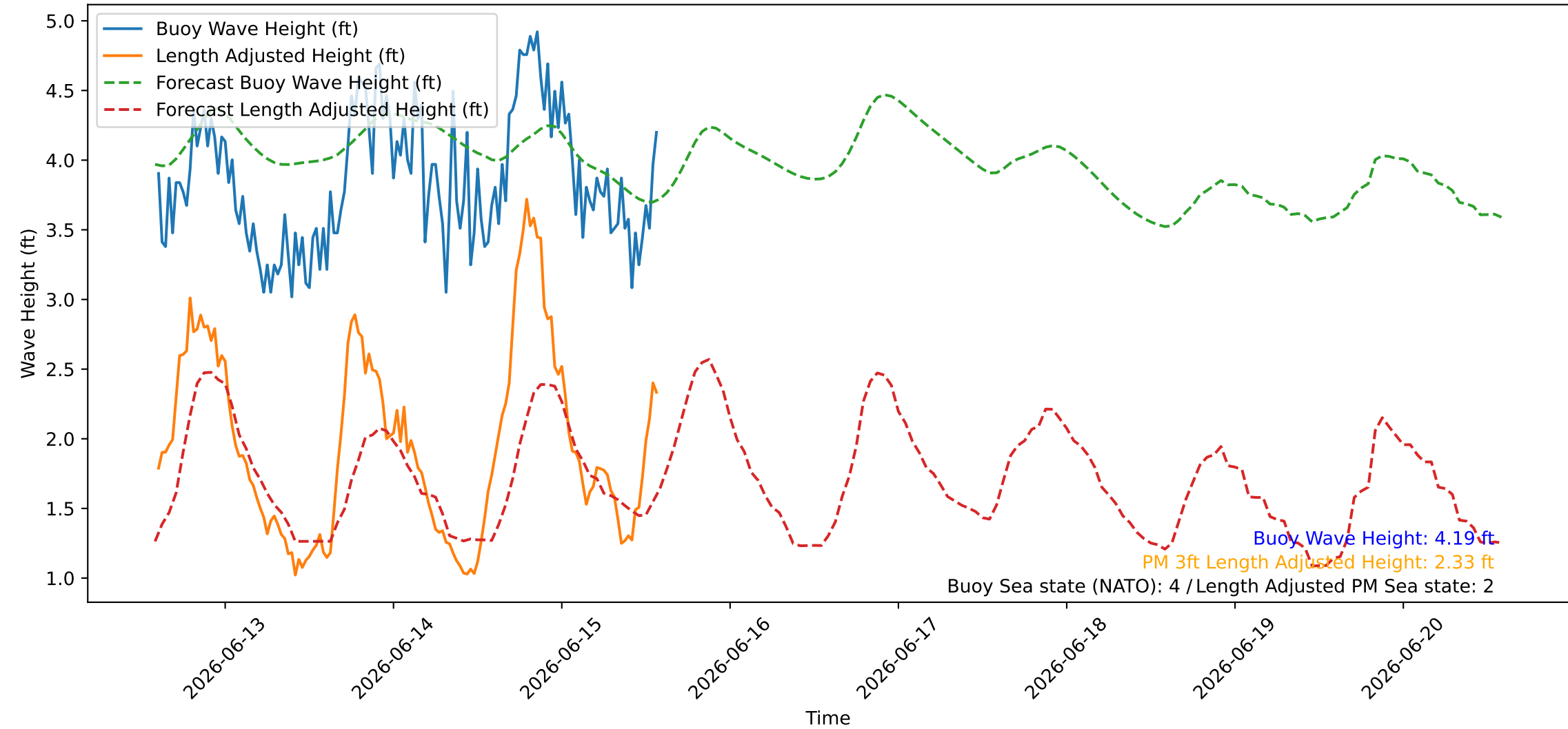
Wave Heights over Time for Green Beach at 2026-06-15 14:21:09
