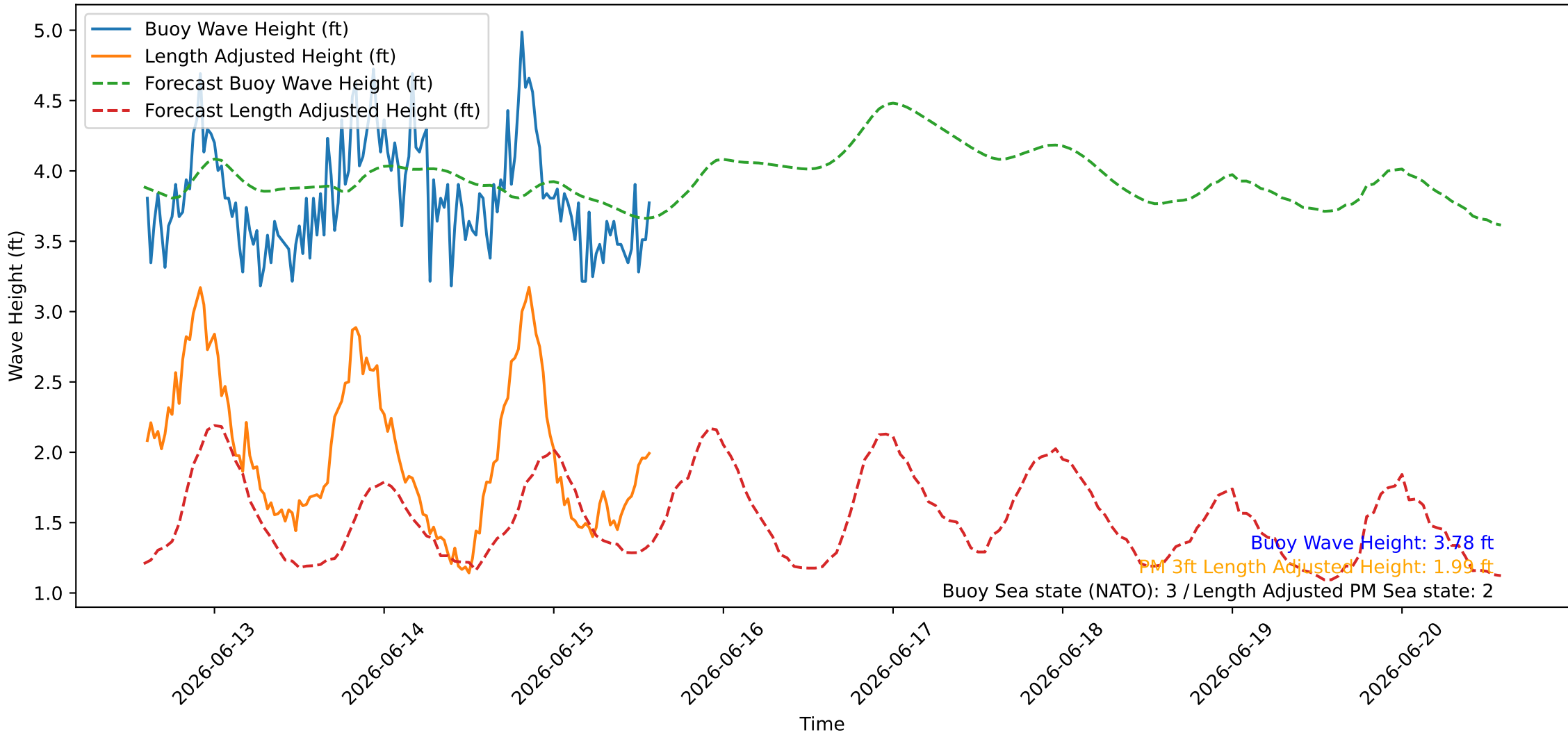
Wave Heights over Time for Oceanside Harbor at 2026-06-15 14:20:26
