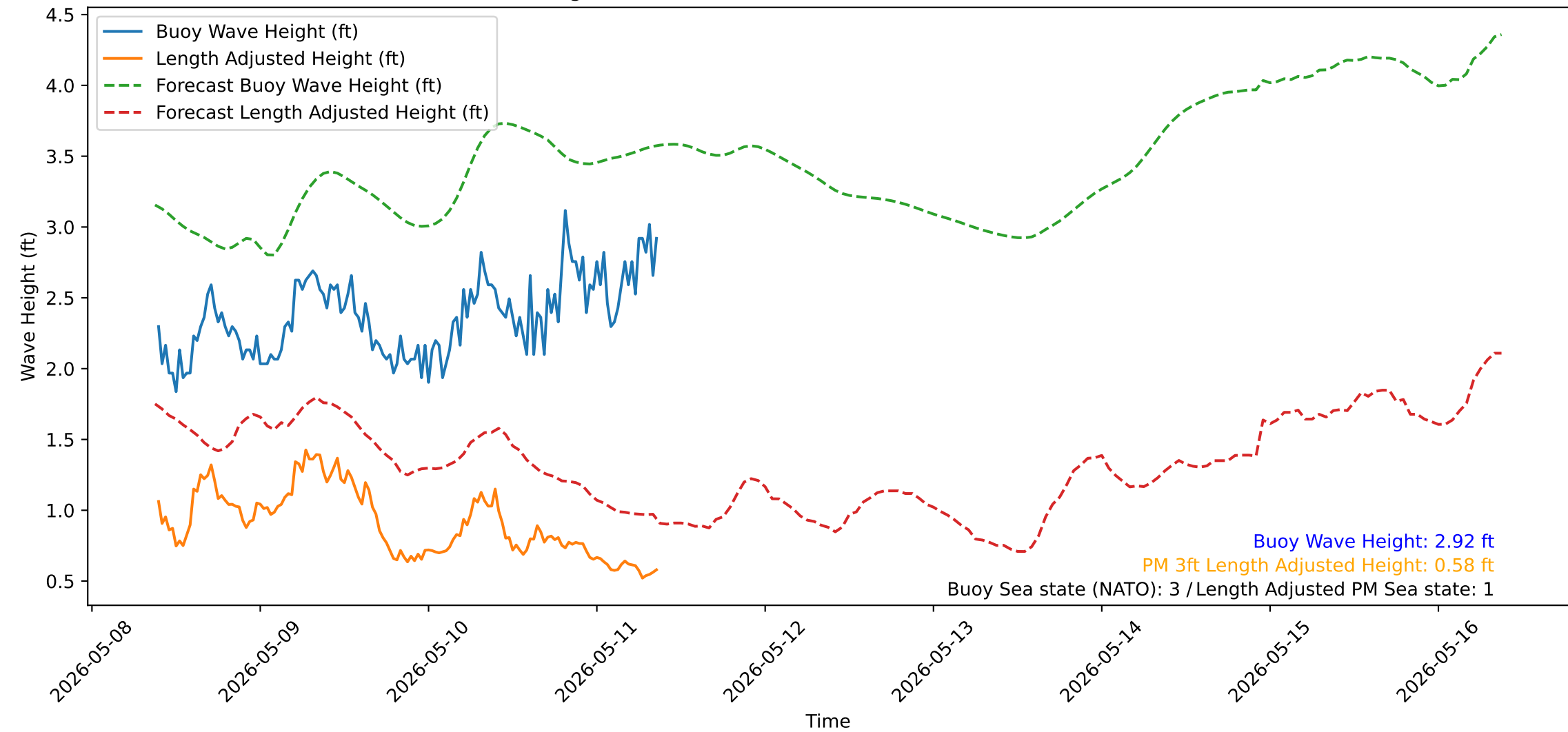
Wave Heights over Time for Green Beach at 2026-05-11 09:21:14
