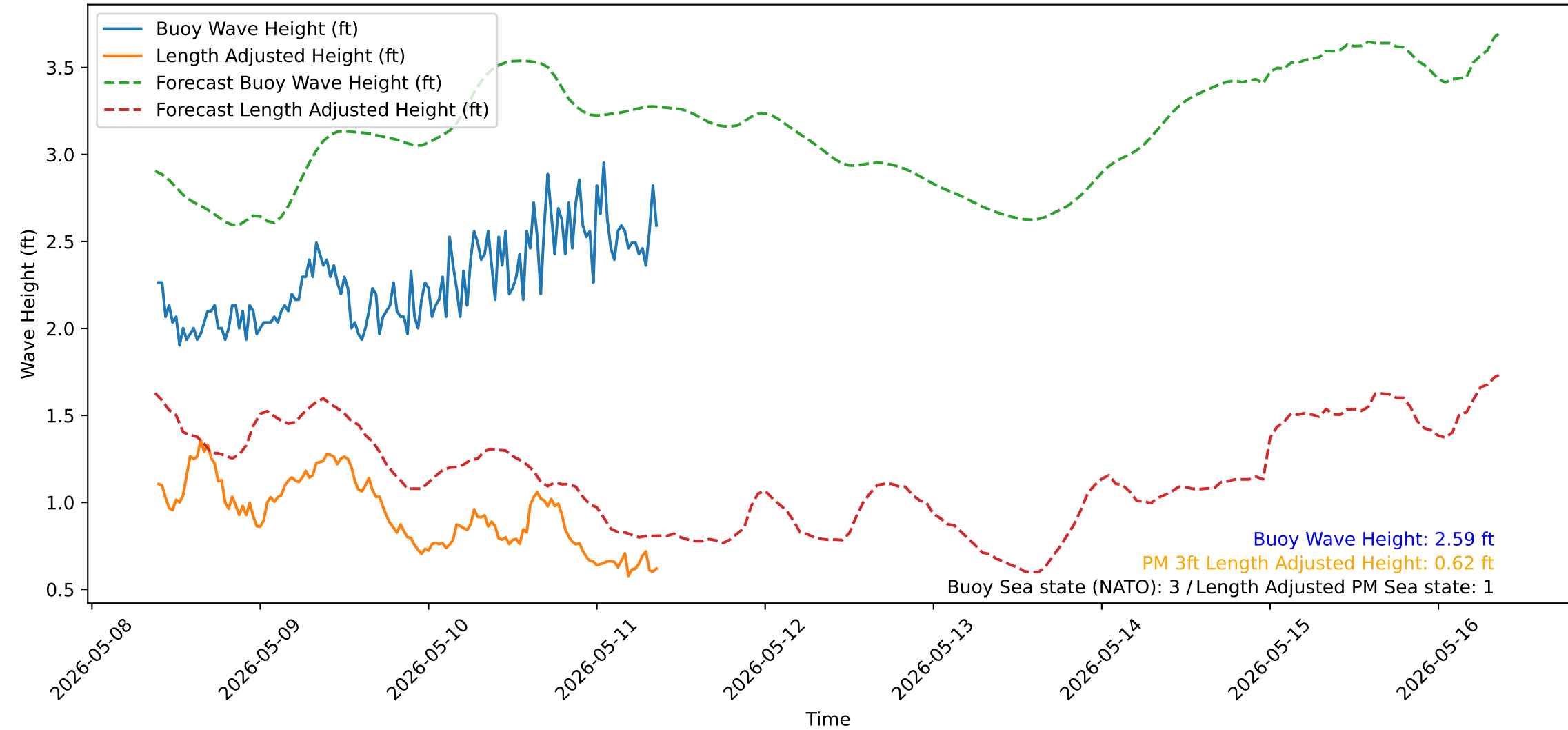
Wave Heights over Time for Red Beach at 2026-05-11 09:20:52
