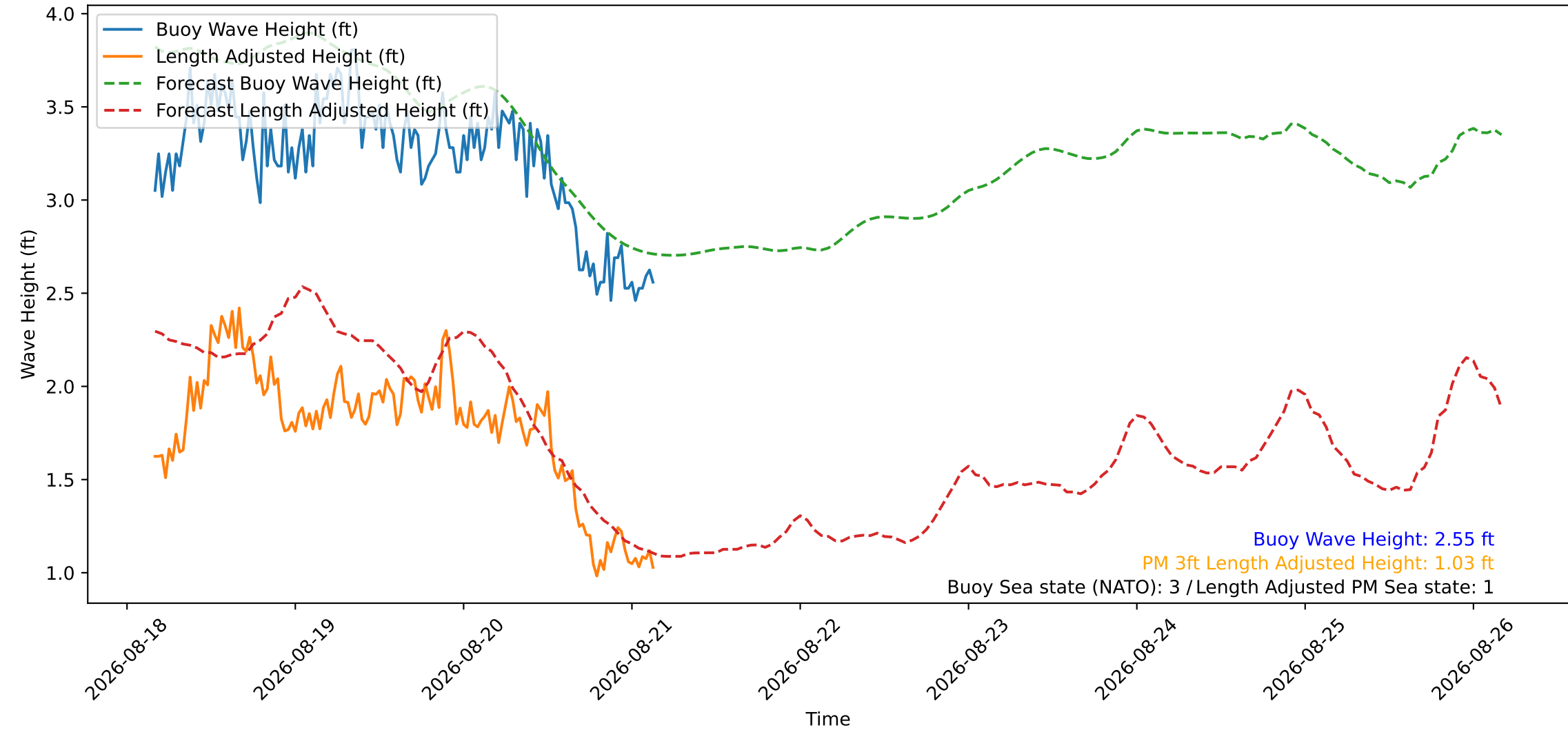
Wave Heights over Time for Oceanside Harbor at 2026-08-21 04:00:26
