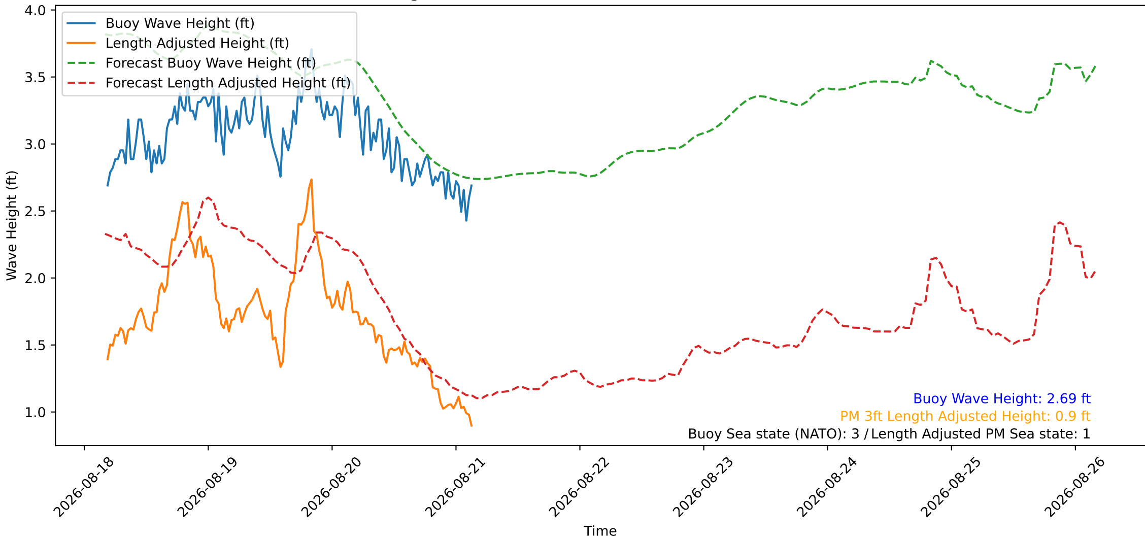
Wave Heights over Time for Green Beach at 2026-08-21 04:01:08
