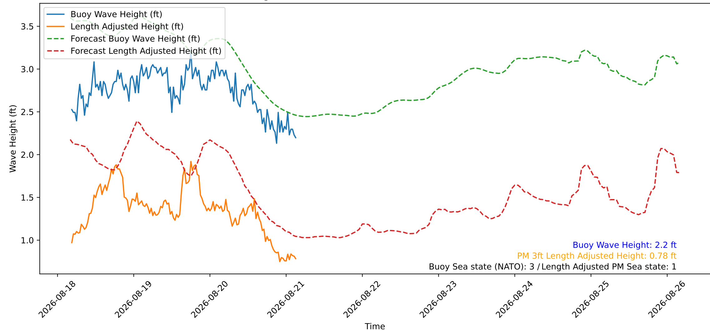
Wave Heights over Time for Red Beach at 2026-08-21 04:00:45
