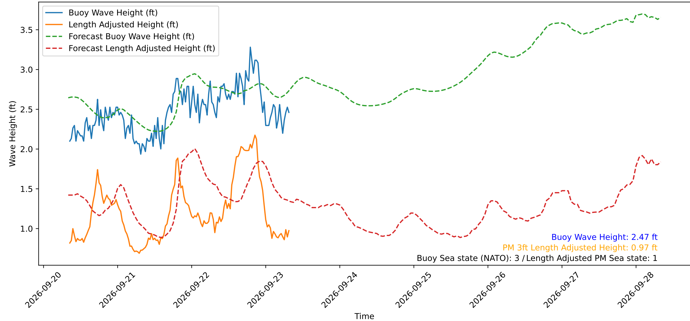
Wave Heights over Time for Red Beach at 2026-09-23 08:20:50
