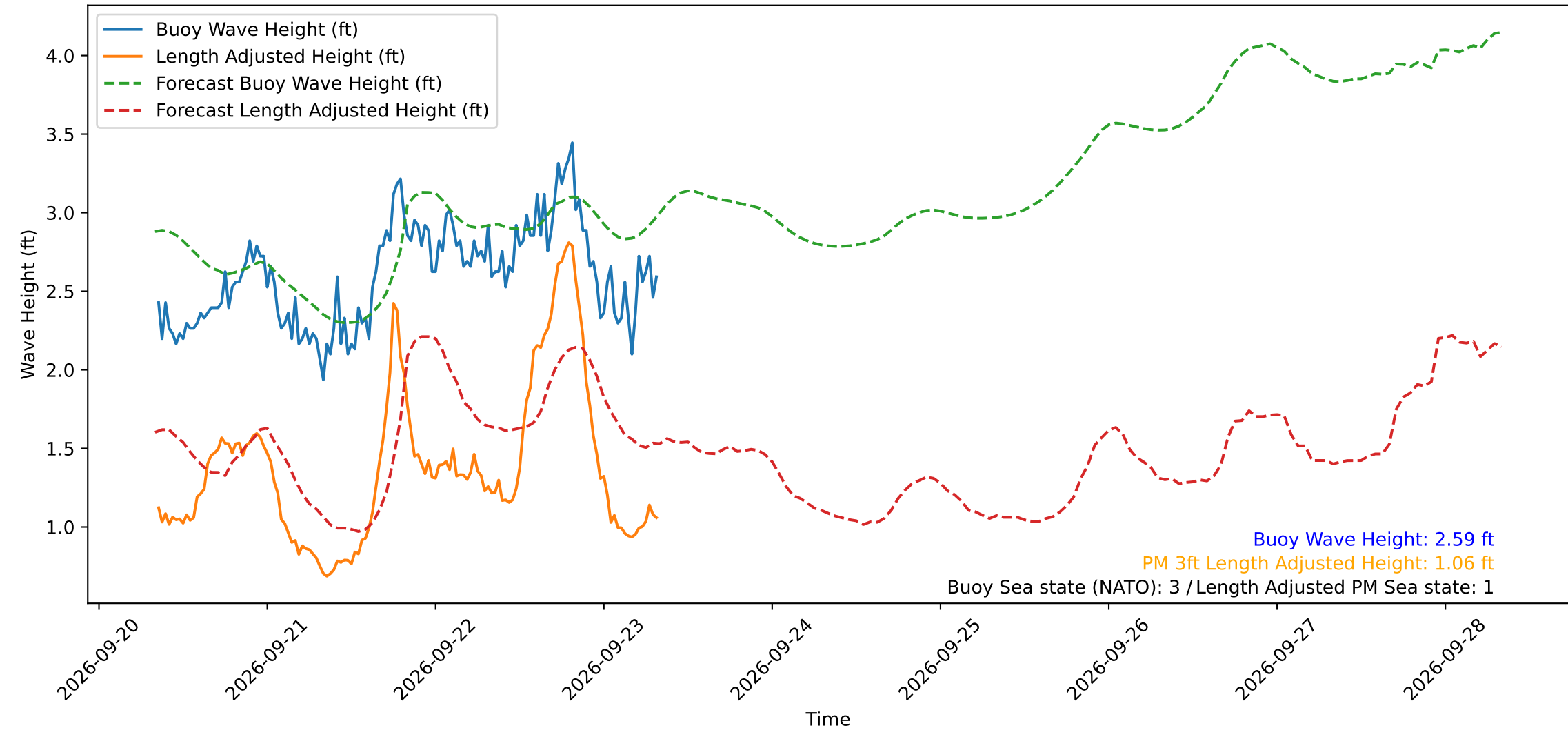
Wave Heights over Time for Green Beach at 2026-09-23 08:21:15
