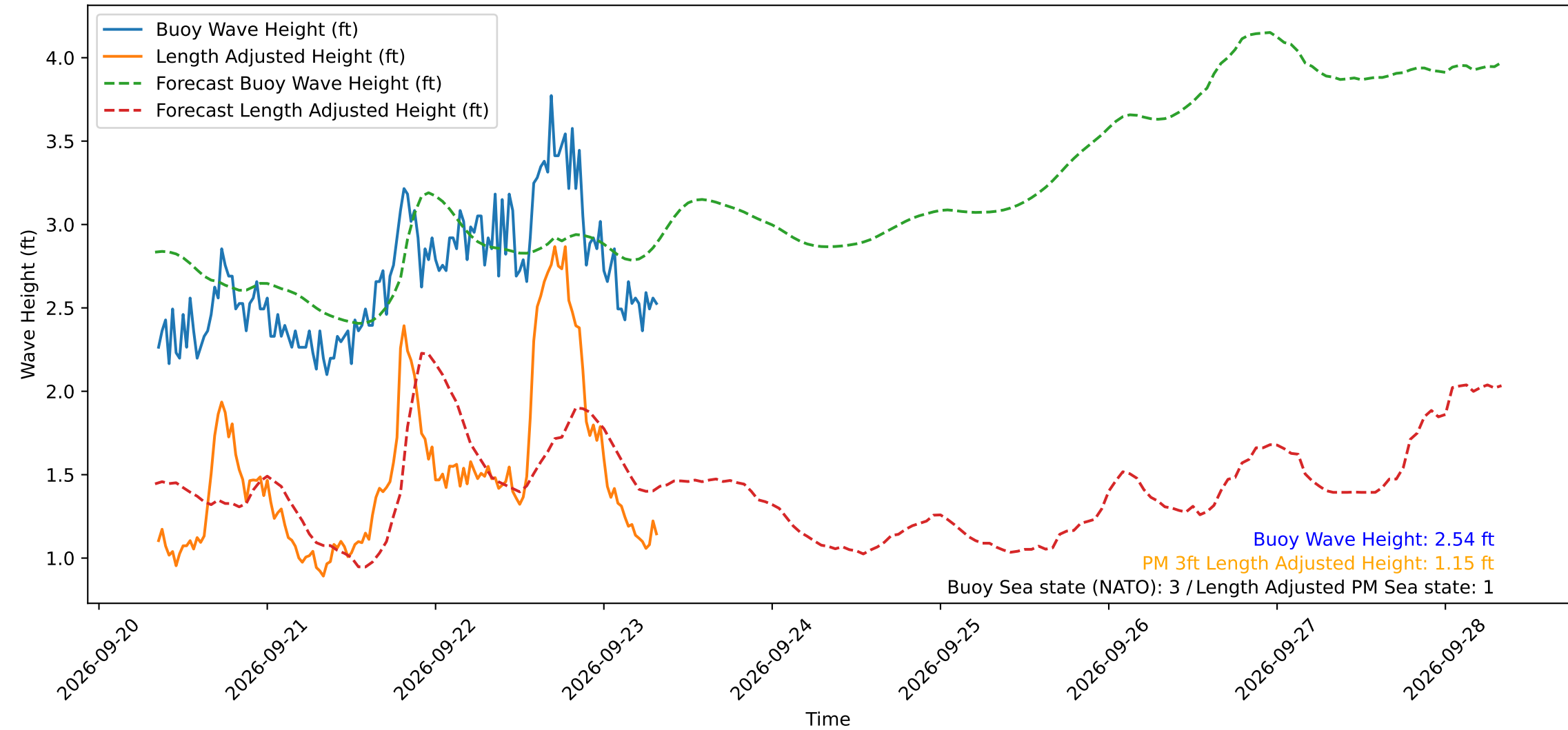
Wave Heights over Time for Oceanside Harbor at 2026-09-23 08:20:30
