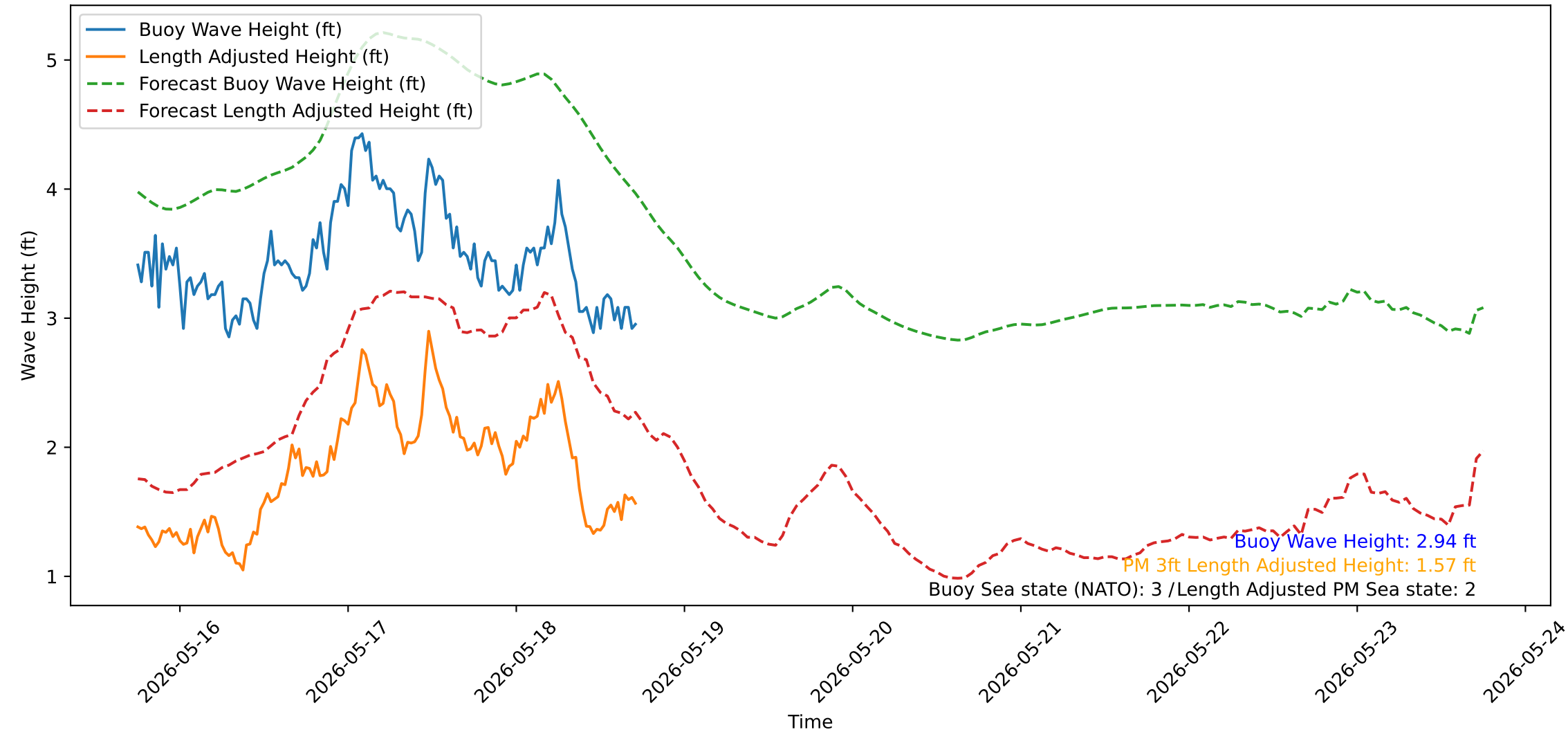
Wave Heights over Time for Green Beach at 2026-05-18 17:51:14
