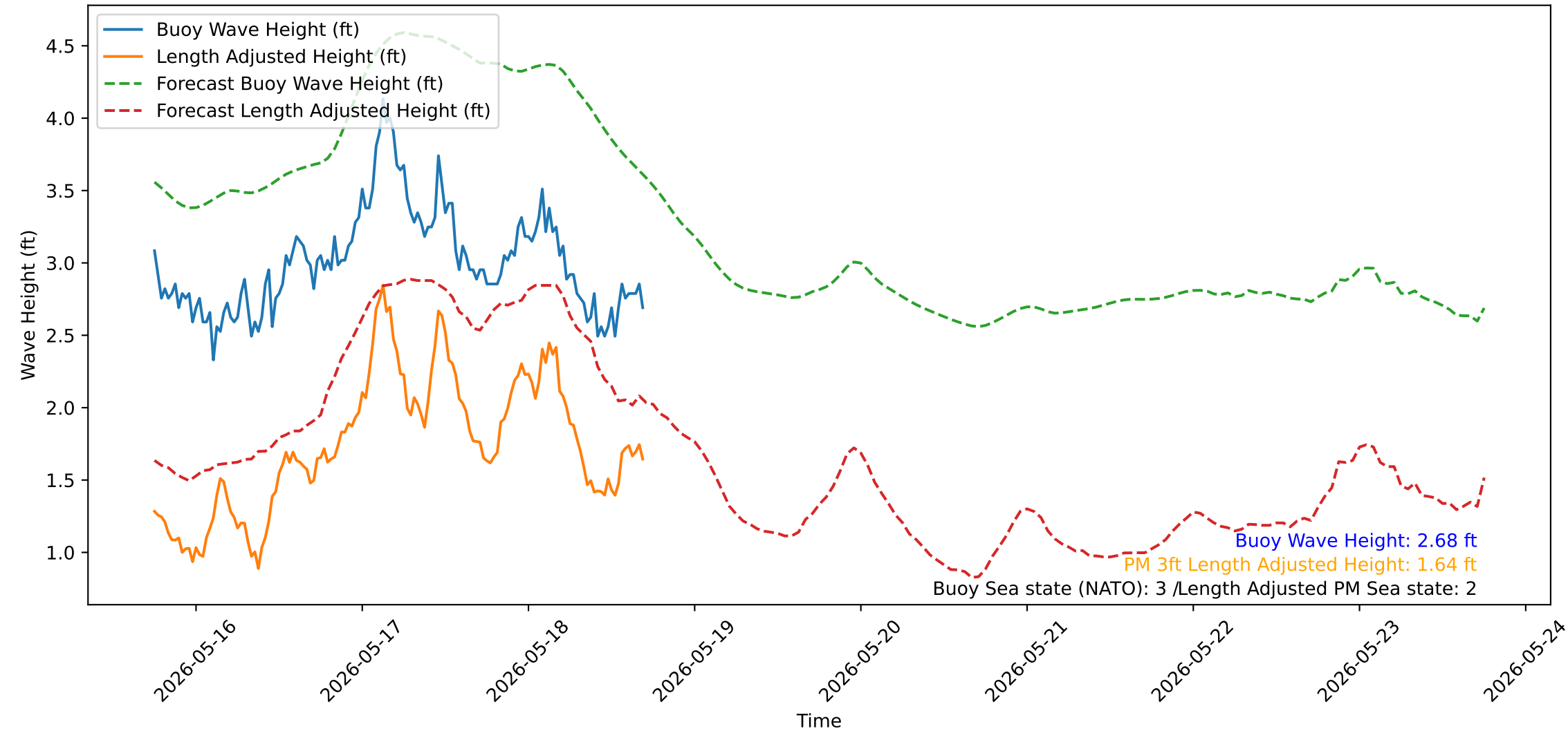
Wave Heights over Time for Red Beach at 2026-05-18 17:50:51
