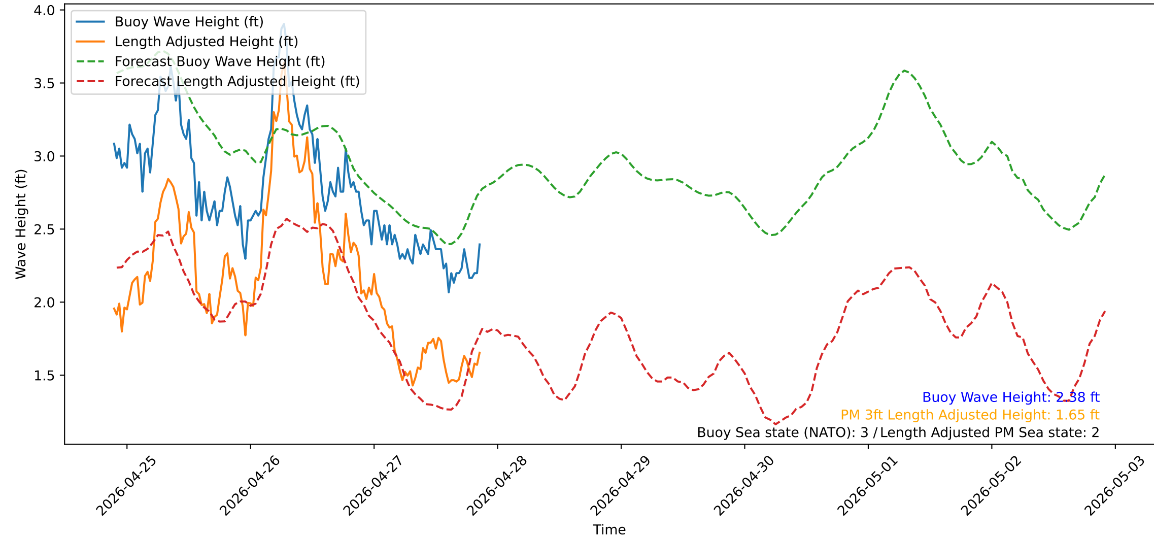
Wave Heights over Time for Oceanside Harbor at 2026-04-27 21:30:31
