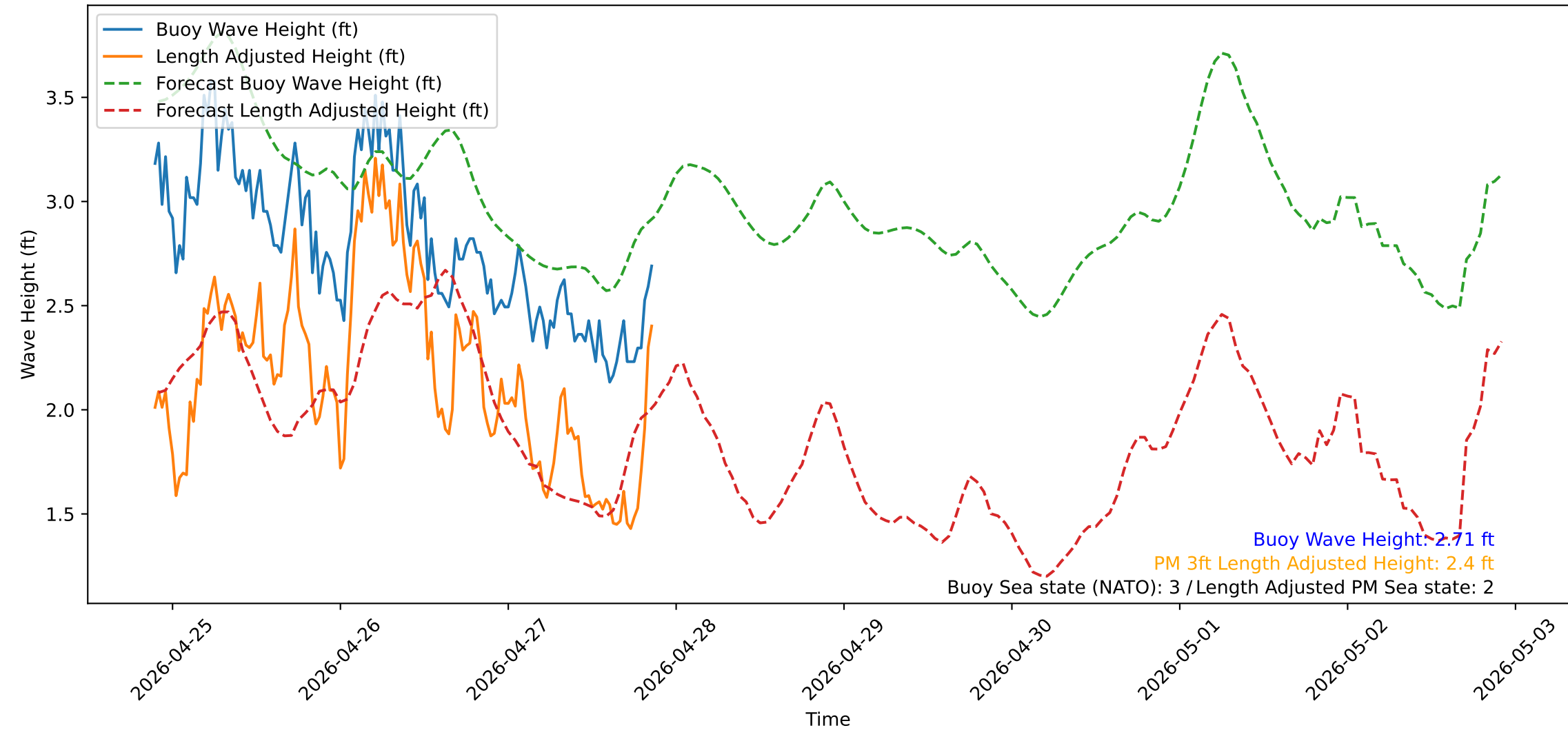
Wave Heights over Time for Green Beach at 2026-04-27 21:31:12
