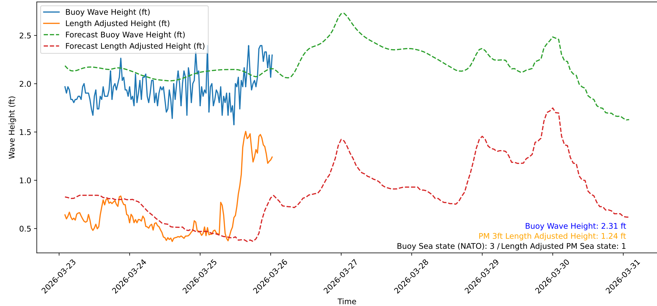
Wave Heights over Time for Red Beach at 2026-03-26 01:30:47
