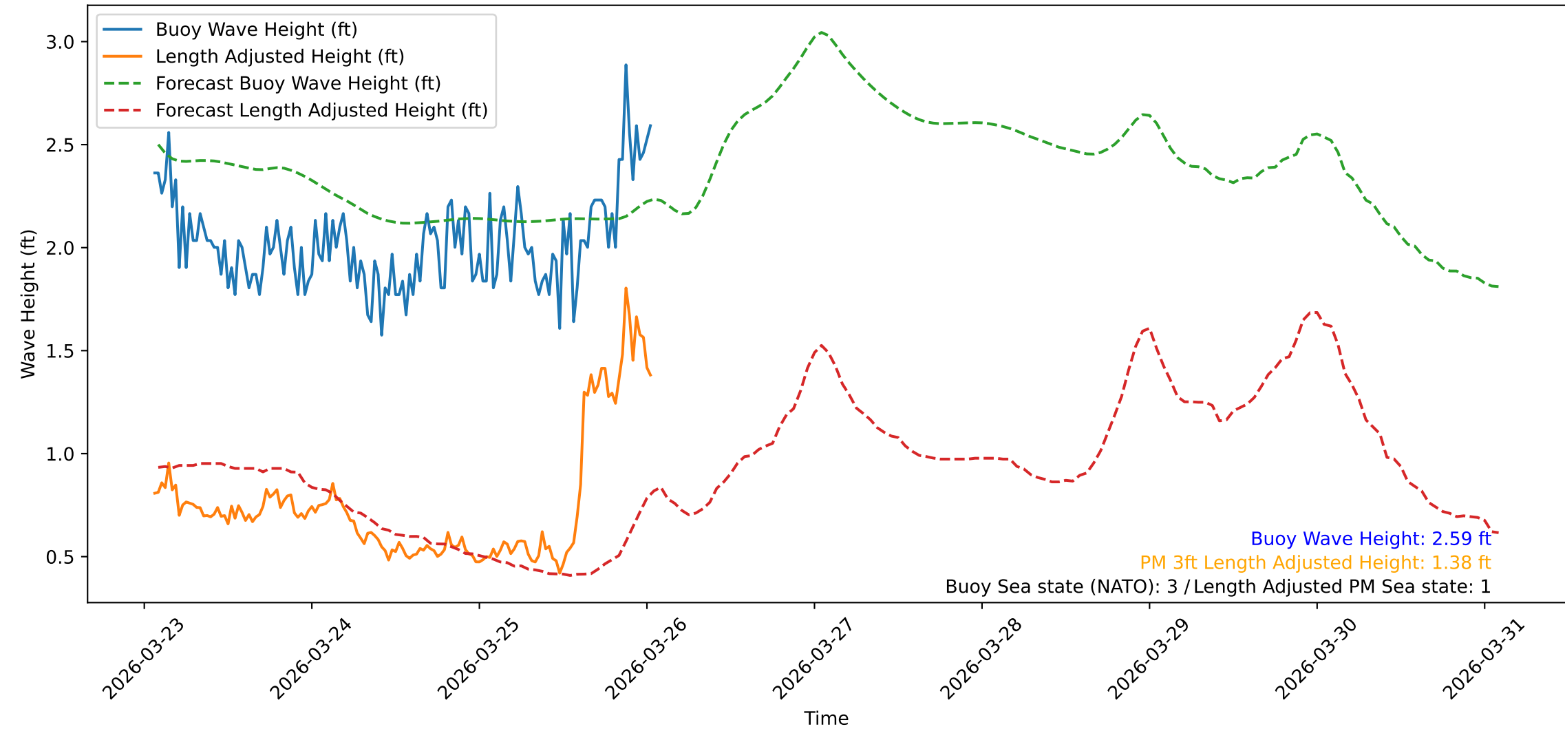
Wave Heights over Time for Oceanside Harbor at 2026-03-26 01:30:32
