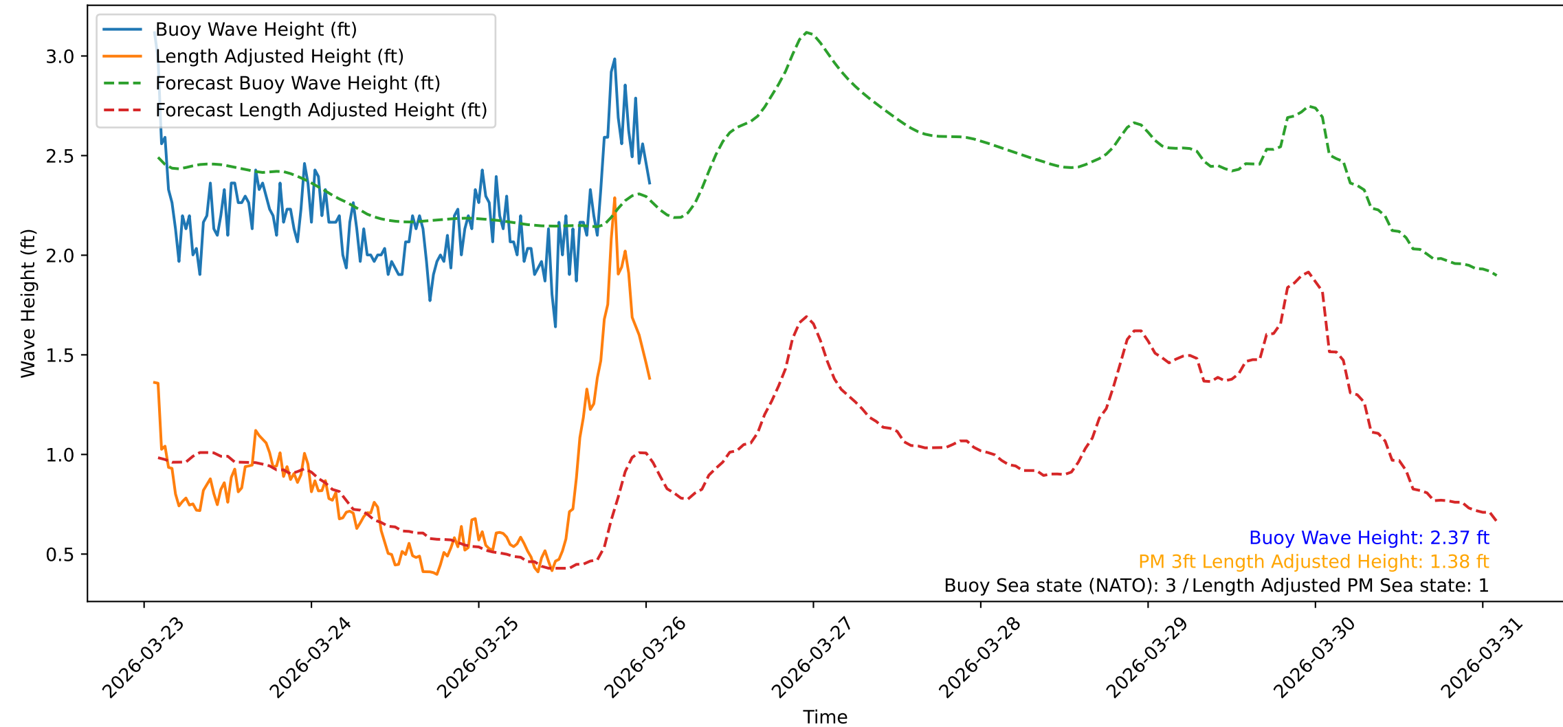
Wave Heights over Time for Green Beach at 2026-03-26 01:31:09
