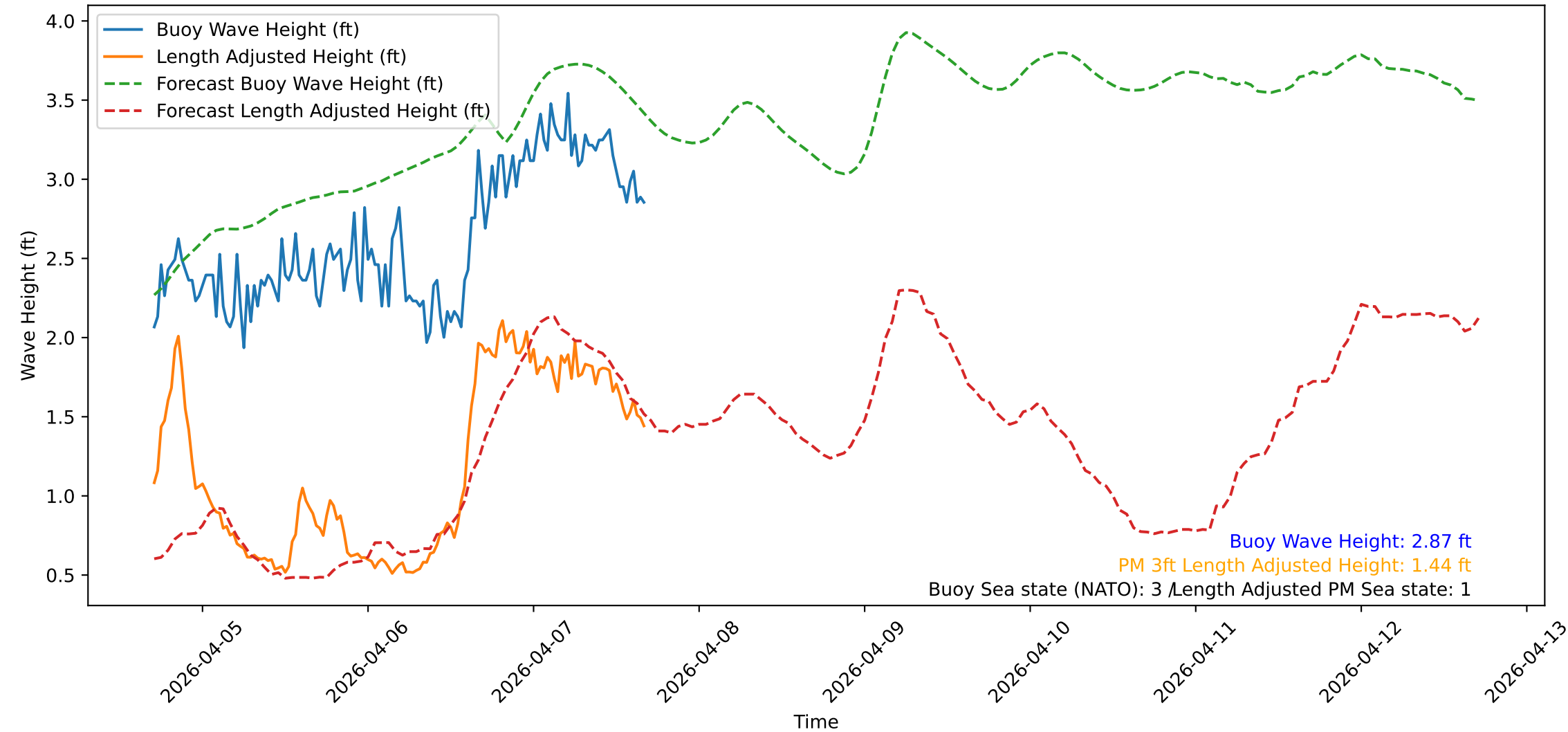
Wave Heights over Time for Red Beach at 2026-04-07 16:40:48
