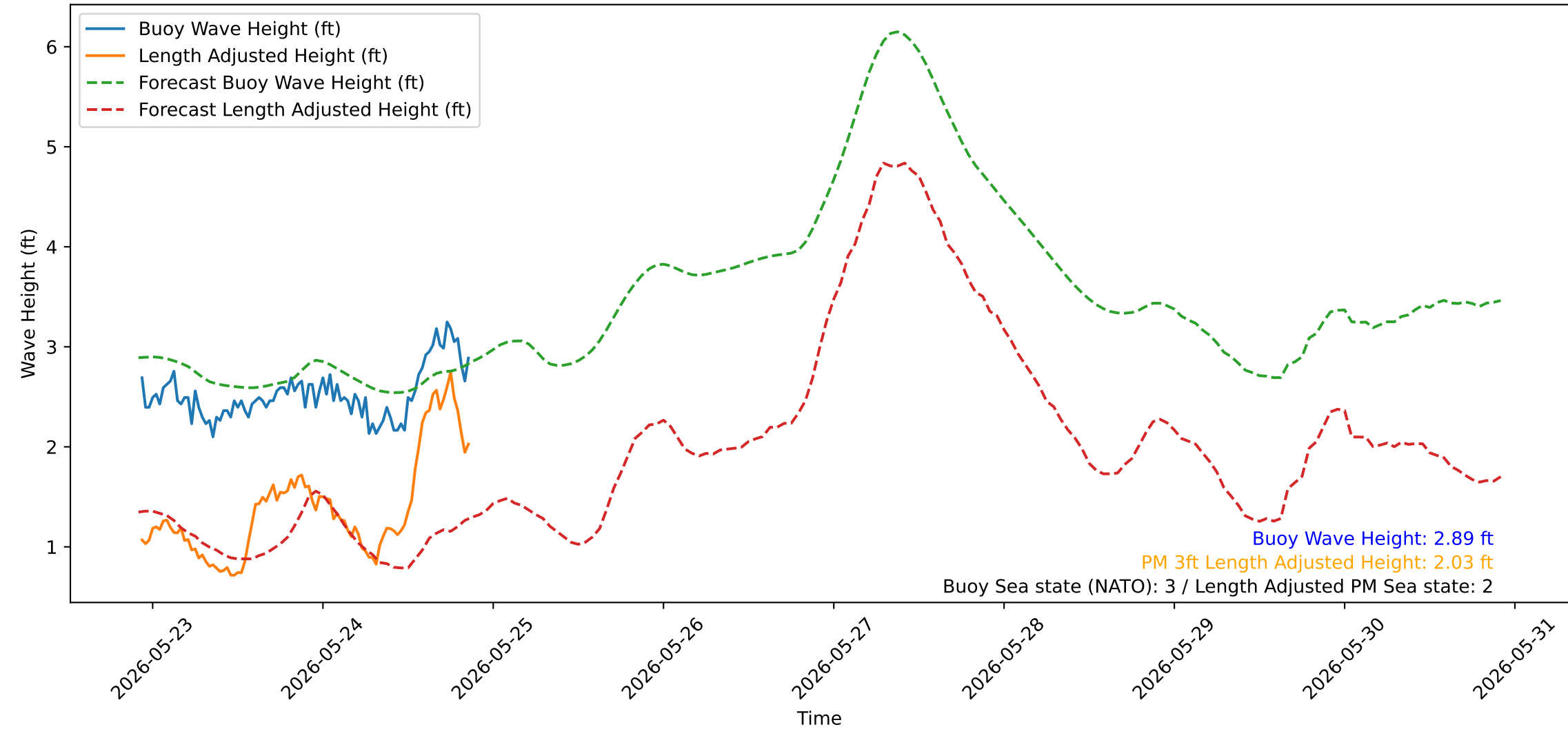
Wave Heights over Time for Oceanside Harbor at 2026-05-25 22:20:29
