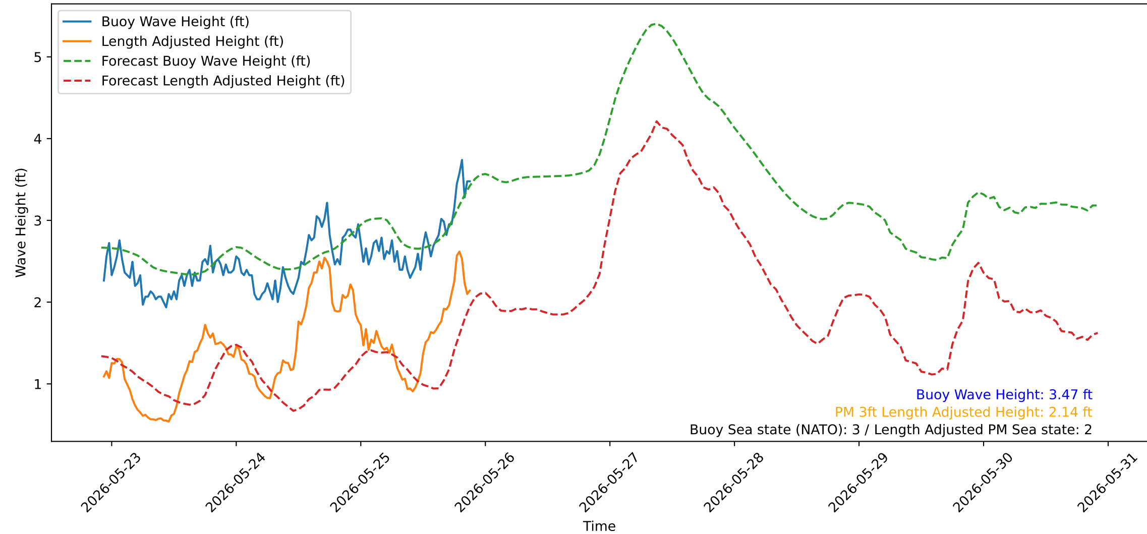
Wave Heights over Time for Red Beach at 2026-05-25 22:20:50
