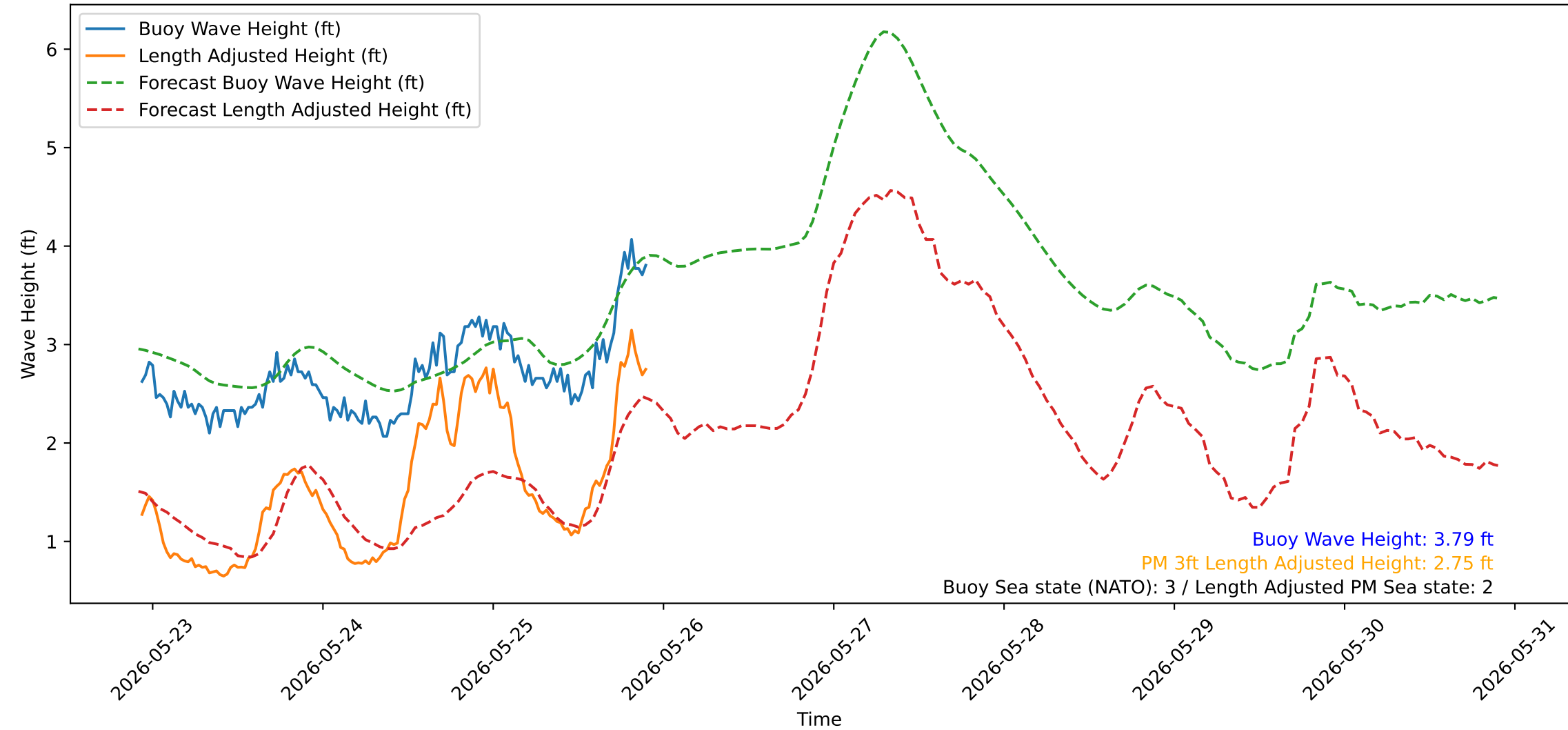
Wave Heights over Time for Green Beach at 2026-05-25 22:21:13
