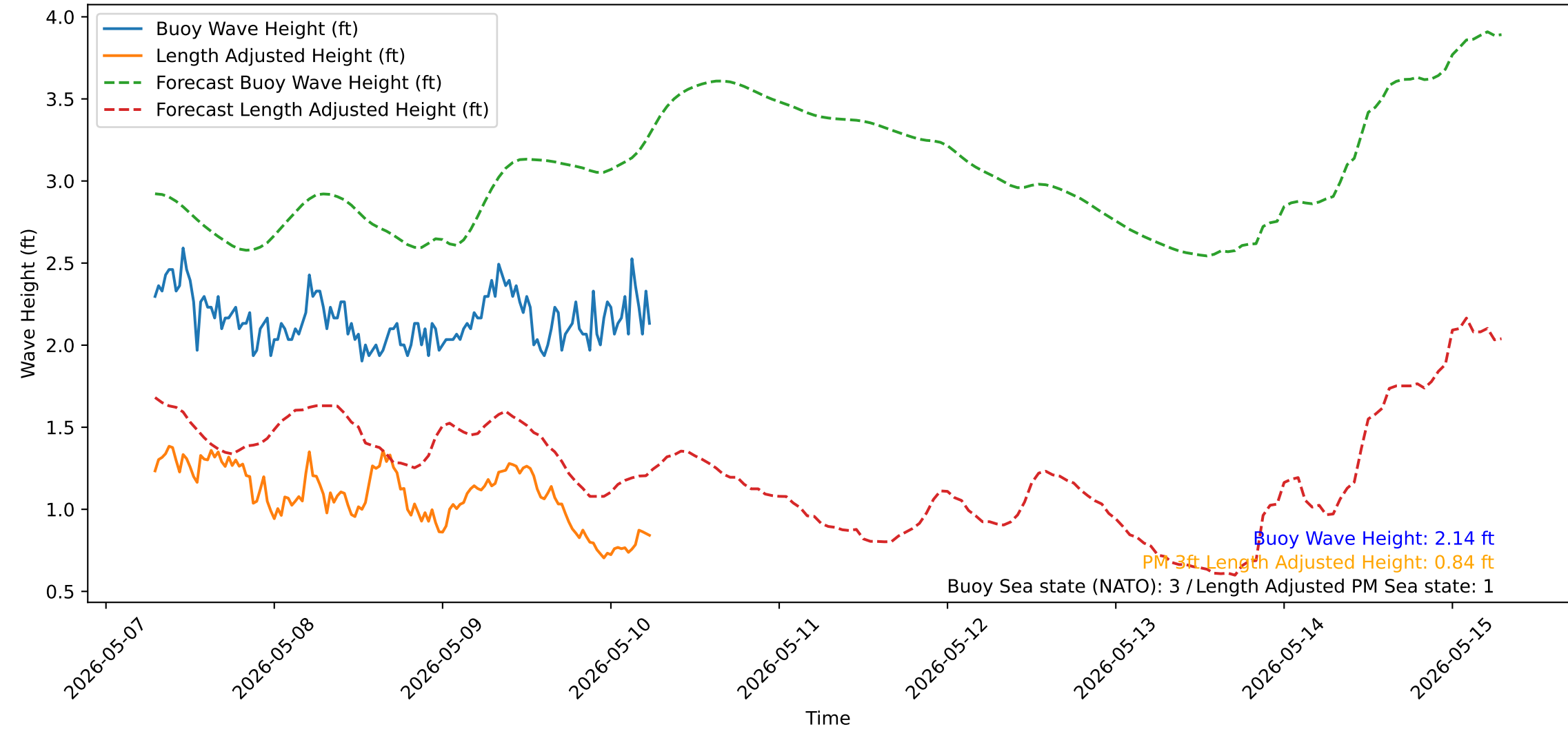
Wave Heights over Time for Red Beach at 2026-05-10 06:30:54
