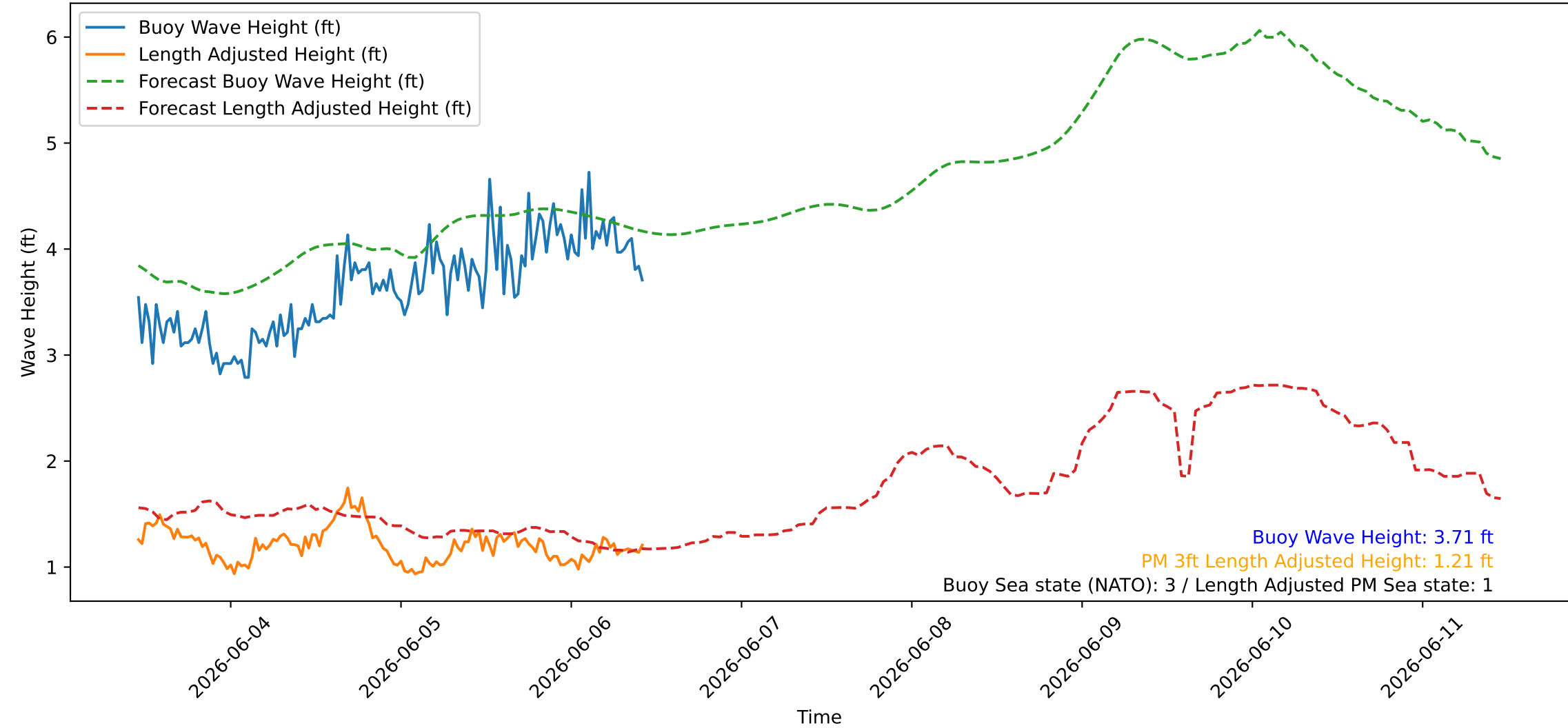
Wave Heights over Time for Green Beach at 2026-06-06 10:51:10
