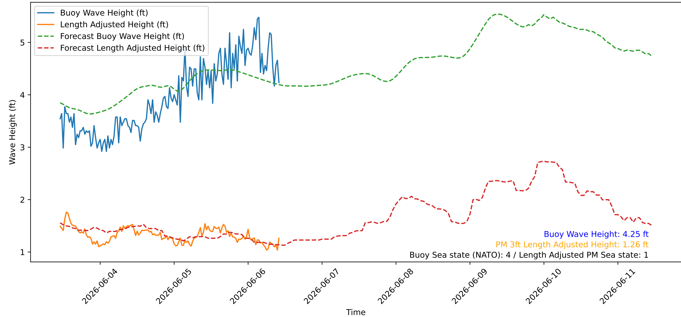
Wave Heights over Time for Oceanside Harbor at 2026-06-06 10:50:27
