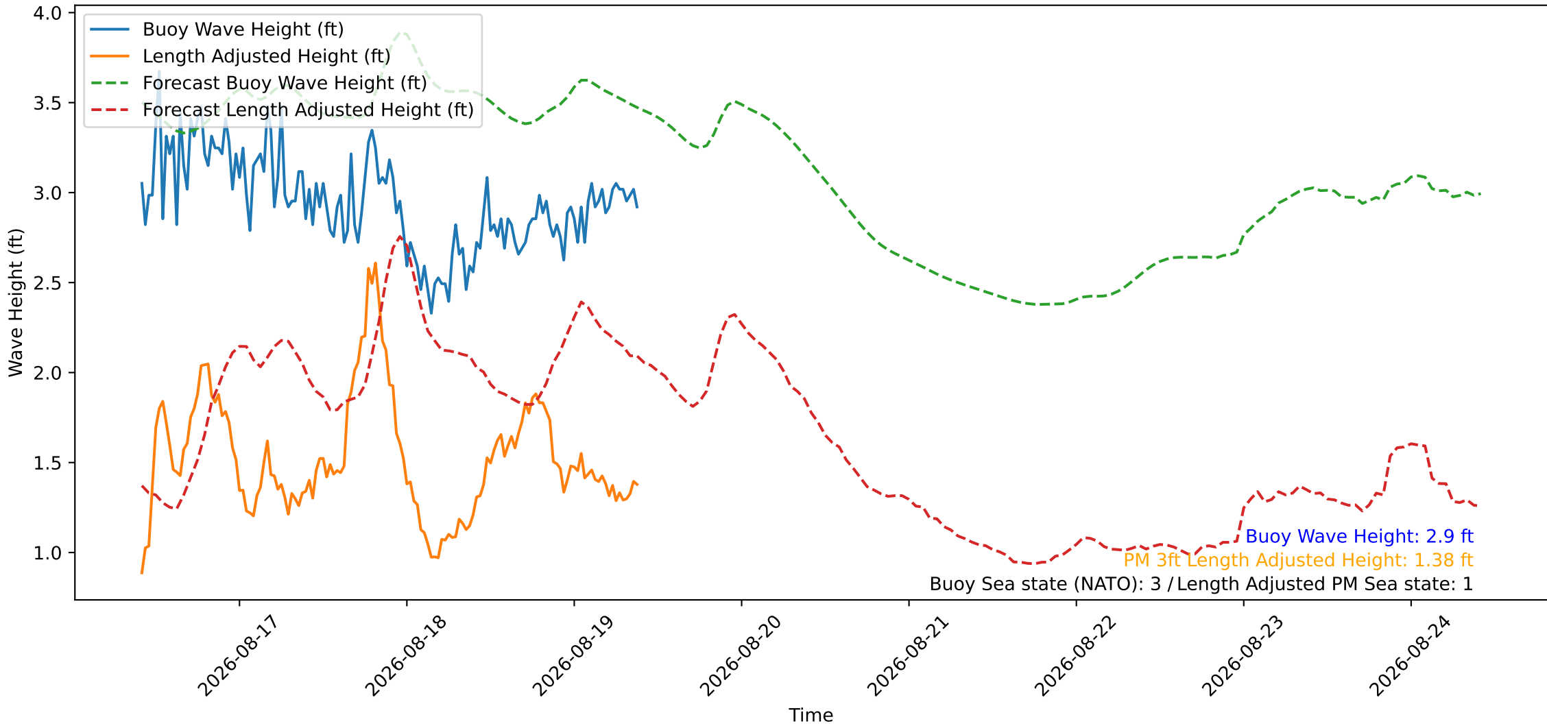
Wave Heights over Time for Red Beach at 2026-08-19 09:40:45
