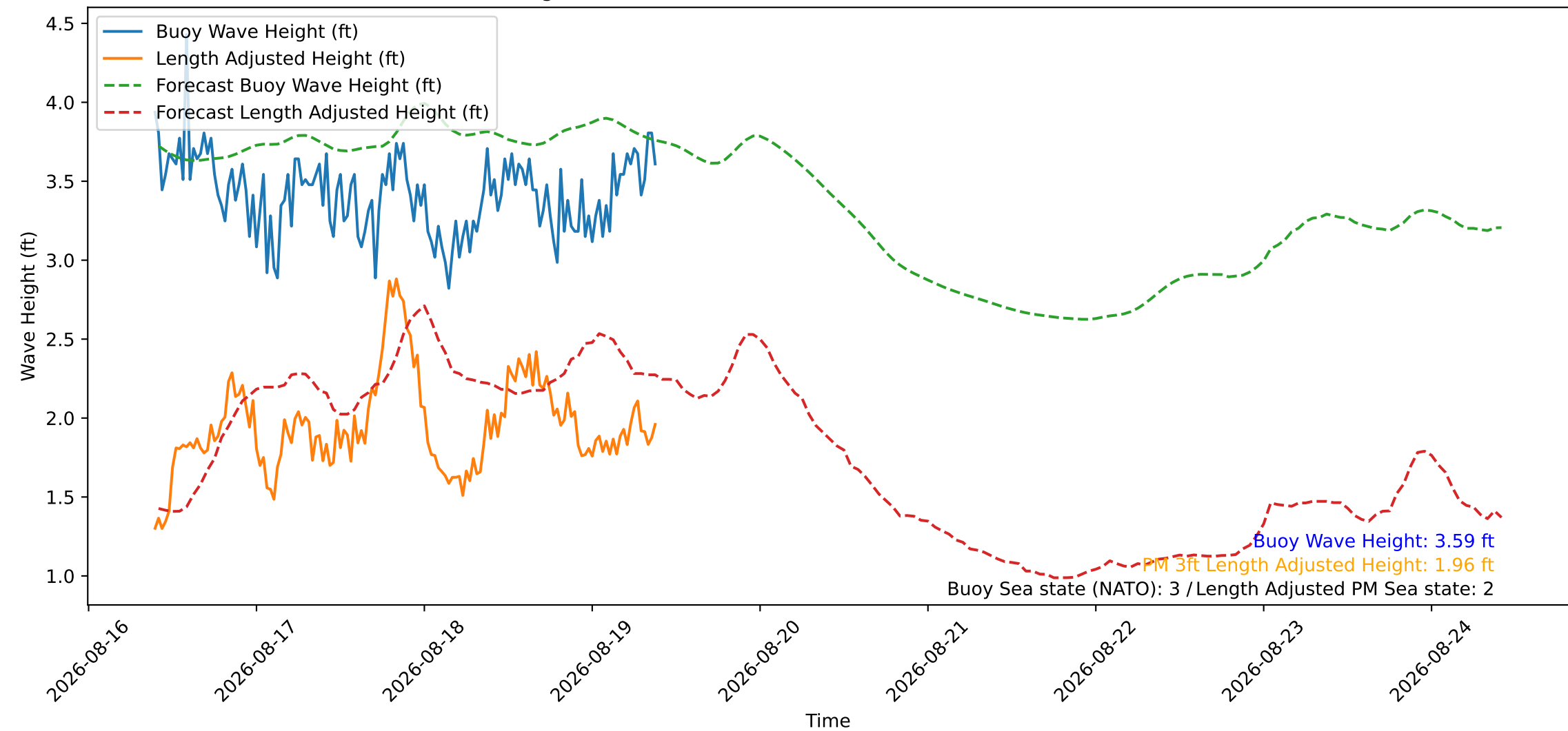
Wave Heights over Time for Oceanside Harbor at 2026-08-19 09:40:26
