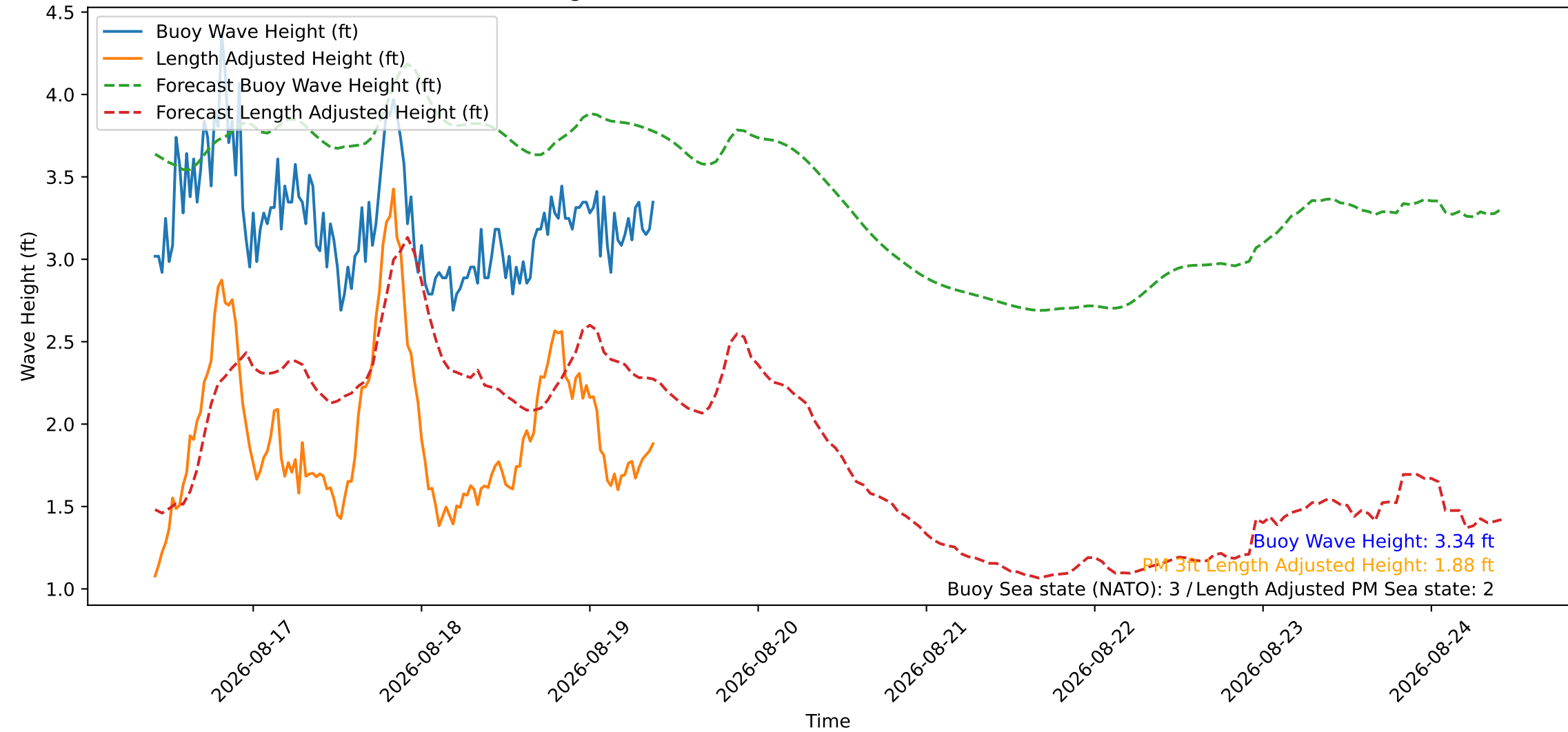
Wave Heights over Time for Green Beach at 2026-08-19 09:41:08
