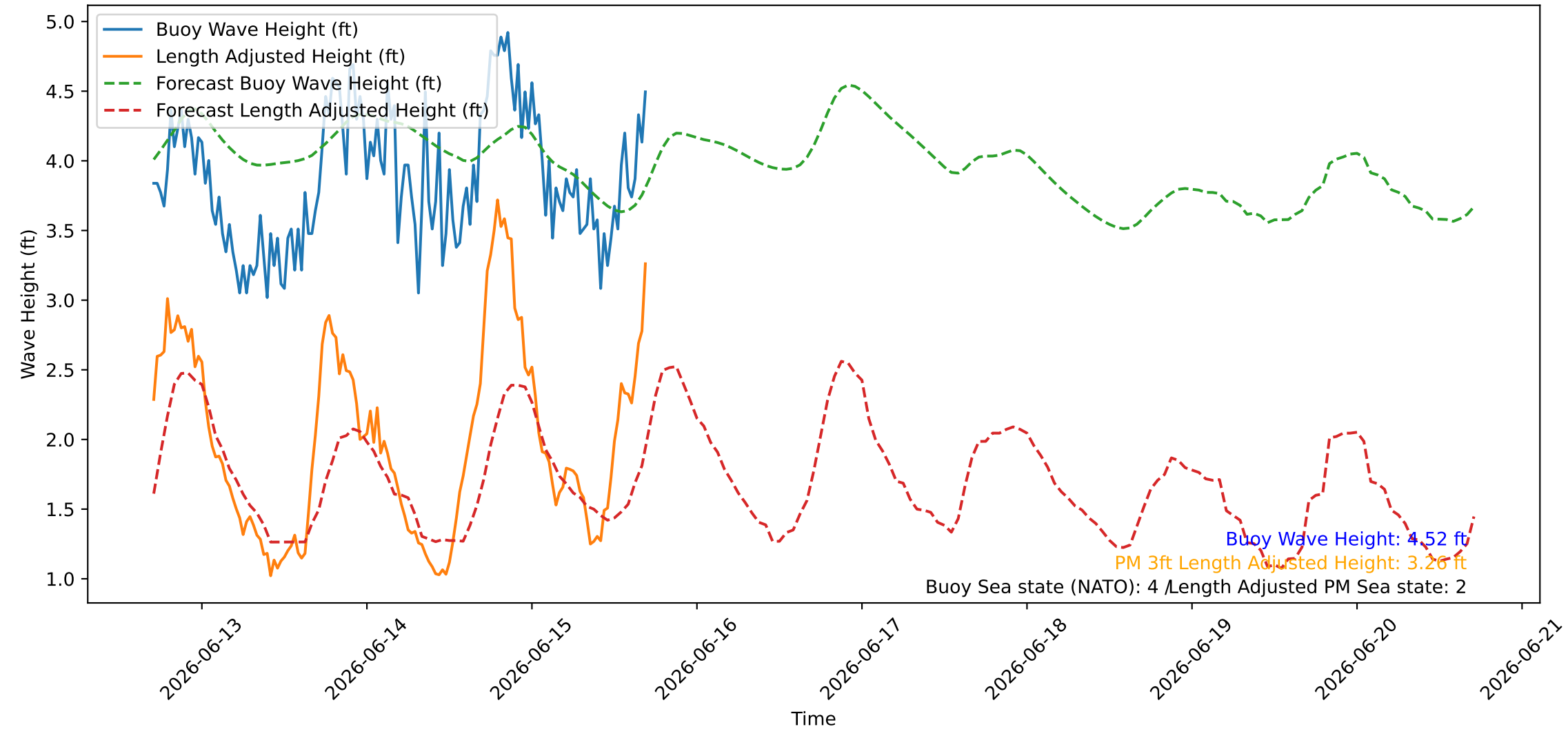
Wave Heights over Time for Green Beach at 2026-06-15 17:11:07
