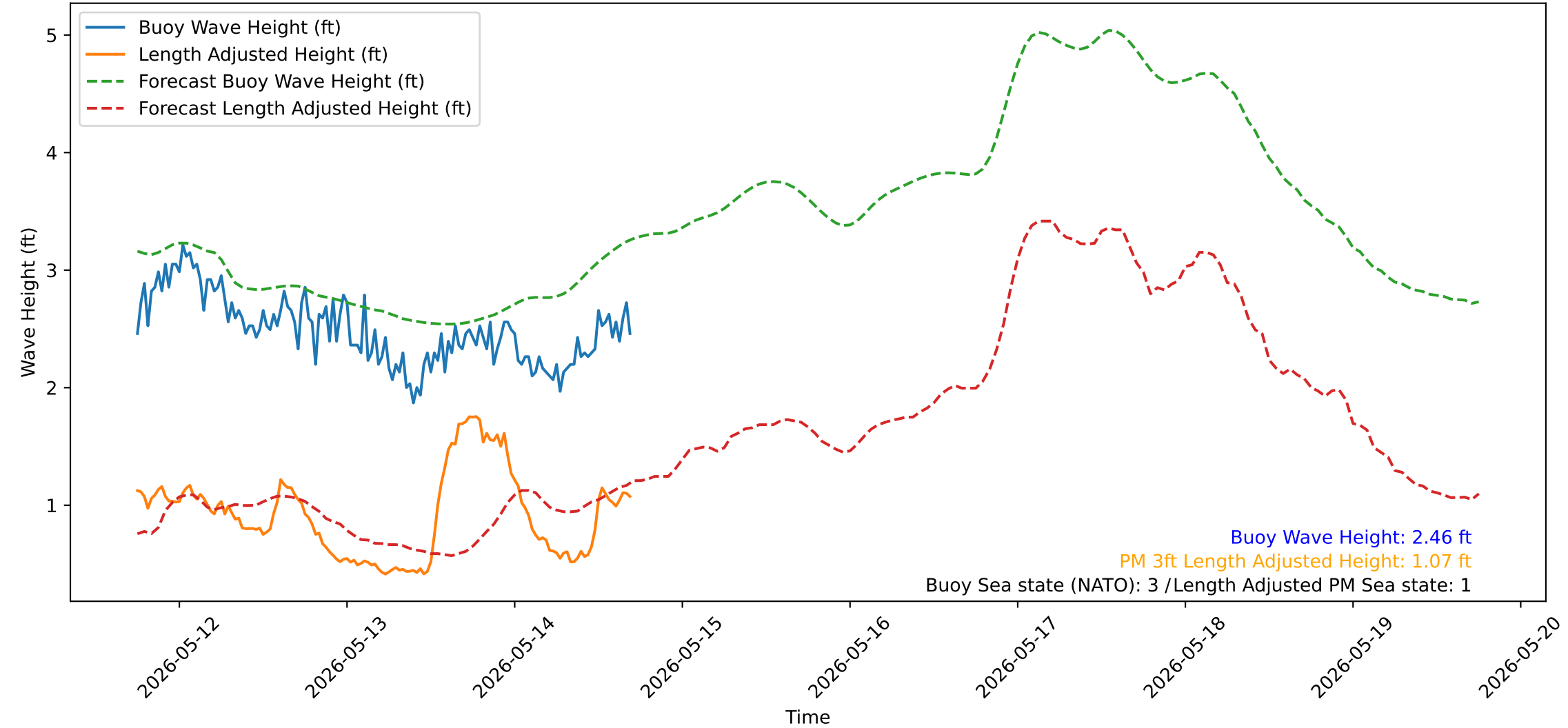
Wave Heights over Time for Red Beach at 2026-05-14 17:30:51
