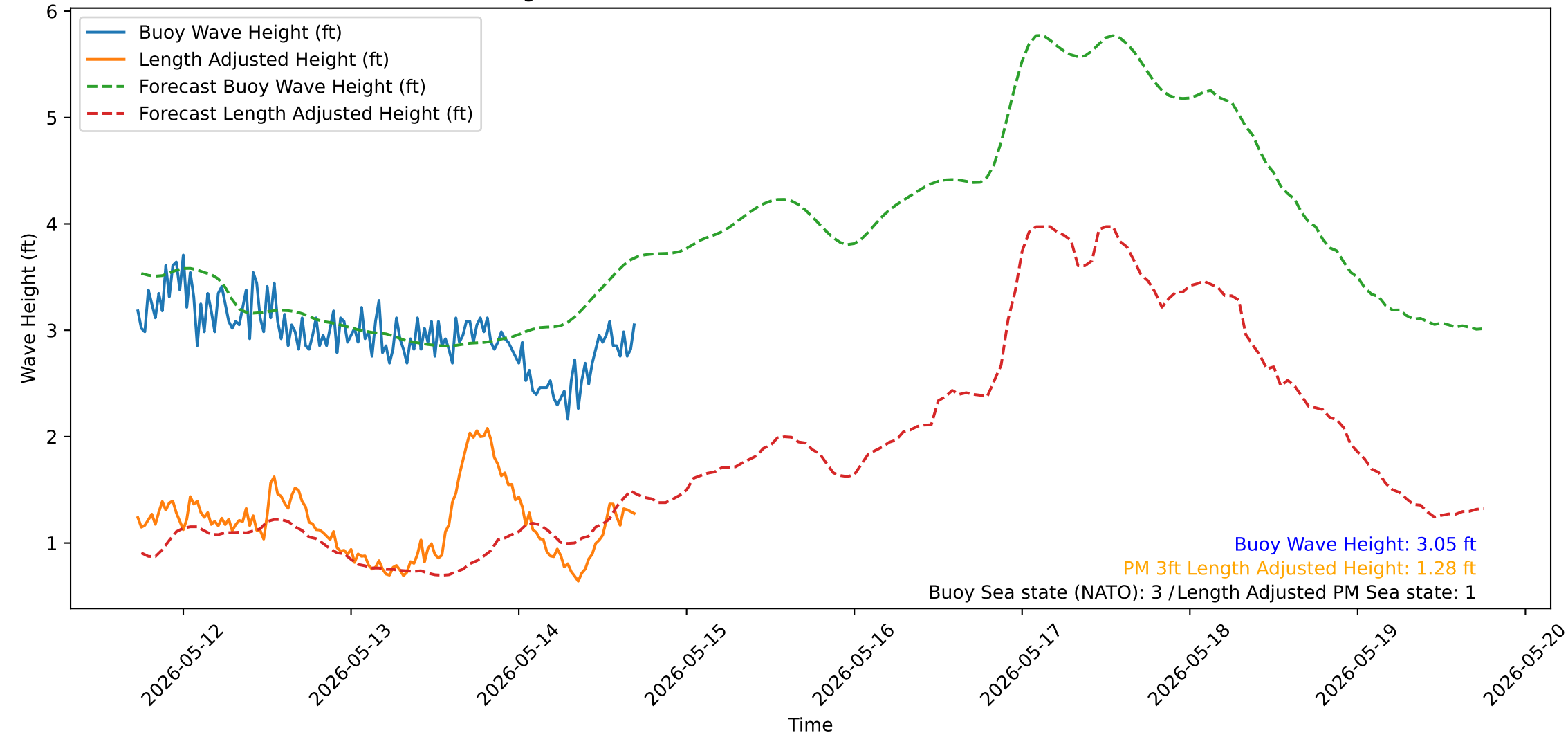
Wave Heights over Time for Oceanside Harbor at 2026-05-14 17:30:31
