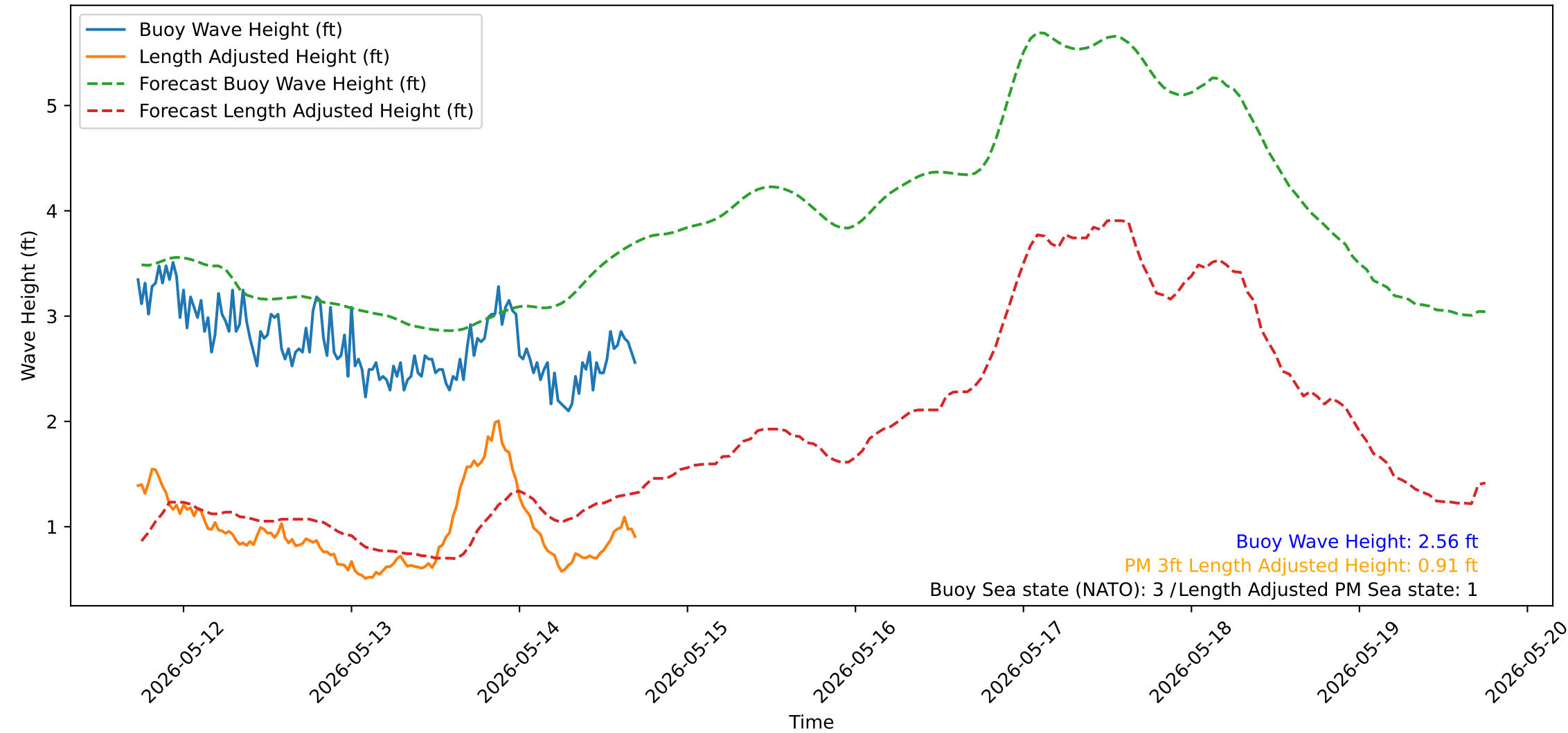
Wave Heights over Time for Green Beach at 2026-05-14 17:31:14
