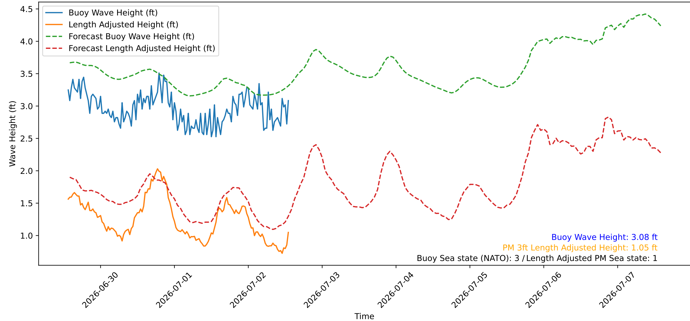
Wave Heights over Time for Green Beach at 2026-07-02 13:41:09
