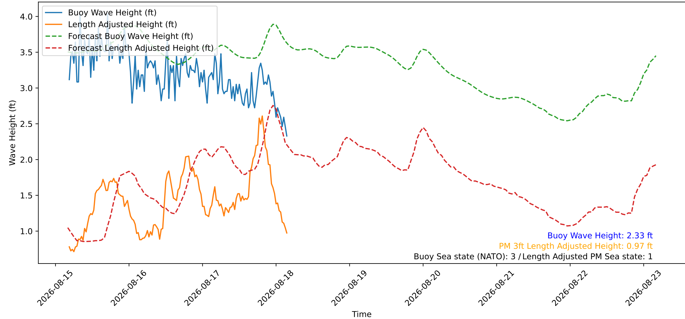
Wave Heights over Time for Red Beach at 2026-08-18 04:20:48
