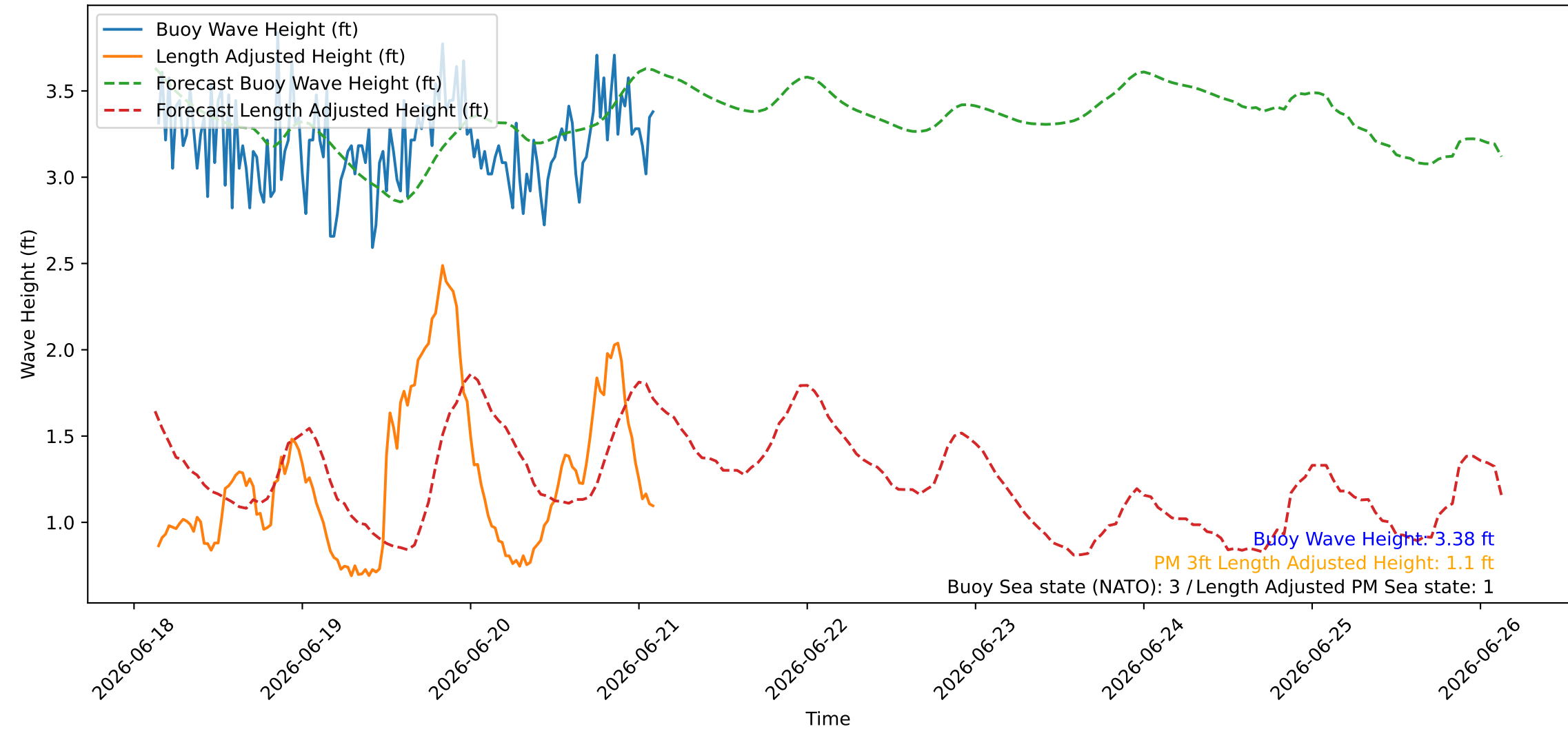
Wave Heights over Time for Red Beach at 2026-06-21 03:00:45
