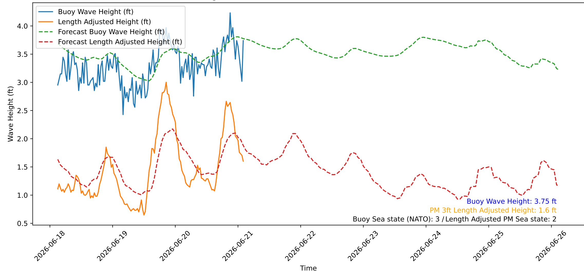
Wave Heights over Time for Green Beach at 2026-06-21 03:01:07
