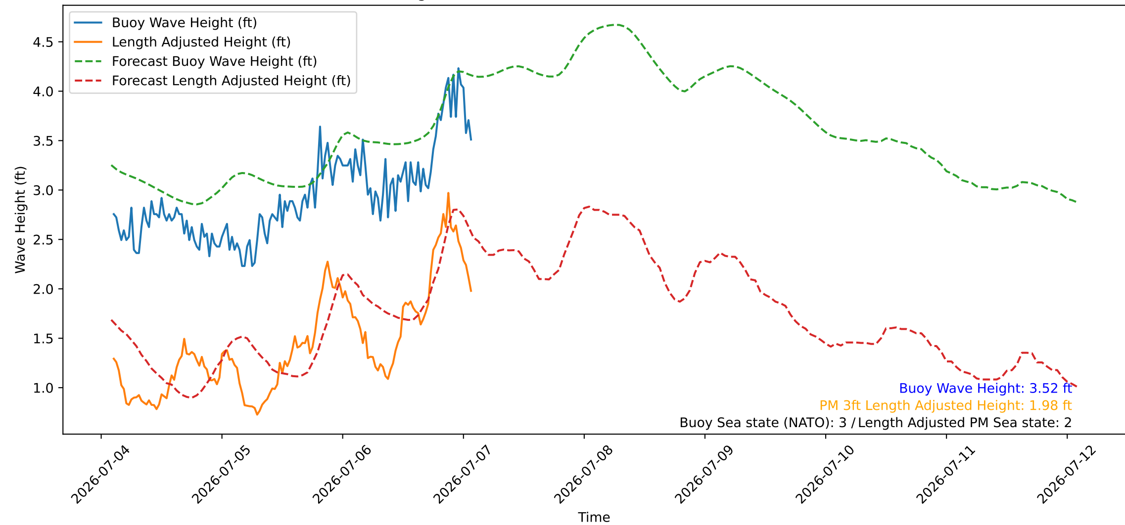
Wave Heights over Time for Red Beach at 2026-07-07 02:10:46
