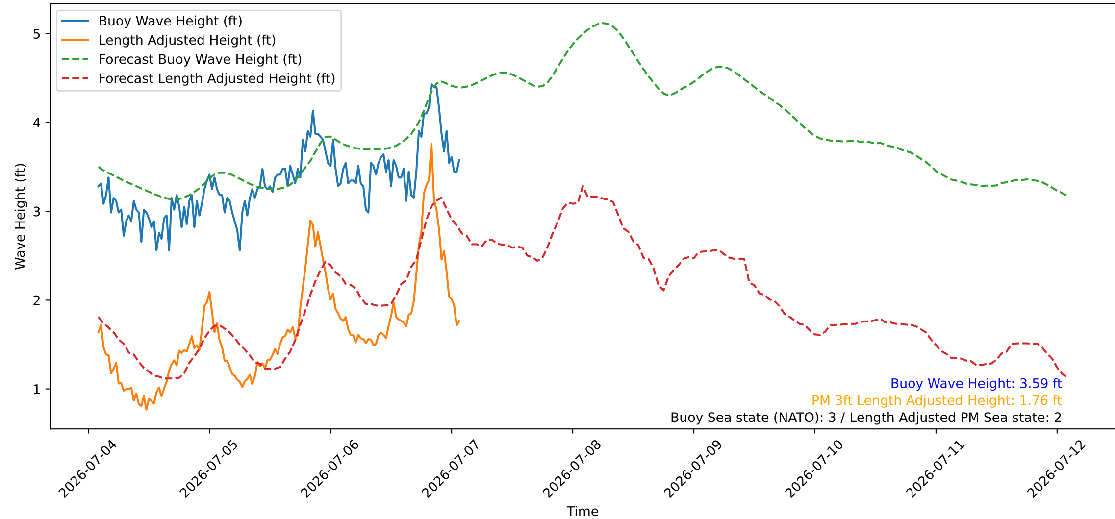
Wave Heights over Time for Green Beach at 2026-07-07 02:11:09
