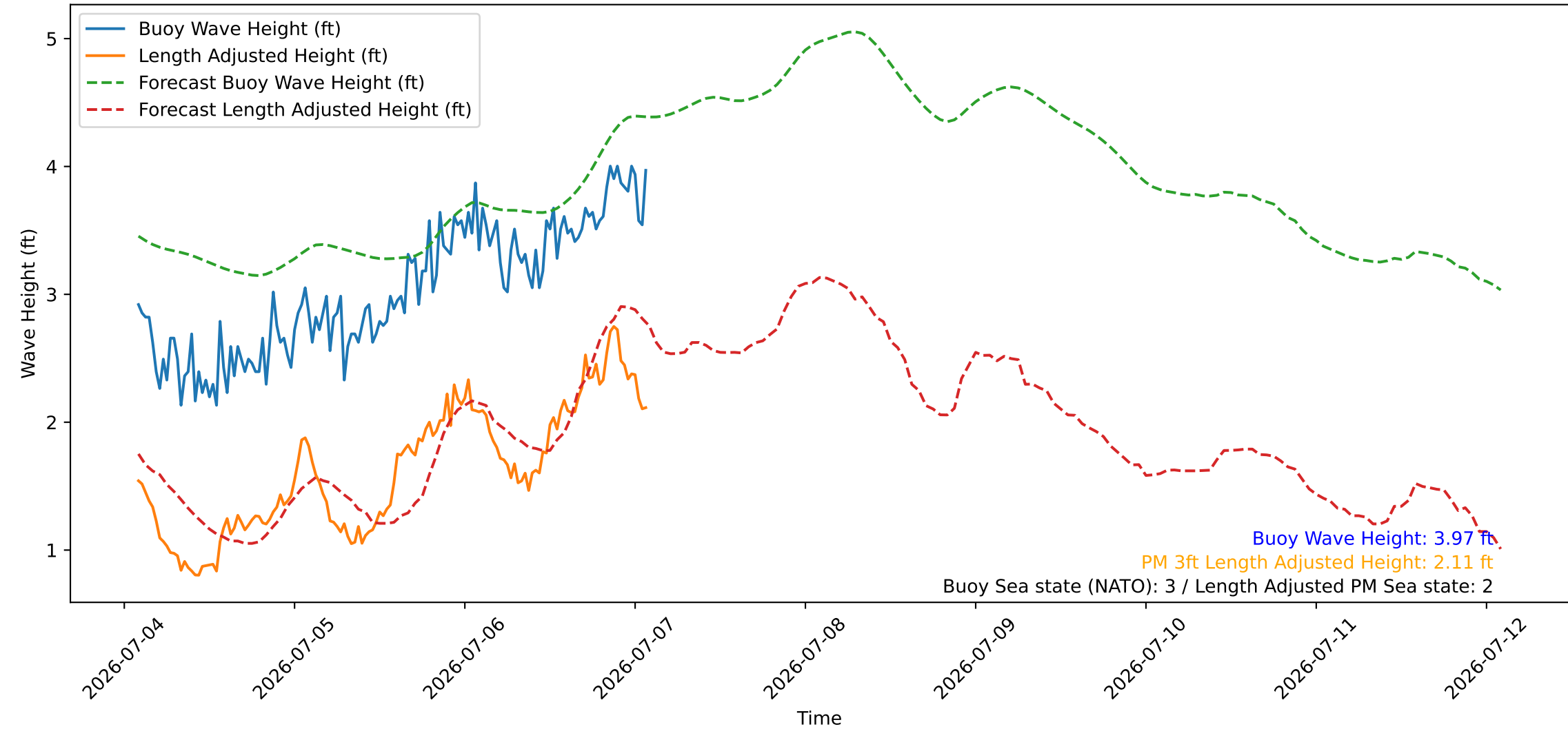
Wave Heights over Time for Oceanside Harbor at 2026-07-07 02:10:26
