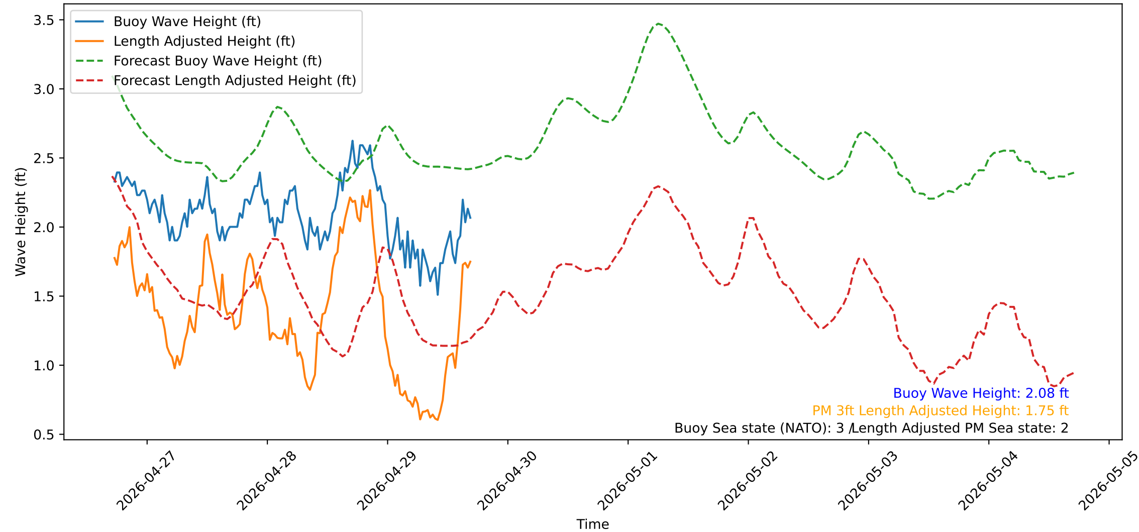
Wave Heights over Time for Red Beach at 2026-04-29 17:20:51
