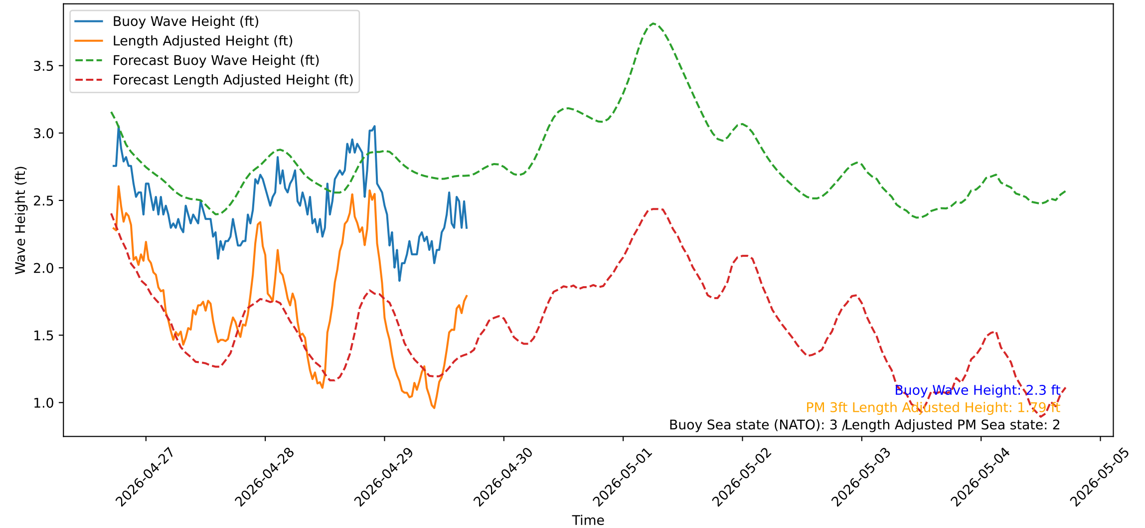
Wave Heights over Time for Oceanside Harbor at 2026-04-29 17:20:31
