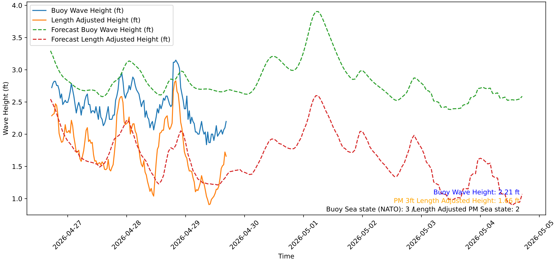
Wave Heights over Time for Green Beach at 2026-04-29 17:21:14
