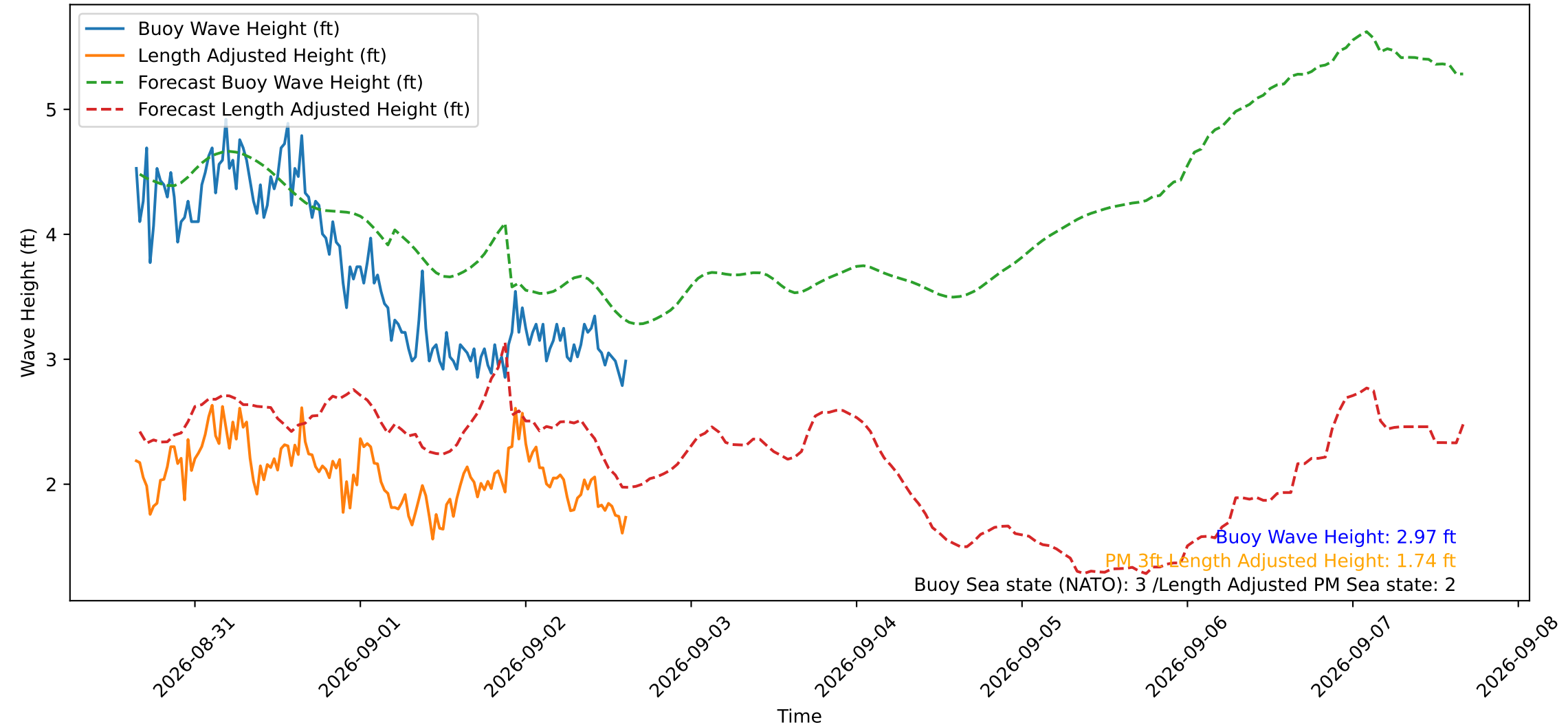
Wave Heights over Time for Oceanside Harbor at 2026-09-02 15:30:30
