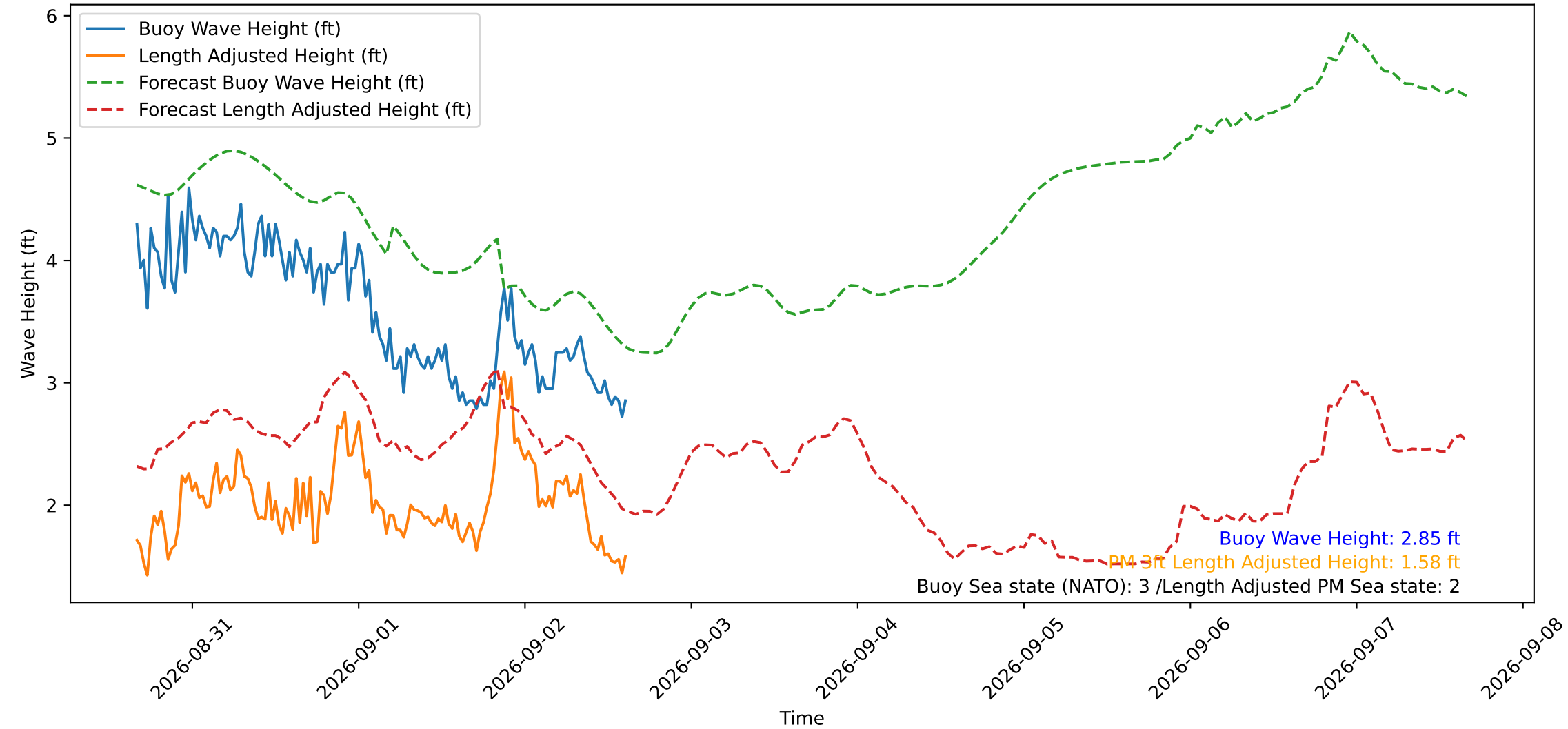
Wave Heights over Time for Green Beach at 2026-09-02 15:31:12
