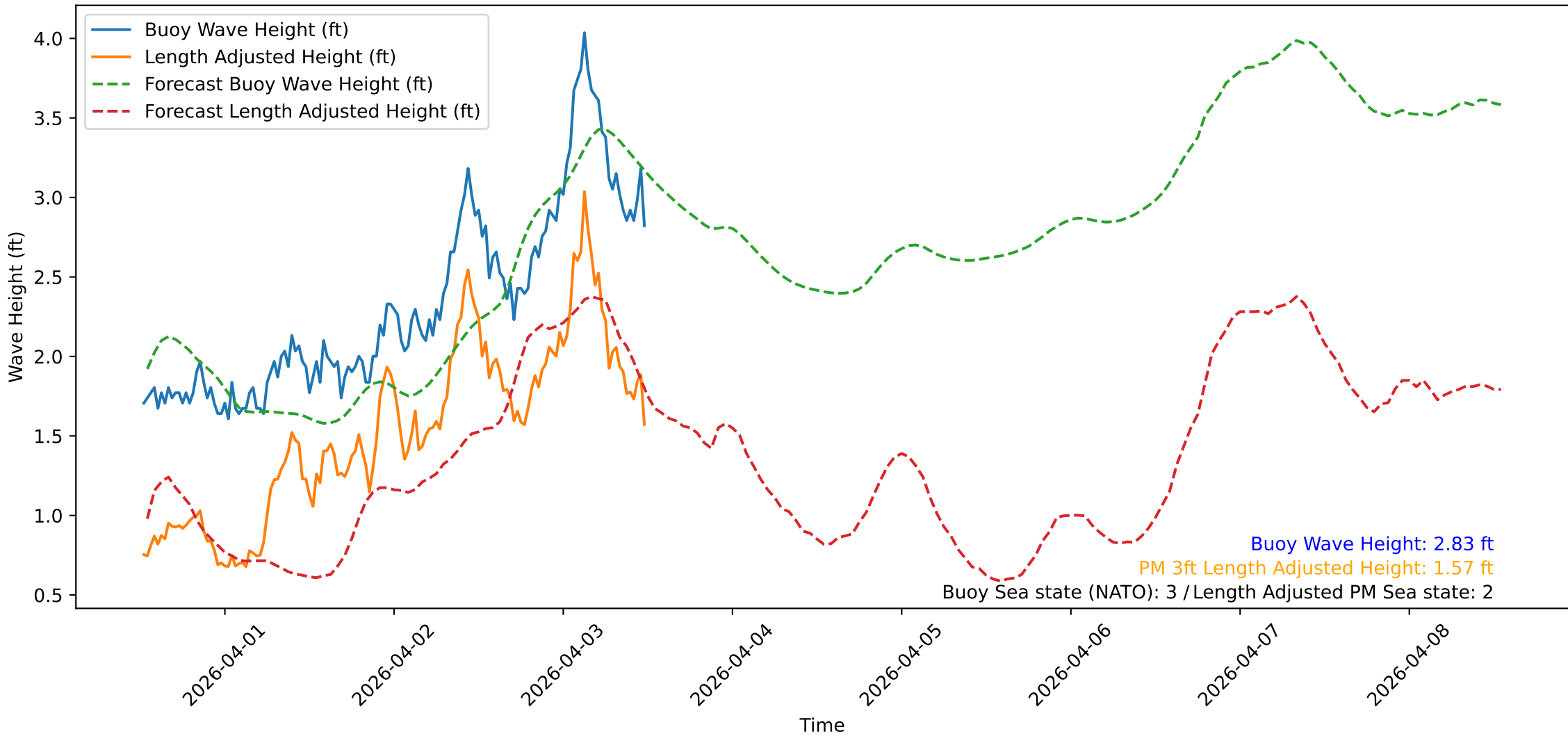
Wave Heights over Time for Oceanside Harbor at 2026-04-03 12:30:33
