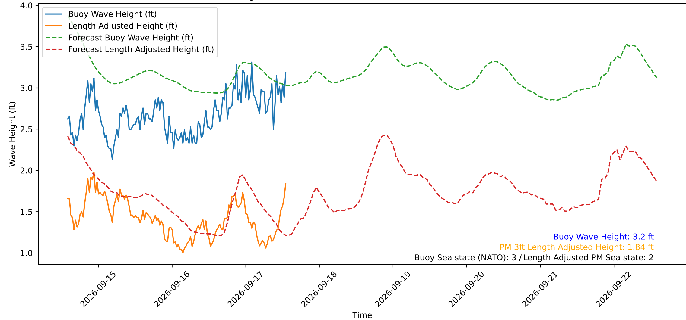
Wave Heights over Time for Green Beach at 2026-09-17 13:41:12
